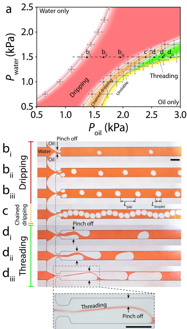
Figure 3. Characterisation of asynchronous oil droplets at various combinations of oil and water pressure: (a) Droplet generation map, showing the existence of ‘dripping’, ‘chained dripping’, ‘threading’ and ‘unstable’ modes. Average \pm standard deviation values are based on 10–50 droplets per each experiment according to the stability of droplets, with 4 experimental repeats for each device, and 3 devices being used for each experiment. (b) ‘Dripping’ mode corresponding to the asynchronous generation of droplets at the orifice. (c) ‘Chained dripping’ mode corresponding to generation of droplets that are separated by a thin layer of water. (d) ‘Threading’ mode corresponding to the advancement of oil columns through the orifice and the asynchronous generation of droplets along the sidewalls. Increase of oil pressure leads to the formation of long droplets that are separated by a thin thread of water. Scale bars are 500 \mu\text{m} .
