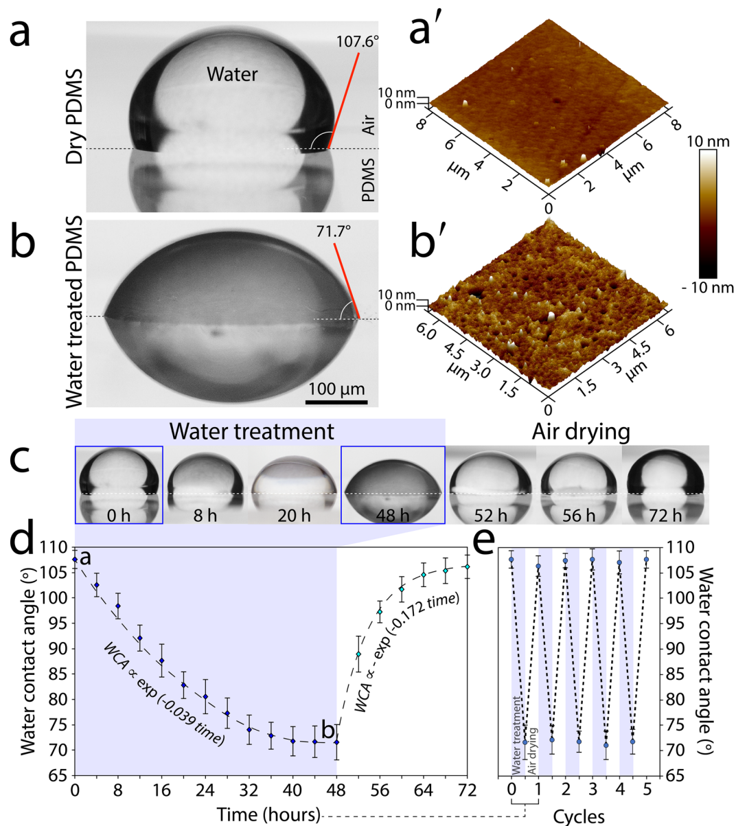
Figure 1. Altering the wettability of PDMS by water treatment: (a,b) Water contact angle of dry and water-treated (after 48 hours) PDMS surfaces. (a'-b') Surface roughness of dry and water-treated PDMS surfaces obtained by AFM analysis. (c-d) Variations in water contact angle as a function of time, showing the ability to reverse the wetting properties of PDMS in repeated cycles. (e) Reversible water contact angles over successive cycles. Average \pm standard deviation values are based on 5 experimental repeats per each PDMS block, with 3 PDMS blocks being used for each experiment.
