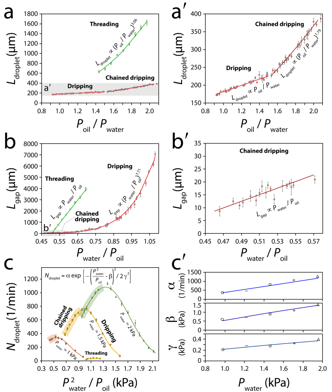
Figure 4. Characterisation of asynchronous oil droplets at various oil and water pressures: (a-a') Variation in droplet size against P_{oil}/P_{water} , (b-b') Variation in droplet gap against P_{water}/P_{oil} , (c) Variation in droplet generation rate against P_{water}^2/P_{oil} , (c') Variation in the variance ( \alpha ), mean ( \beta ) and standard deviation ( \gamma ) coefficients used in the Gaussian distribution function against P_{water} . Average \pm standard deviation values are based on 10–50 droplets per each experiment according to the stability of droplets, with 4 experimental repeats for each device, and 3 devices being used for each experiment.
