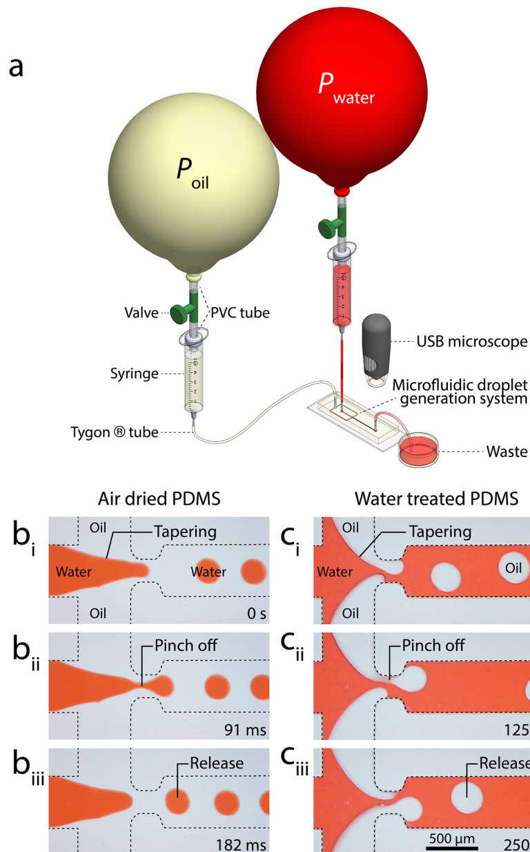
Figure 2. Comparison of droplet generation within the air-dried and water-treated microfluidic structures: (a) Experimental setup consisting of a flow focusing structure coupled with two balloon-based pressure pumps to drive red-stained water and mineral oil. (b) Generation of water droplets in oil within the air-dried channel during tapering, pinch-off, and release steps. (c) Asynchronous generation of oil droplets in water within the water-treated channel during tapering, asynchronous advancement, pinch-off, and release steps.
