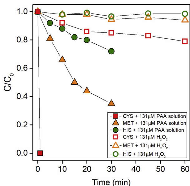
Fig. 2. Time course of transformation of CYS, MET, and HIS with PAA solution (solid dots) and H 2 O 2 solution (valid dots). Experimental conditions: [amino acids] 0 = 10 μM, [PAA] 0 = 131 μM, [H 2 O 2 ] 0 = 131 μM, pH = 7, room temperature.
