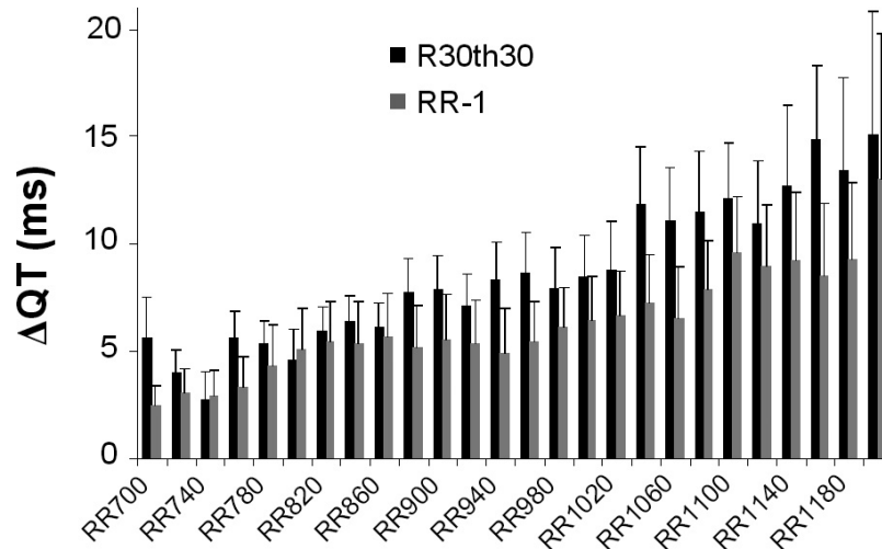
FIG. 2 QT interval changes with moxifloxacin at various heart rates. Mean + standard error of the mean.
