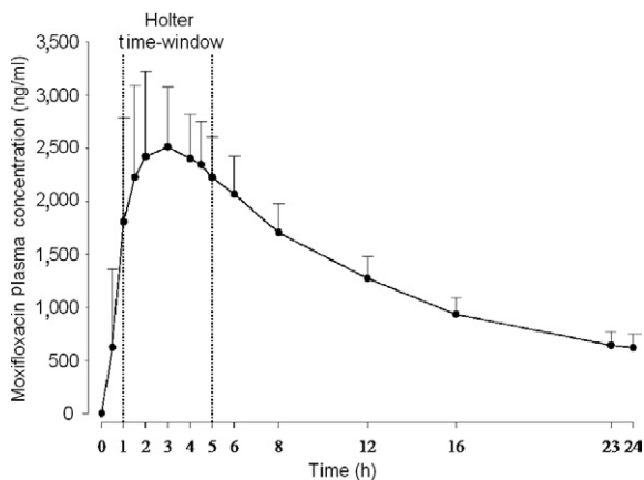
FIG. 1 Moxifloxacin plasma concentrations profiles. Moxifloxacin was administered at T0, and ECG collection was performed from h1 through h5 (T1-T5). Mean \pm standard deviation. ECG = electrocardiogram.
