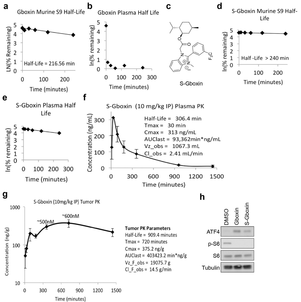
Extended Data Figure 7. S-Gboxin is pharmacokinetically stable and suitable for in vivo studies. a. Gboxin S9 half-life. n = 1. b. Gboxin plasma half-life. n = 1. c. S-Gboxin structure. d. S-Gboxin S9 half-life. n = 1. e. S-Gboxin plasma half-life. n = 1. f. S-Gboxin plasma PK data. n = 3; mean ± SD. g. S-Gboxin tumor PK data. n = 3 to 6 at each time point; mean ± SD. Plasma ( f ) and tumor ( g ) PK data indicates S-Gboxin is suitable for in vivo studies. h. Representative western blots show S-Gboxin, like its original compound Gboxin, upregulates ATF4 and suppresses p-S6 expression in HTS GBM cells. Cells were treated with DMSO, Gboxin (1 μM), or S-Gboxin (1 μM) for 12 hours. n = 2.
