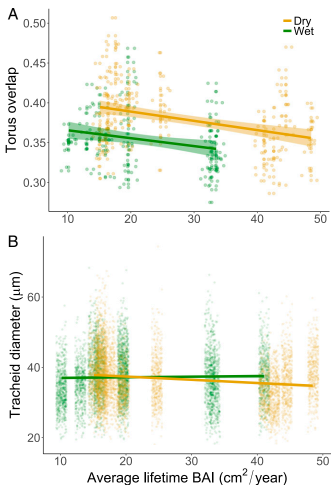
Fig. 4. Torus overlap (A) and tracheid diameters (B) by average lifetime annual BAI (cm 2 /y) for each site: Mackay Bar (Dry) and Bullion Ridge (Wet). Xylem traits were sampled at a fixed trunk diameter of 30 cm for all trees ( n = 7 trees per class, 21 total). Shaded bands represent 95% confidence intervals, but are too narrow to be visible in B due to large sample size. Points represent individual pit ( n = 322 ) and tracheid measurements ( n = 10,470 ). Torus overlap was negatively related to average lifetime growth rates among trees at both sites ( F_{1,21.59} = 7.189 , P = 0.0138 ) and was larger in trees from the drier site ( F_{1,22.19} = 11.902 , P = 0.0023 ).
