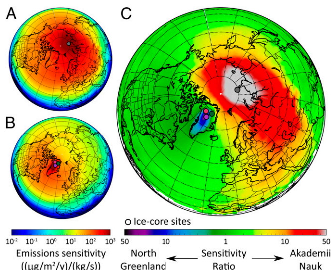
Fig. 3. FLEXPART (18, 19) simulation-based sensitivity of the (A) AN and (B) NG ice core records to lead emissions and (C) their ratio. The \sim 8 -fold higher lead deposition observed in the AN record compared with the NG composite (Fig. 1) is consistent with the 2- to 12-times higher sensitivity to European emissions in the AN/NG ratio, indicating that lead pollution in the Arctic array was dominated by European emissions before the Industrial Revolution.
