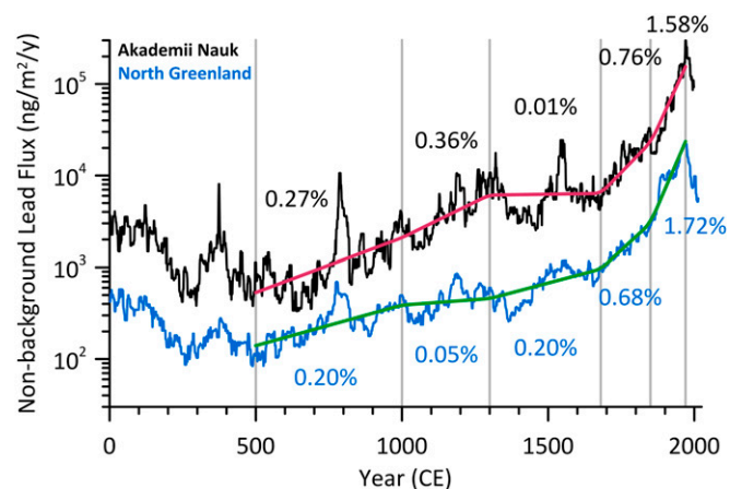
Fig. 2. Arctic lead pollution (11-y median filter) with fitted average growth rates ( Materials and Methods ) during specific historical periods in the NG (green) and AN (red) records ( SI Appendix , Table S2).
