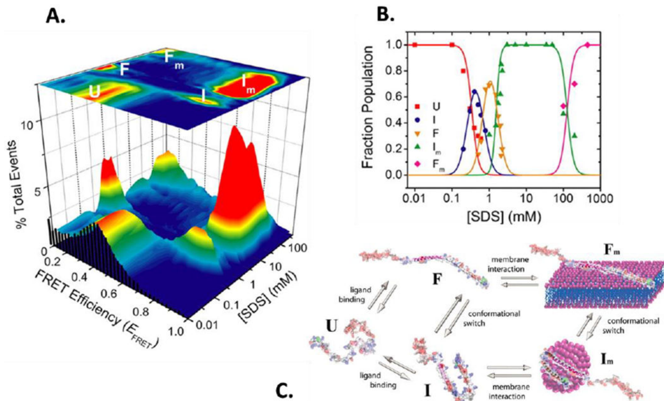
Figure 2. Single-molecule fluorescence data for \alpha -synuclein. A. 3D smFRET histograms as a function of concentration of the lipid mimic showing a complex folding-binding landscape. B. Populations of different species derived from histograms in A, showing multiple transitions between different species. C. Cartoons of the different states revealed in A. Adapted from Ferreon et al. Proc. Natl. Acad. Sci. (2009) 14:5645. See text for additional details.
