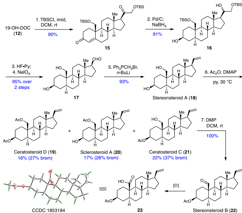
Fig. 4 Unified synthesis of the sterosteroid family. Five sterosteroid family members including sclerosteroid A, sterosteroid A and B, ceratosteroid C and D were synthesized from the common intermediate 19-OH-DOC in 5 to 7 steps
