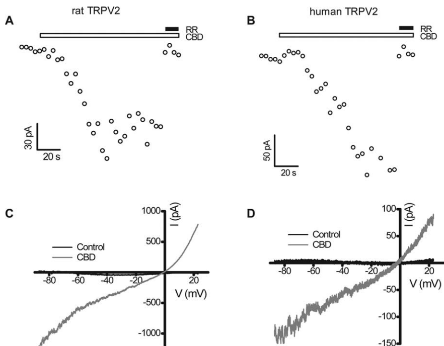
Figure 3. Activation of TRPV2 by CBD in whole-cell patch clamp. A, B , Time course of activation by 30 \mu\text{M} CBD at -87 mV for rat ( A ) and human ( B ) TRPV2. C, D , Current–voltage ( I – V ) relationships of rat ( C ) and human ( D ) TRPV2 in response to 30 \mu\text{M} CBD. The currents were elicited with a continuous voltage ramp from -87 mV to +23 mV once every 4 s. The I – V plots are averages of five current traces and are subtracted from responses in the concurrent presence of CBD (30 \mu\text{M} ) and RR (10 \mu\text{M} ).
