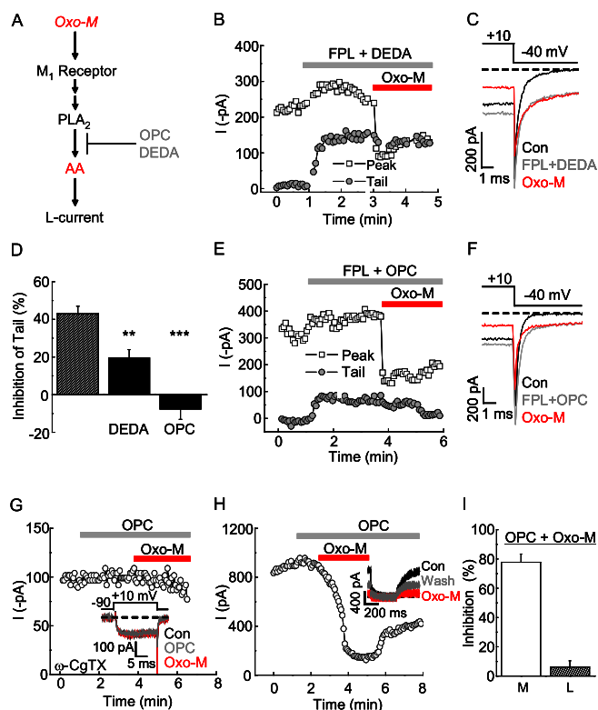
Figure 3. PLA 2 antagonists minimize L-current but not M-current inhibition by Oxo-M. A , Schematic illustrating experimental protocol to test effects of selective PLA 2 antagonists, DEDA (IC 50 of \sim 20 \mu M) and OPC (IC 50 of 6 \mu M), on L-current modulation. B–F , When FPL was included in the bath to enhance L-current, Oxo-M-induced inhibition of the long-lasting tail current was lost in the presence of either 100 \mu M DEDA ( B , C ) or 10 \mu M OPC ( E , F ). D , Summary of the average percentage inhibition of the long-lasting tail current after Oxo-M treatment (hatched bar) or Oxo-M plus various PLA 2 inhibitors (filled bars): DEDA (100 \mu M; 20 \pm 4\% ); OPC (10 \mu M; -8 \pm 6\% ). **p < 0.01 , ***p < 0.001 compared with no inhibitor, using a two-way t test for two means; n = 4–8 recordings per group. G , When cells were preincubated in \omega -CgTX to block N-channel activity, Oxo-M-induced inhibition of L-current was minimized in the presence of OPC. Inset, Selected sweeps from the experiment; fast tail currents have been truncated. H , Oxo-M inhibited M-current over time and in individual sweeps (inset) in the presence of OPC. I , Summary of Oxo-M-induced inhibition of peak L-current ( n = 10 ) in \omega -CgTX-treated cells and of M-current ( n = 5 ) in the presence of 10 \mu M OPC. Con, Control.
