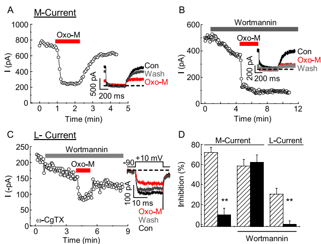
Figure 2. Wortmannin blocks recovery of M-current but not L-current. A , Bath application of Oxo-M reversibly inhibits M-current in adult SCG neurons. Inset, Selected traces from the recording. B , Wortmannin (10 \mu M) blocked M-current recovery from inhibition. Inset, Selected traces from the recording. C , In contrast, L-current inhibition in neonatal SCG neurons reversed in the presence of wortmannin. Inset shows selected traces from the recording. The fast tail currents have been truncated. D , Summary of L- and M-current inhibition by Oxo-M and their recovery in the presence of wortmannin. Under control conditions, Oxo-M inhibited M-current 72 \pm 5\% ( n = 6 ). Inhibition (hatched bars) was readily reversible, with only 9.6 \pm 6.5\% inhibition remaining after \sim 1 min of washout (filled bars). In contrast, although the presence of wortmannin did not significantly change M-current inhibition by Oxo-M ( 58 \pm 7\% ; n = 4 ), M-current remained inhibited by 62 \pm 7.6\% after 3 min of wash. Oxo-M-induced L-current inhibition in the presence of wortmannin was normal ( 30 \pm 6\% ; n = 6 ) in \omega -CgTX-treated cells ( p > 0.17 when comparing percentage current inhibition of untreated to wortmannin-treated cells using a two-tailed t test for two means). Inhibition readily reversed, with 0.1 \pm 3.6\% remaining after \sim 1 min of washout. **p < 0.01 compared with inhibition by Oxo-M using a two-tailed paired t test. Con, Control.
