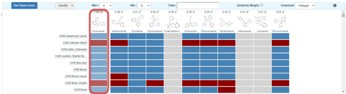
Figure 9. GenRA predictions
