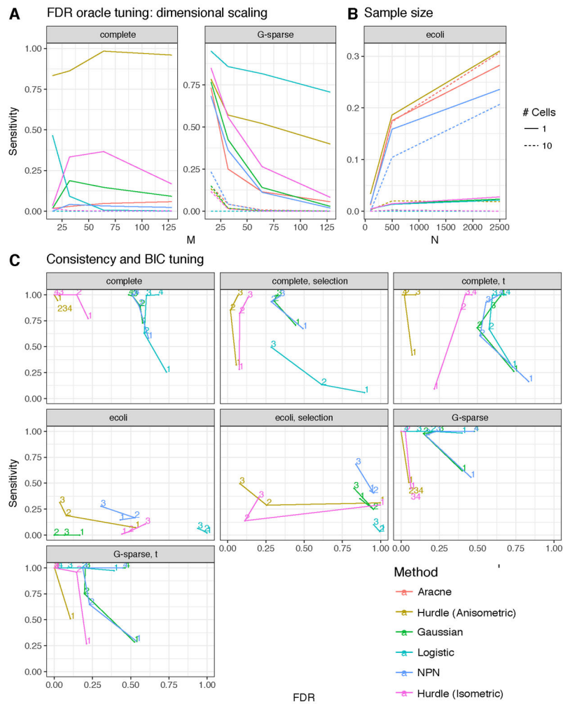
Fig 4: Dimensional (a) and sample size scaling (b) of six different network inference algorithms applied to simulated data under oracle FDR tuning. Data are generated from the multivariate hurdle model (6) under chain graphs (a) and e. coli graph (b). Panel (c) shows network selection consistency of various methods using the Bayesian Information Criterion under various models described in the supplement. The paths trace out the changes in FDR and sensitivity as the sample size increases geometrically from 100 (1) to 12,500(4).
