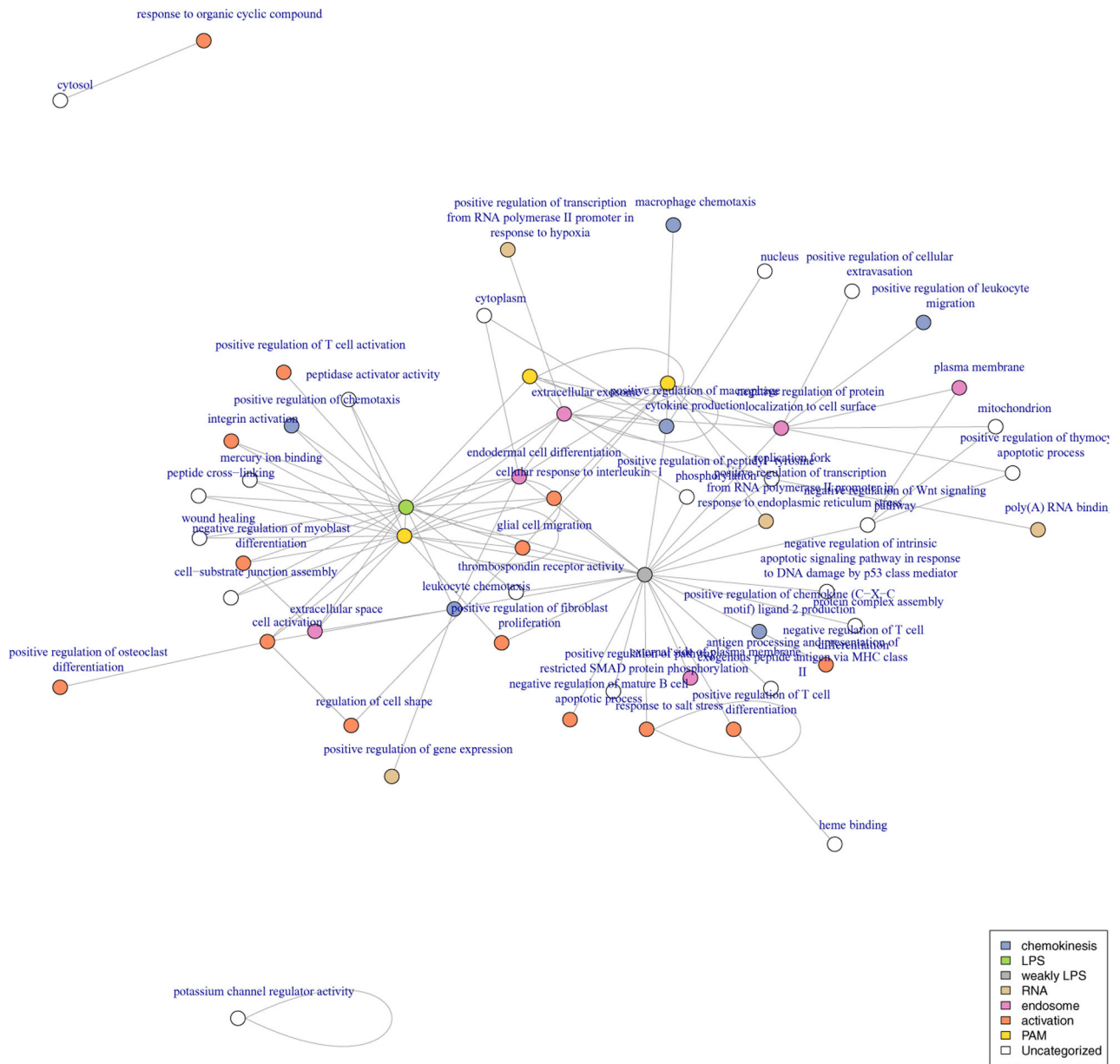
Fig 10: Modules enriched at FDR 10% using graphical geneset edge enrichment in mouse dendritic cells under Gaussian model.
