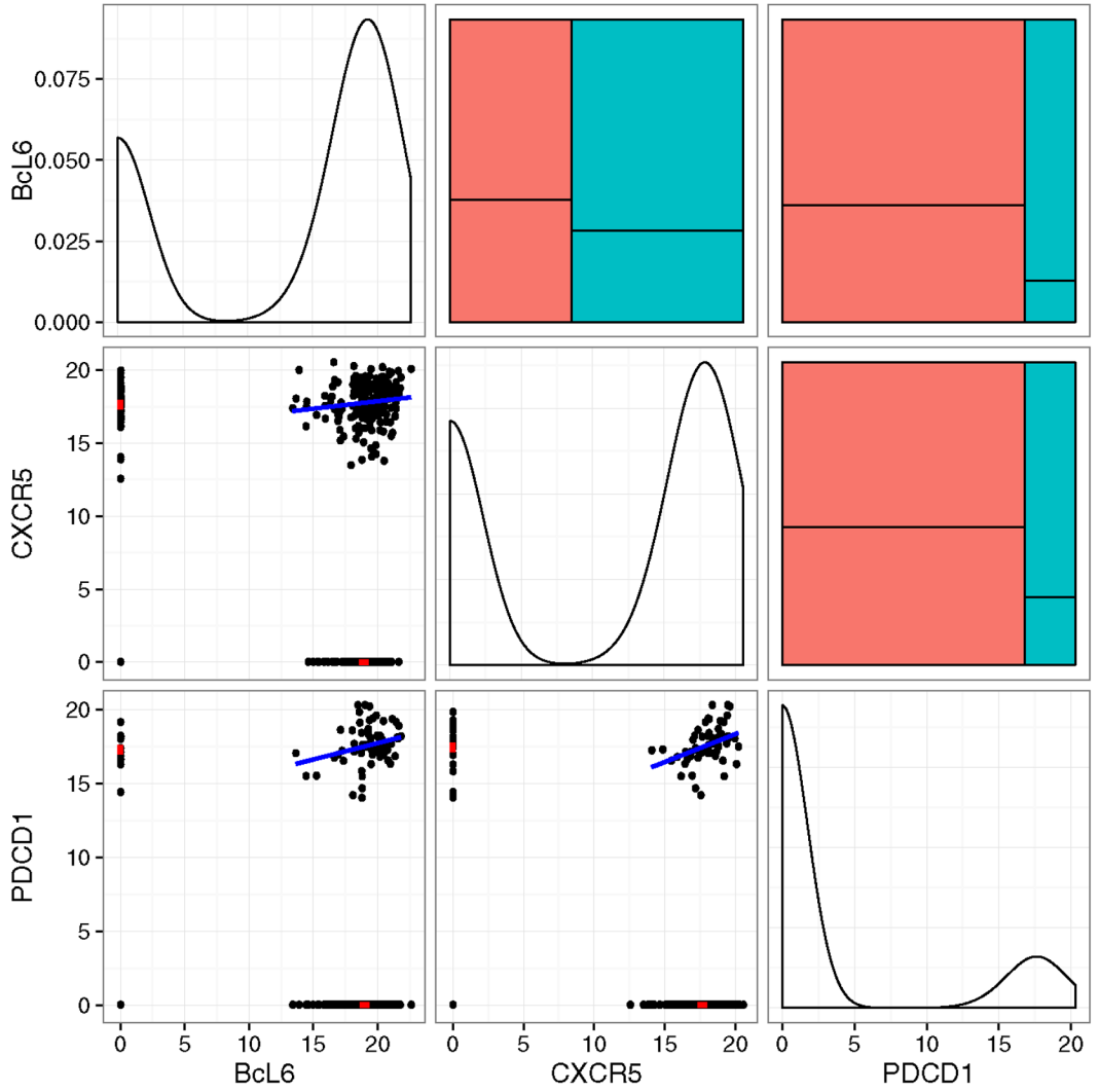
Fig 2: Scatter plots of inverse cycle threshold ( 40 - Ct ) measurements y from a quantitative PCR (qPCR)-based single cell gene expression experiment (lower panels). The cycle threshold ( Ct ) is the PCR cycle at which a predefined fluorescence threshold is crossed, so a larger inverse cycle threshold corresponds to greater log-expression [McDavid et al., 2013]. Measurements that failed to cross the threshold after 40 cycles are coded as 0. The upper panels show mosaic plots of each pair of contingency tables that can be formed from the indicator functions [v_y]_i = I_{y_i > 0} . On the lower panels, the linear regression on positive pairs of observations is indicated in blue, while the conditional mean values are indicated in red.
