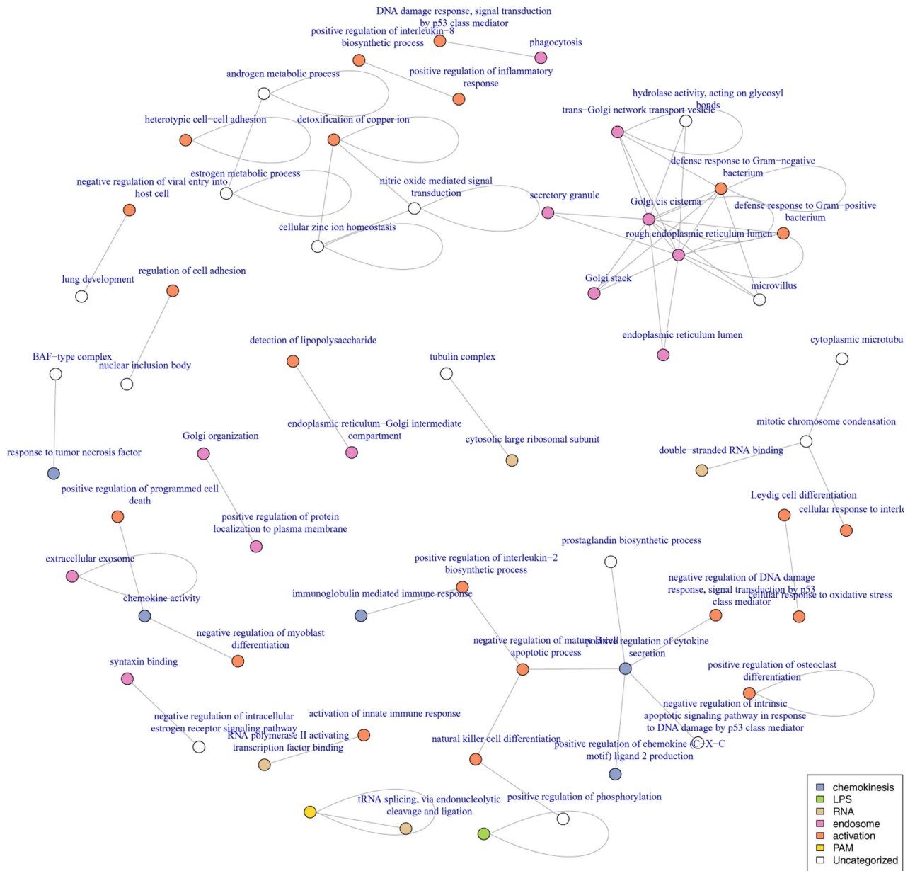
Fig 11: Modules enriched at FDR 10% using graphical geneset edge enrichment in mouse dendritic cells under Hurdle model.
