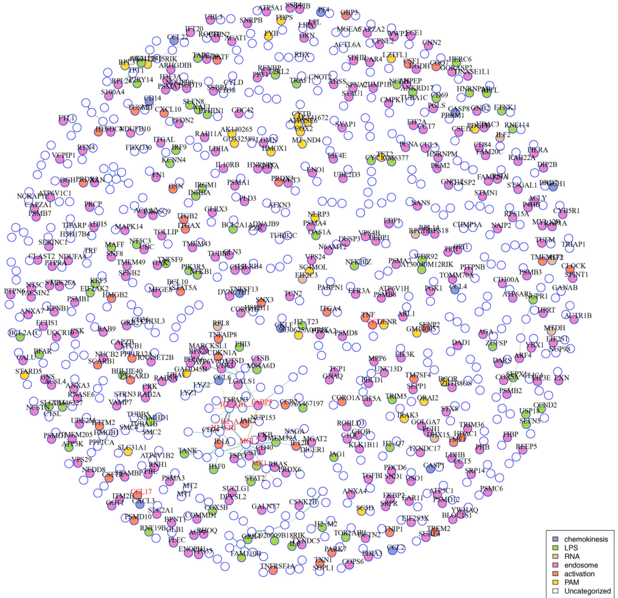
Fig 8: Core Hurdle model networks estimated in LPS-treated mouse dendritic cells. Hub genes are shown in red. Vertex colors indicate gene ontology membership. Disconnected subgraphs with two vertices are suppressed.
