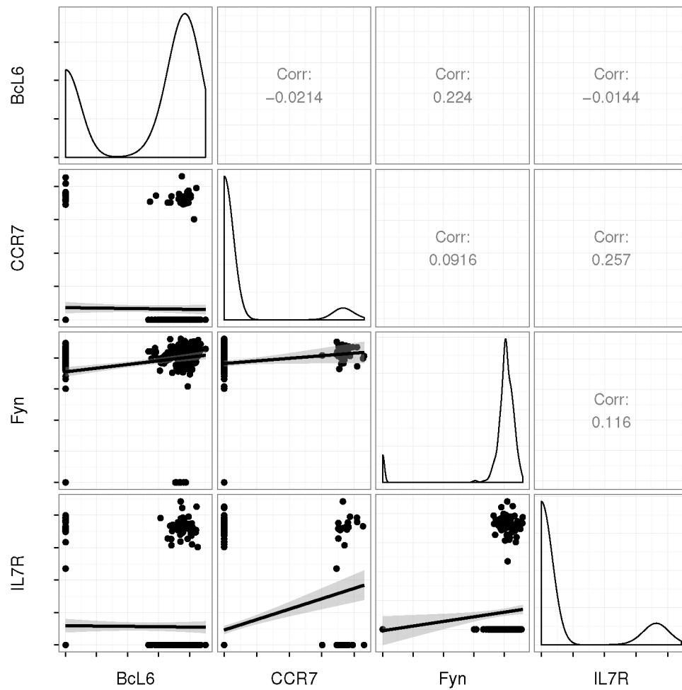
Fig 1: Scatter plots of inverse cycle threshold (40-Ct) measurements from a quantitative PCR (qPCR)-based single cell gene expression experiment (lower panels). The cycle threshold (Ct) is the PCR cycle at which a predefined fluorescence threshold is crossed, so a larger inverse cycle threshold corresponds to greater log-expression [McDavid et al., 2013]. Measurements that failed to cross the threshold after 40 cycles are coded as 0. Marginal expression in Tfh (CXCR5 + PD1 + ) cells of Tfh marker genes is illustrated in the kernel-density estimates along the diagonal. The lower panels show the linear relationships between pairs of genes.
