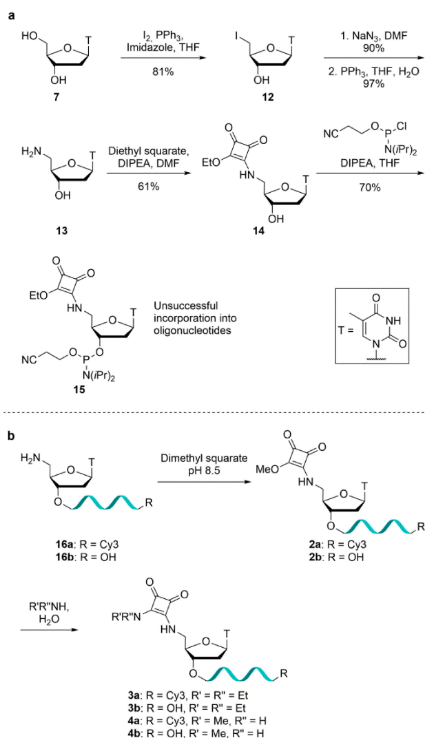
Scheme 2. Synthesis of 5'-modified oligonucleotides. a) Synthesis of 5'-squaramide modified phosphoramidite 15 . b) Synthesis of squaramide-modified oligonucleotides 2a-b , 3a-b and 4a-b after solid-phase synthesis.
