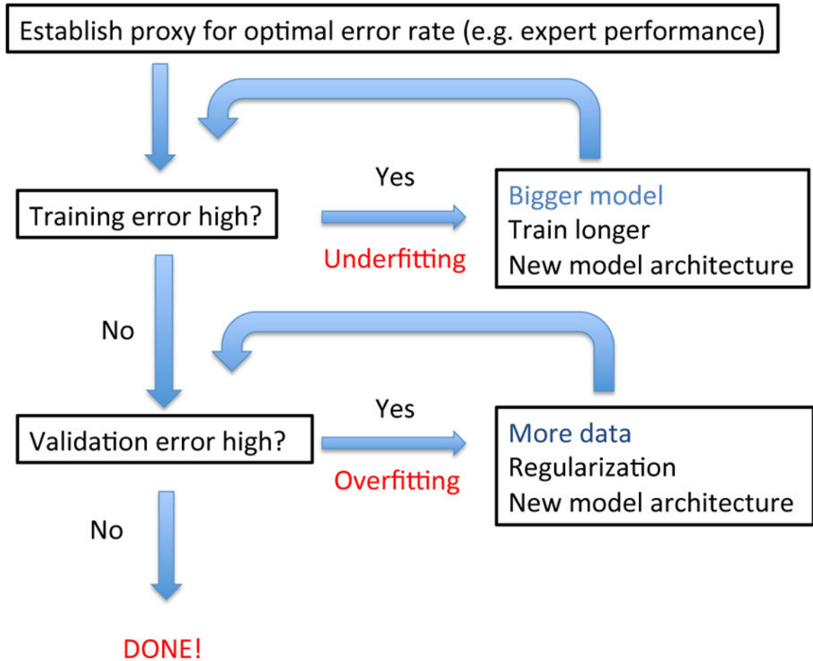
FIG. 46. Organizing a workflow for Deep Learning.
