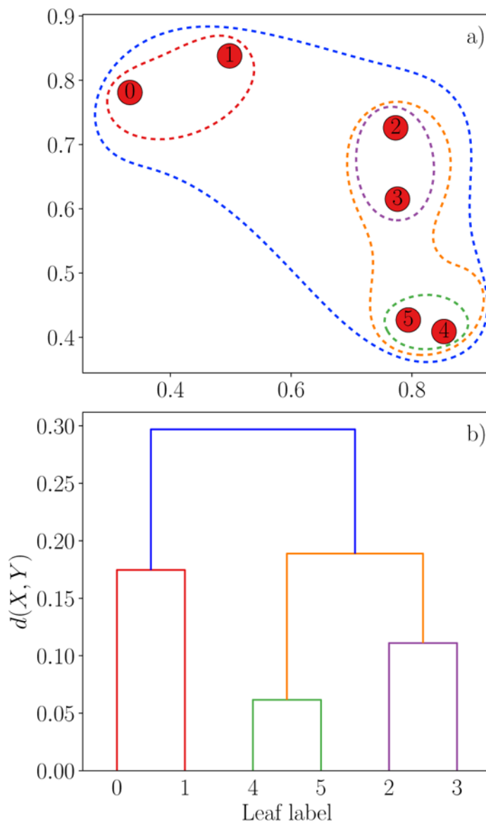
FIG. 56. Hierarchical clustering example with single linkage. (a) The data points are successively grouped as denoted by the colored dotted lines. (b) Dendrogram representation of the hierarchical decomposition. Each node of the tree represents a cluster. One has to specify a scale cut-off for the distance measure d(X, Y) (corresponding to a horizontal cut in the dendrogram) in order to obtain a set of clusters.
