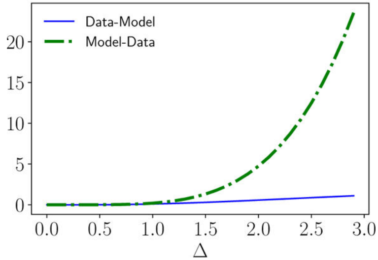
FIG. 69. KL-divergences between the data distribution p_{\text{data}} and the model p_{\theta} . Data is drawn from a bimodal Gaussian distribution with unit variances peaked at \pm 2.5 with \Delta = 2.0 and the model p_{\theta}(x) is a Gaussian with mean zero and same variance as p_{\text{data}}(x) . (Top) p_{\text{data}} and p_{\theta} for \Delta = 2.0 . (Bottom) D_{KL}(p_{\text{data}}||p_{\theta}) (Data-Model) and D_{KL}(p_{\theta}||p_{\text{data}}) (Model-Data) as a function of \Delta . Notice that D_{KL}(p_{\text{data}}||p_{\theta}) is insensitive to placing weight in the model distribution in regions where p_{\text{data}} \approx 0 whereas D_{KL}(p_{\theta}||p_{\text{data}}) punishes this harshly.
