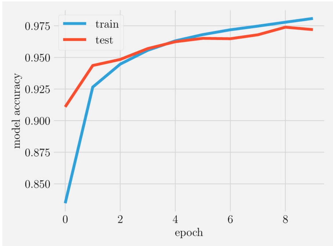
FIG. 37. Model accuracy of the DNN defined in the main text to study the MNIST problem as a function of the training epochs.
