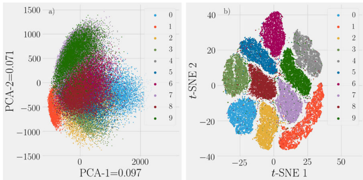
FIG. 54. Visualization of the MNIST handwritten digits training dataset (here N=60000 ). (a) First two principal components. (b) t-SNE applied with a perplexity of 30, a Barnes-Hut angle of 0.5 and 1000 gradient descent iterations. In order to reduce the noise and speed-up computation, PCA was first applied to the dataset to project it down to 40 dimensions. We used an open-source implementation to produce the results (Linderman et al. , 2017), see https://github.com/KlugerLab/FIt-SNE .
