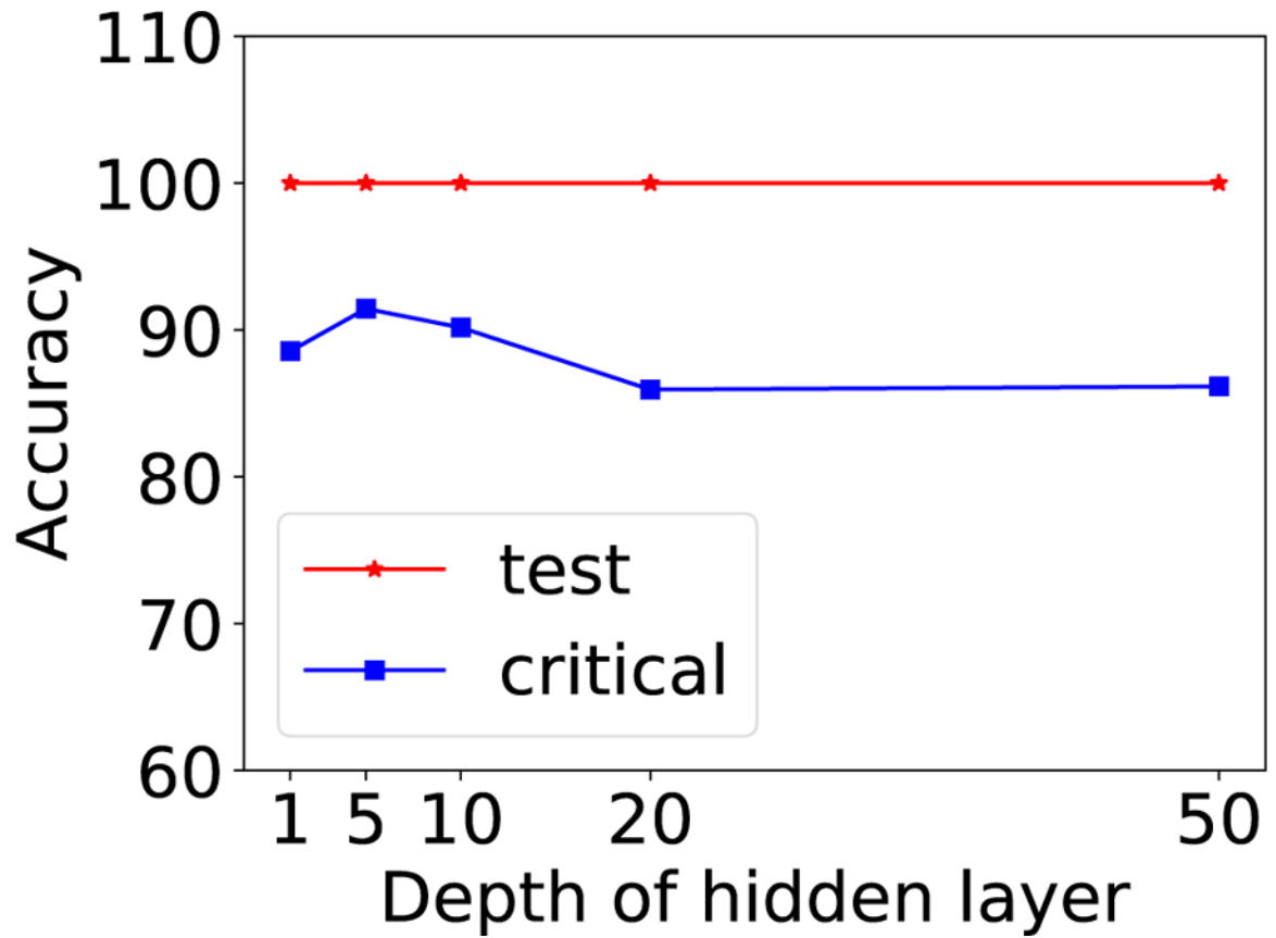
FIG. 45. Single-layer convolutional network for classifying phases in the Ising mode.
