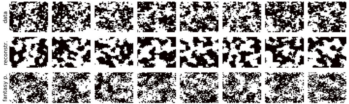
FIG. 68. MC samples, their reconstructions and fantasy particles generated by a Deep Boltzmann Machine in the disordered phase of the the 2D Ising data set at T/J = 2.75 . We used two hidden layers of 1000 and 100 layers, respectively.
