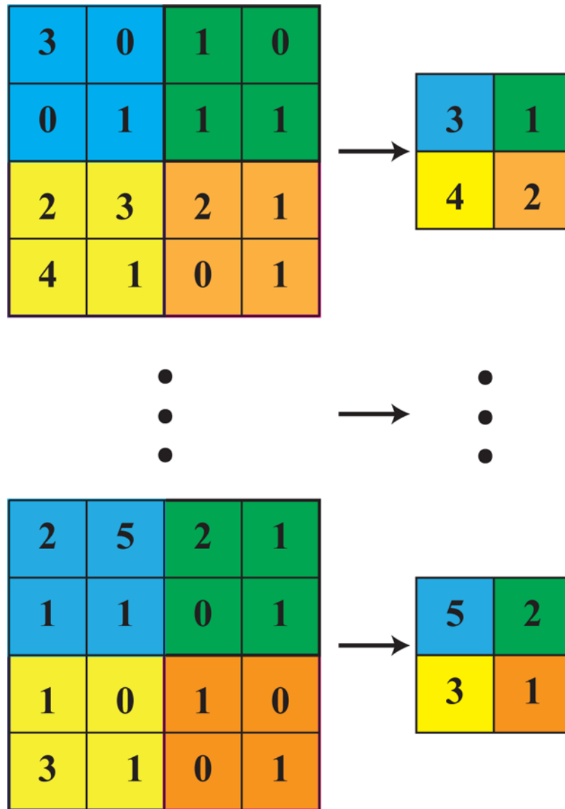
FIG. 44. Illustration of Max Pooling.
