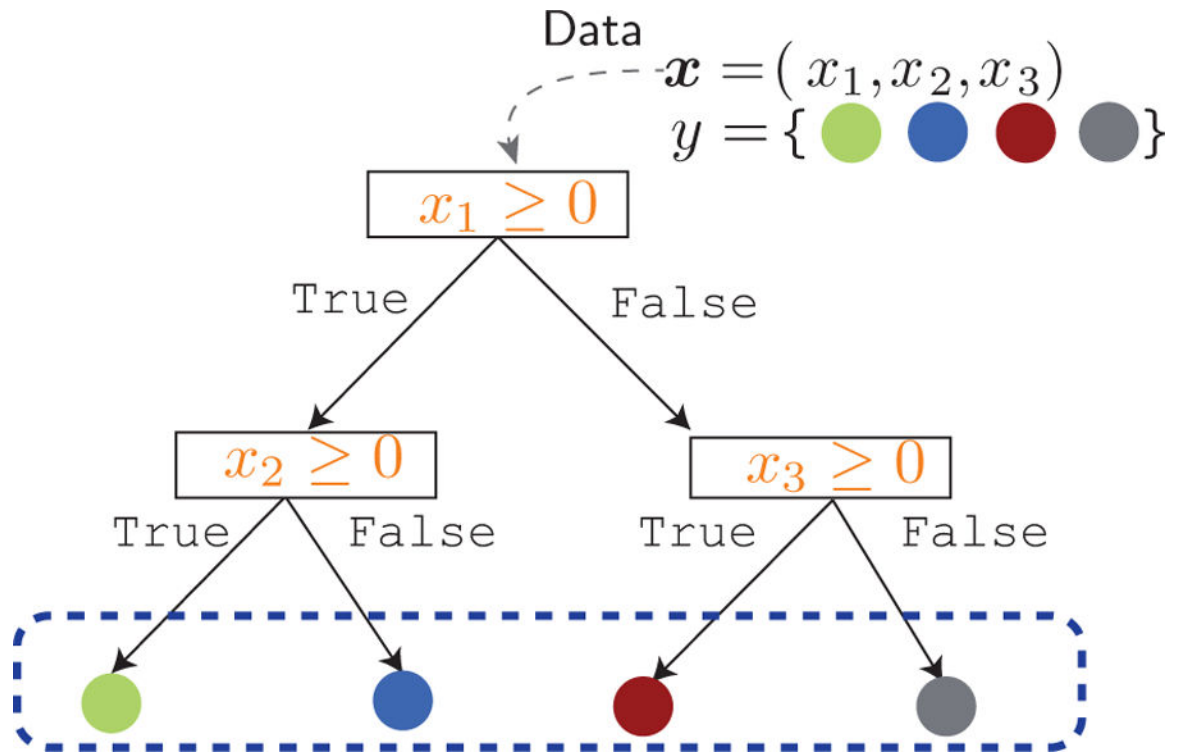
Example of a decision tree. For an input observation \mathbf{x} , its label y is predicted by traversing it from the root all the way down the leaves, following branches it satisfies.
