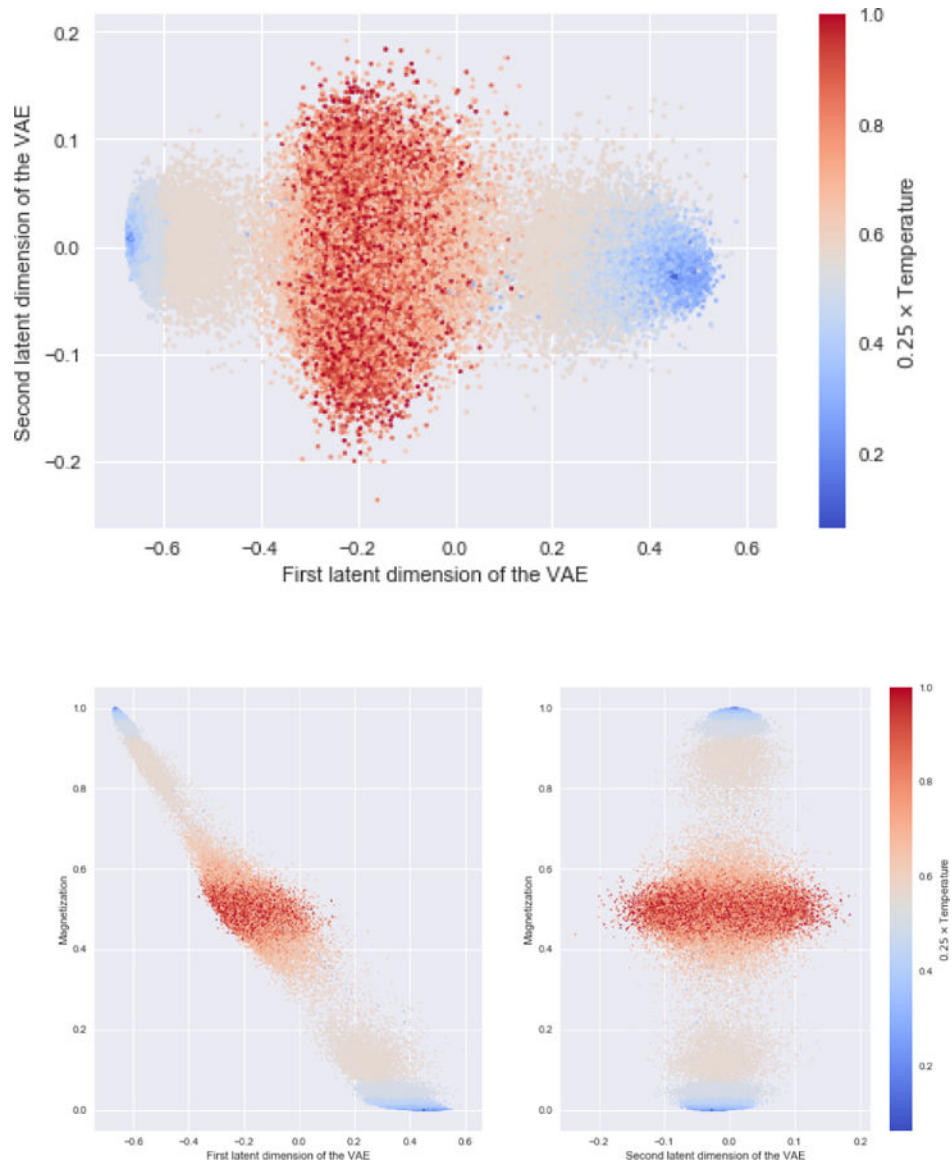
FIG. 77. (Top) Embedding of the Ising dataset into a two-dimensional latent space using a VAE with two latent dimensions (see Notebook 20 and main text for details.) Data points are colored by temperature sample was drawn at. (Bottom) Correlation between the latent dimensions and the magnetization for each sample. Notice the first principle component corresponds to the magnetization.
