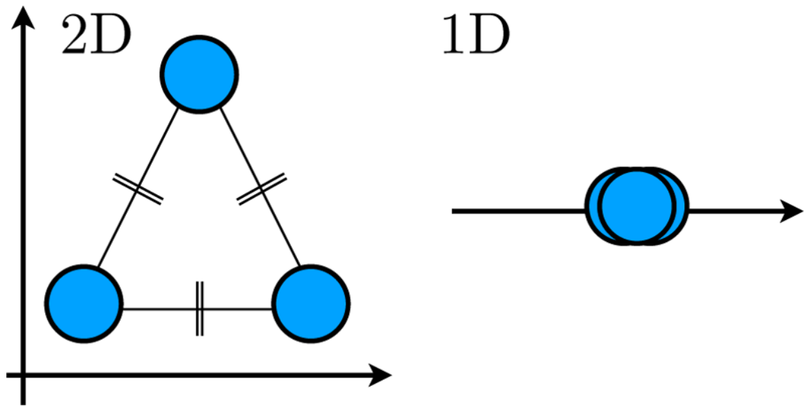
FIG. 49. Illustration of the crowding problem. (Left) A two-dimensional dataset X consisting of 3 equidistant points. (Right) Mapping X to a one-dimensional space while trying to preserve relative distances leads to a collapse of the mapped data points.
