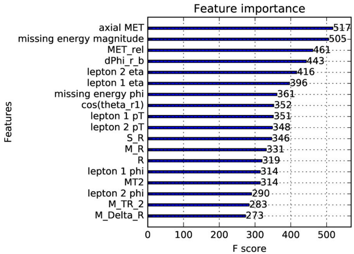
FIG. 33. Feature Importance Scores in SUSY dataset from applying XGBoost to 100, 000 samples. See Notebook 10 for more details.
