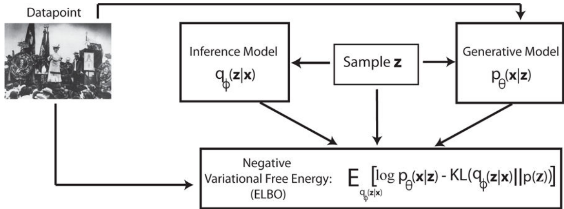
FIG. 73. Schematic explaining the computational flow of VAEs. Figure based on Kingma's Ph.D. dissertation Chapter 2. (Kingma et al. , 2017).
