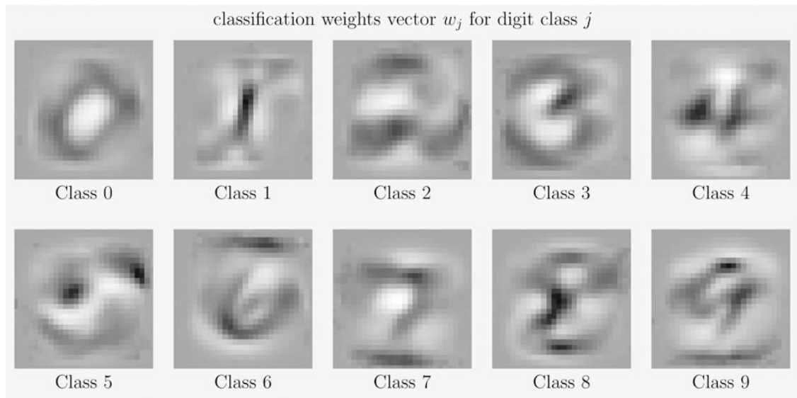
FIG. 26. Visualization of the weights w_j after training a SoftMax Regression model on the MNIST dataset (see Notebook 7). We emphasize that SoftMax Regression does not have explicit 2D spatial knowledge; the model learns from data points flattened out in a one-dimensional array.
