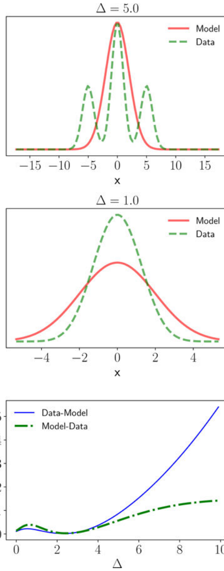
FIG. 70. KL-divergences between the data distribution p_{\text{data}} and the model p_{\theta} . Data is drawn from a Gaussian mixture of the form p_{\text{data}} = 0.25\mathcal{N}(-\Delta) + 0.25 * \mathcal{N}(\Delta) + 0.5\mathcal{N}(0) where \mathcal{N}(a) is a normal distribution with unit variance centered at x = a . p_{\theta}(x) is a Gaussian with \sigma^2 = 2 . (Top) p_{\text{data}} and p_{\theta} for \Delta = 5 . (Middle) p_{\text{data}} and p_{\theta} for \Delta = 1 . (Bottom) D_{KL}(p_{\text{data}}||p_{\theta}) [Data-Model] and D_{KL}(p_{\theta}||p_{\text{data}}) [Model-Data] as a function of \Delta . Notice that D_{KL}(p_{\theta}||p_{\text{data}}) is insensitive to placing weight in the model distribution in regions where p_{\theta} \approx 0 whereas D_{KL}(p_{\text{data}}||p_{\theta}) punishes this harshly.
