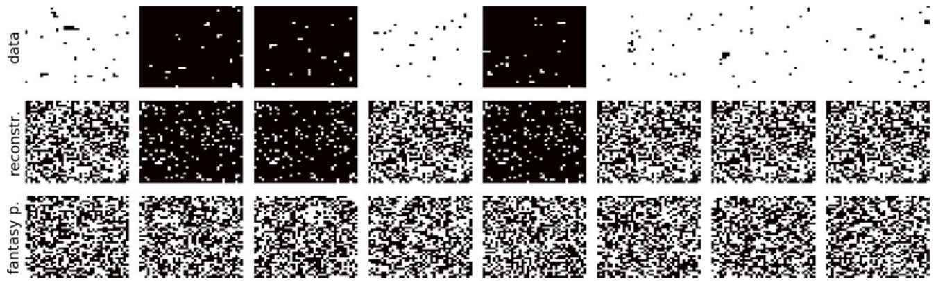
FIG. 66. MC samples, their reconstructions and fantasy particles generated by a Deep Boltzmann Machine in the ordered phase of the the 2D Ising data set at T/J = 1.75 . We used two hidden layers of 1000 and 100 layers, respectively.
