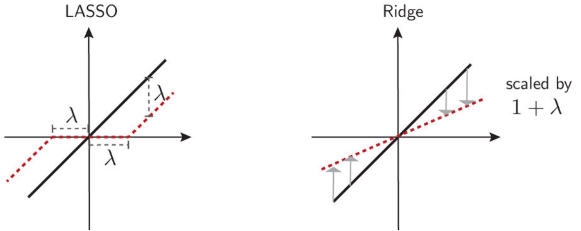
FIG. 12. [Adapted from (Friedman et al. , 2001)] Comparing LASSO and Ridge regression. The black 45 degree line is the unconstrained estimate for reference. The estimators are shown by red dashed lines. For LASSO, this corresponds to the soft-thresholding function Eq. (54) while for Ridge regression the solution is given by Eq. (46)
