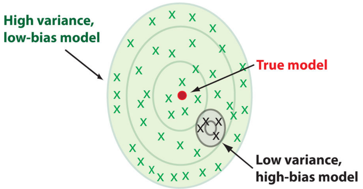
FIG. 6. Bias-Variance tradeoff.
