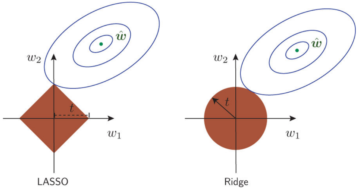
FIG. 13. [Adapted from (Friedman et al. , 2001)] Illustration of LASSO (left) and Ridge regression (right). The blue concentric ovals are the contours of the regression function while the red shaded regions represent the constraint functions: (left) |w_1| + |w_2| \leq t and (right) w_1^2 + w_2^2 \leq t . Intuitively, since the constraint function of LASSO has more protrusions, the ovals tend to intersect the constraint at the vertex, as shown on the left. Since the vertices correspond to parameter vectors \mathbf{w} with only one non-vanishing component, LASSO tends to give sparse solution.
