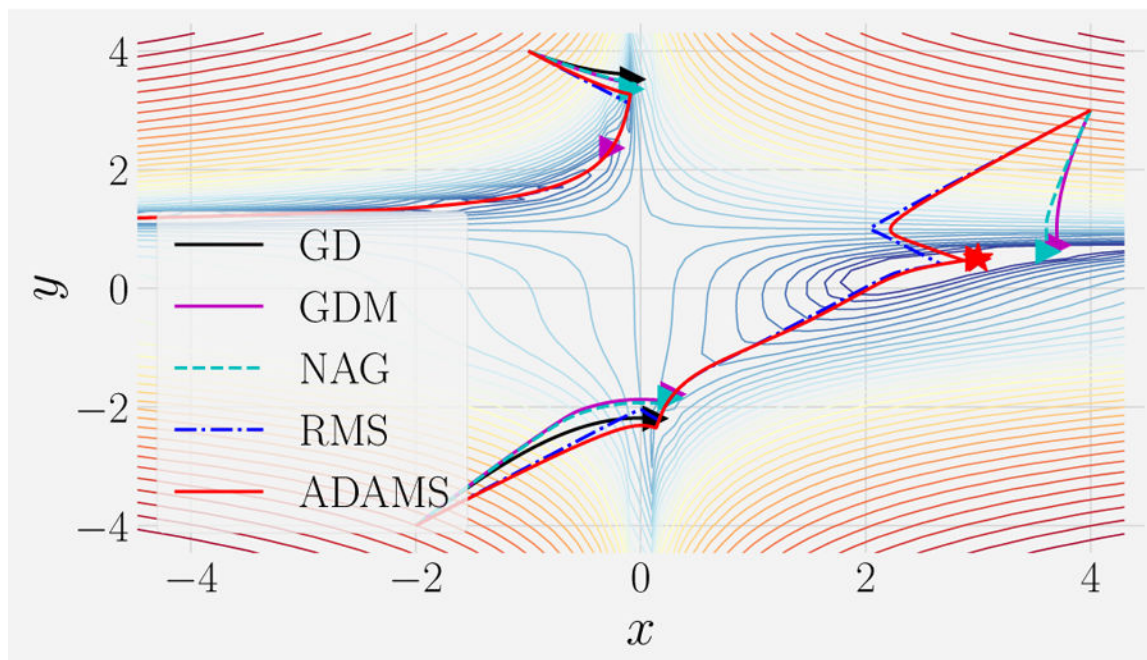
FIG. 9. Comparison of GD and its generalization for Beale's function.
