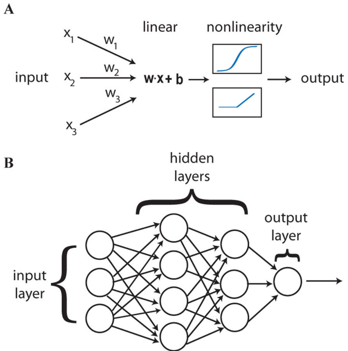
FIG. 34. Basic architecture of neural networks.
