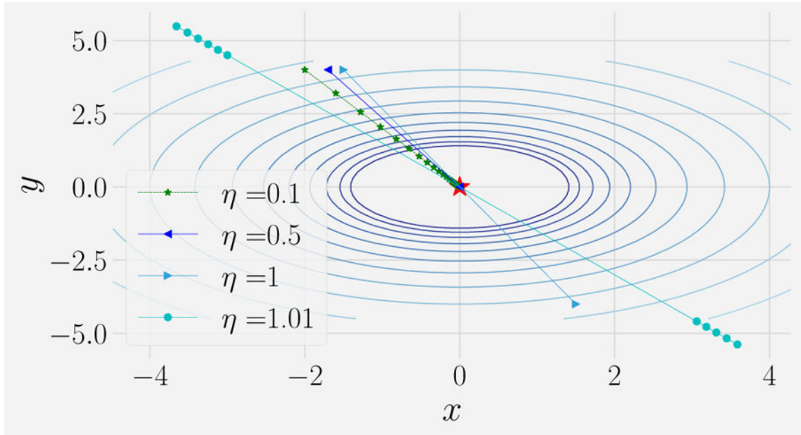
FIG. 7. Gradient descent exhibits three qualitatively different regimes as a function of the learning rate.
