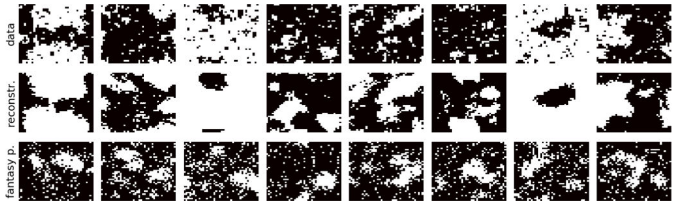
FIG. 67. MC samples, their reconstructions and fantasy particles generated by a Deep Boltzmann Machine in the critical regime of the the 2D Ising data set at T/J = 2.25 . We used two hidden layers of 1000 and 100 layers, respectively.
