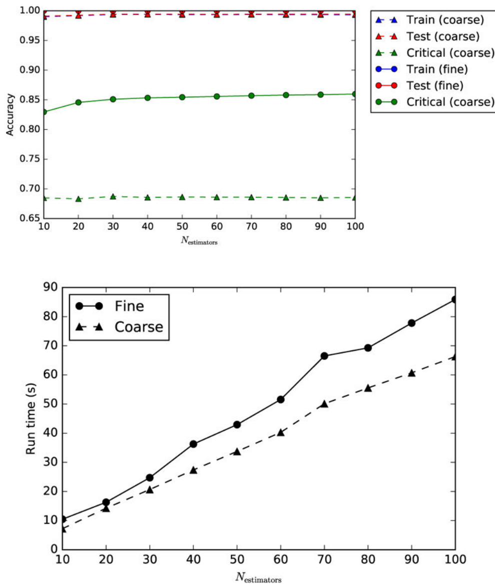
FIG. 32. Using Random Forests (RFs) to classify Ising Phases. (Top) Accuracy of RFs for classifying the phase of samples from the Ising mode for the training set (blue), test set (red), and critical region (green) using coarse trees with a few leaves (triangles) and fine decision trees with many leaves (filled circles). RFs were trained on samples from ordered and disordered phases but were not trained on samples from the critical region. (Bottom) The time it takes to train RFs scales linearly with the number of estimators in the ensemble. For the upper panel, note that the train case (blue) overlaps with the test case (red). Here ‘fine’ and ‘coarse’ refer to trees with 2 and 10,000 leaves, respectively. For implementation details, see Jupyter notebooks 9
