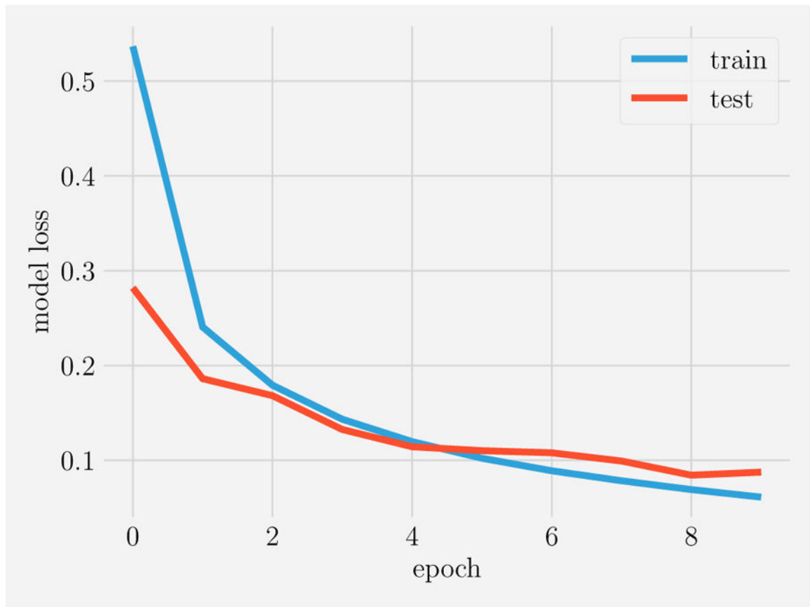
FIG. 38. Model loss of the DNN defined in the main text to study the MNIST problem as a function of the training epochs.
