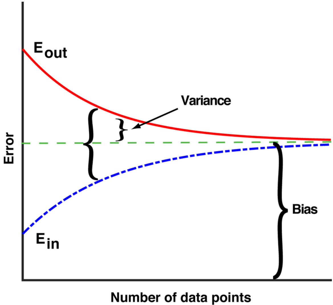
FIG. 4. Schematic of typical in-sample and out-of-sample error as a function of training set size. The typical in-sample or training error, E_{in} , out-of-sample or generalization error, E_{out} , bias, variance, and difference of errors as a function of the number of training data points. The schematic assumes that the number of data points is large (in particular, the schematic does not show the initial drop in E_{in} for small amounts of data), and that our model cannot exactly fit the true function f(x) .
