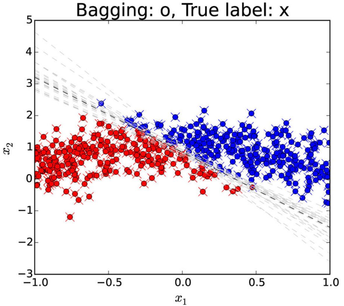
FIG. 29. Bagging applied to the perceptron learning algorithm (PLA).
