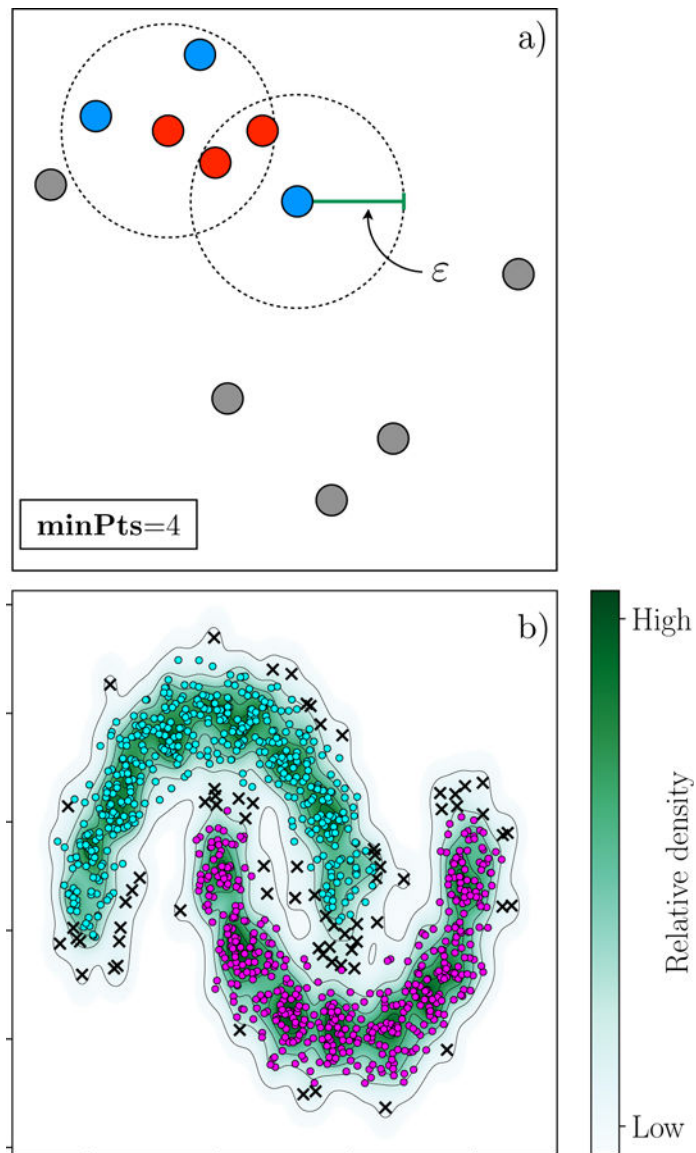
FIG. 57. (a) Illustration of DBSCAN algorithm with minPts = 4. Two \epsilon -neighborhood are represented as dashed circles of radius \epsilon . Red points are the core points and blue points are density-reachable point that are not core points. Outliers are gray colored. (b) Application of DB- ( minPts =40) to a noisy dataset with two non-convex clusters. Density profile is shown for clarity. Outliers are indicated by black crosses.
