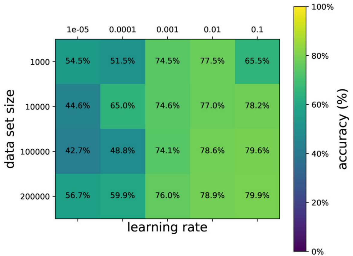
FIG. 40. Grid search results for the test set accuracy of the DNN for the SUSY problem as a function of the learning rate and the size of the dataset. The data used includes all high-and low-level features.
