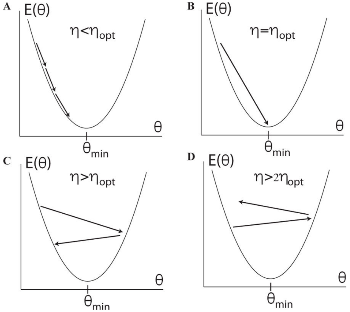
FIG. 8. Effect of learning rate on convergence.
