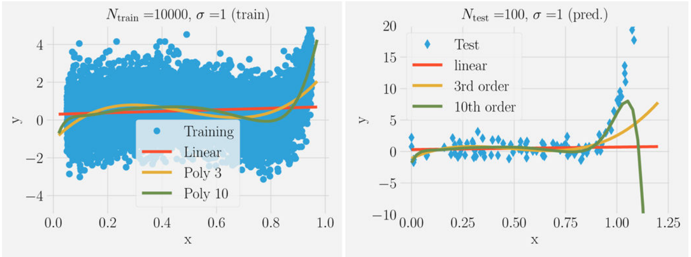
FIG. 3. Fitting versus predicting for noisy data.
