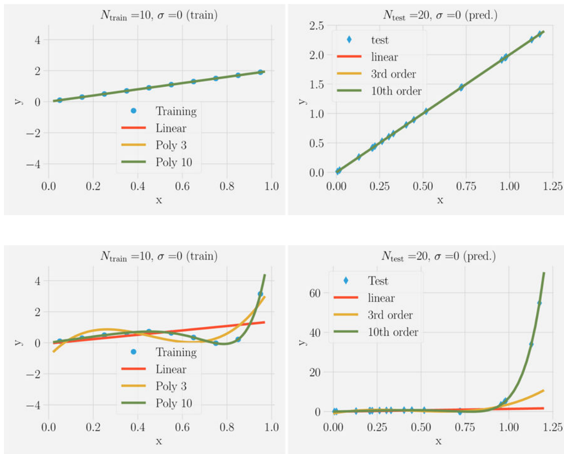
FIG. 1. Fitting versus predicting for noiseless data.
