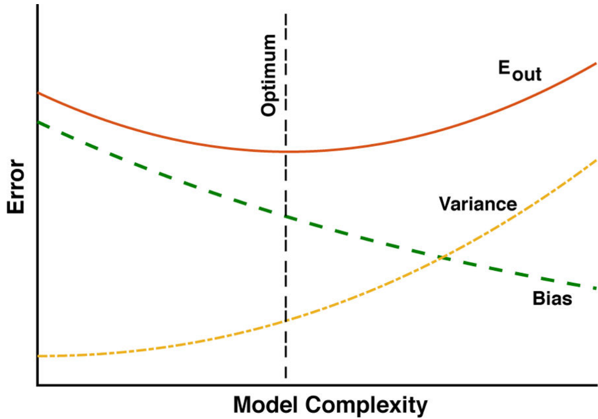
FIG. 5. Bias-Variance tradeoff and model complexity.
