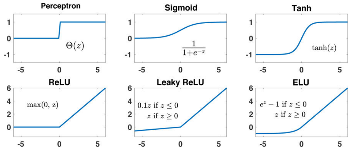
FIG. 35. Possible non-linear activation functions for neurons.
