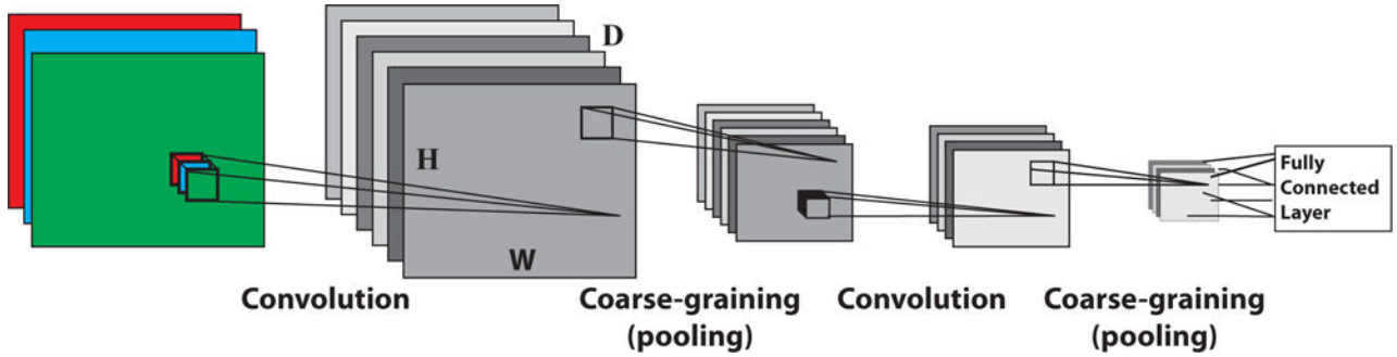
FIG. 42. Architecture of a Convolutional Neural Network (CNN).
