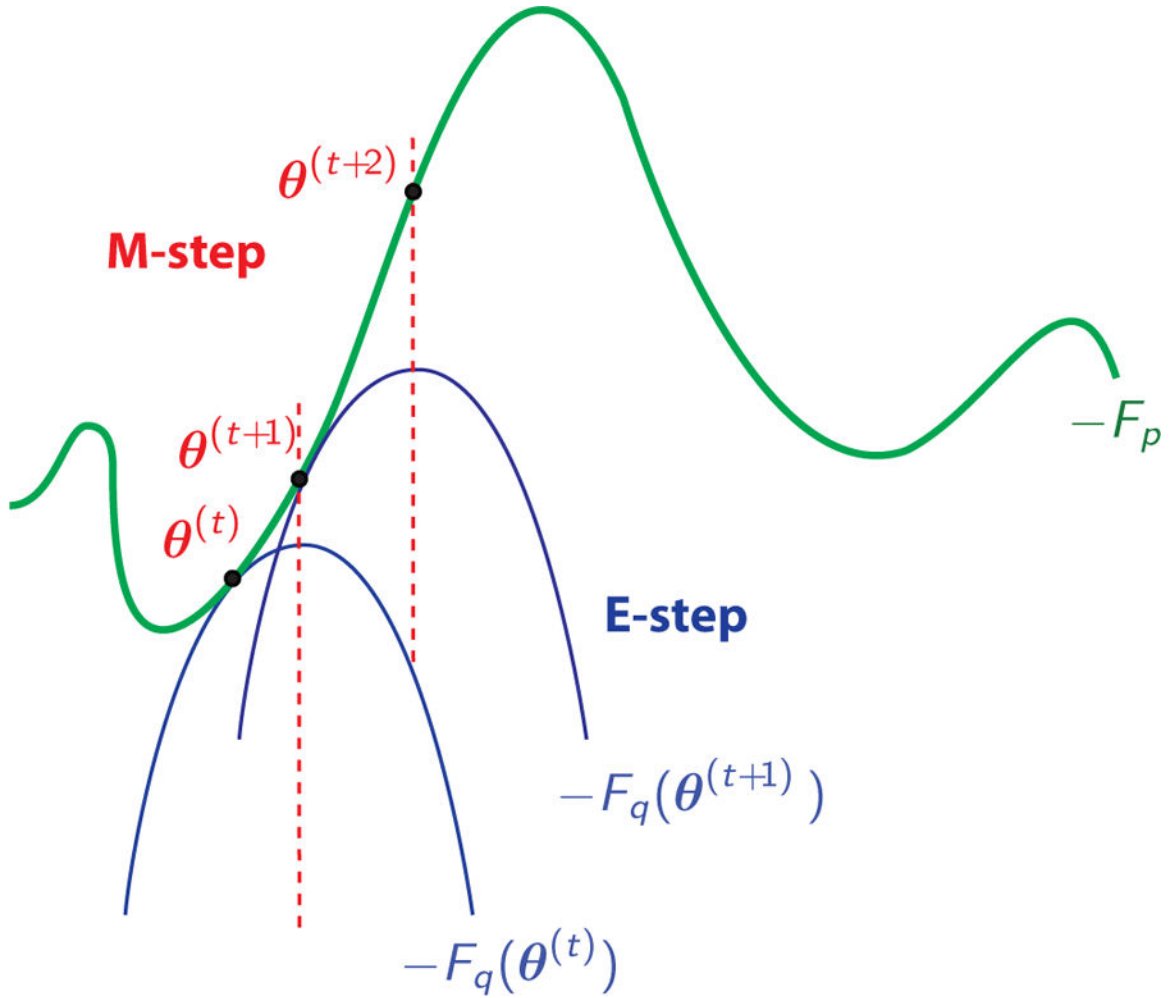
FIG. 59. Convergence of EM algorithm. Starting from \theta^{(t)} , E-step (blue) establishes -F_q(\theta^{(t)}) which is always a lower bound of -F_p := \langle \log p(x|\theta) \rangle_{p_x} (green). M-step (red) is then applied to update the parameter, yielding \theta^{(t+1)} . The updated parameter \theta^{(t+1)} is then used to construct -F_q(\theta^{(t+1)}) in the subsequent E-step. M-step is performed again to update the parameter, etc.
