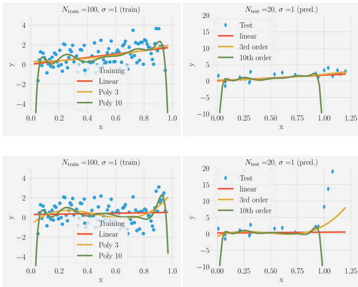
FIG. 2. Fitting versus predicting for noisy data.
