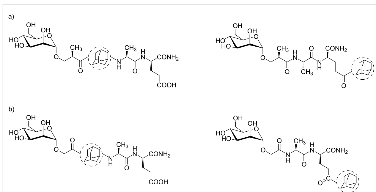
Figure 3: General structure of: a) glycolyl and b) ( R )-hydroxyisobutyryl derivatives.
