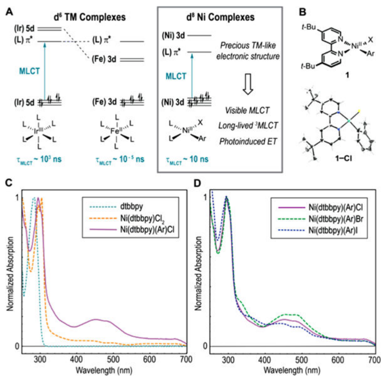
Figure 1. (A) Electronic structure of d 6 photocatalysts compared to Ni(II) aryl halide complexes. (B) Structure of Ni complexes and X-ray crystal structure of 1-Cl . (C) Comparison of component absorption spectra. (D) Absorption spectra for aryl halide complexes.
