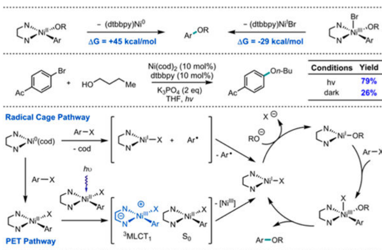
Figure 6. Ni-catalyzed C–O coupling and proposed mechanism. Yields determined by GC-FID using 1-fluoronaphthalene as an external standard.
