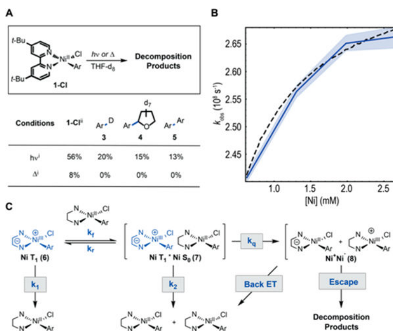
Figure 5. Criteria for bimolecular photoinduced electron transfer. (A) Visible light photolysis and thermolysis experiments. (i) Yield determined by ^1\text{H} NMR. (ii) Conversion is reported. (B) Experimental concentration dependent kinetics (solid blue) plotted together with 95% confidence interval (blue shading) and simulated saturation kinetics (black dashed). (C) Kinetic hypothesis.
