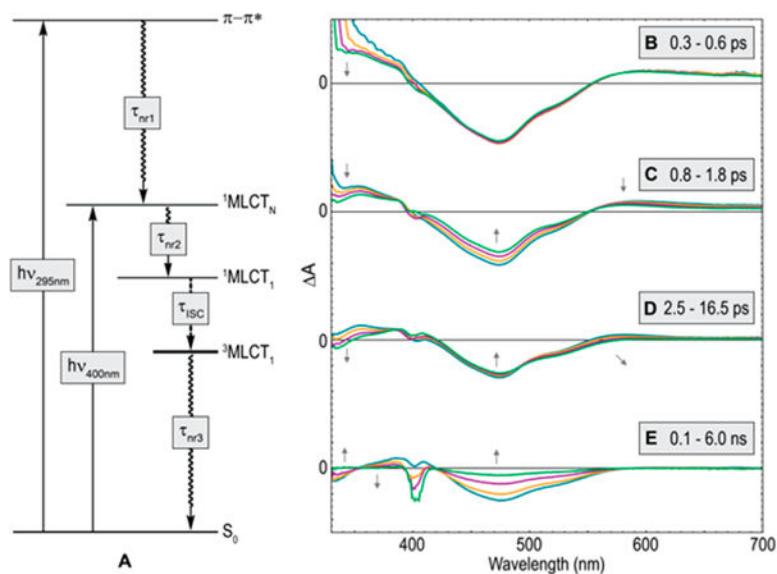
Figure 4. Summary of photophysics Ni(II) aryl halide complexes and evolution of TA spectra for 1-Cl upon visible excitation ( \lambda_{\text{pump}} = 400 \text{ nm} ). (A) Jablonski diagram for all aryl halide complexes. (B) Initial cooling. (C) ISC associated spectral evolution ( \tau_{\text{ISC}} = 1.1 \text{ ps} ). (D) Bleach broadening. (E) Decay to ground state ( \tau_{\text{nr3}} = 4.1 \text{ ns} ). The negative feature at 400 nm is the result of pump scattering.
