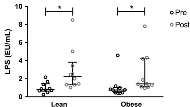
Figure 2. Effect of vancomycin on fasting plasma LPS. Vancomycin treatment significantly increased fasting plasma LPS in both groups (Wilcoxon signed rank test; lean, P = 0.017 ; obese, P = 0.014 ). Lines at median and IQR.
