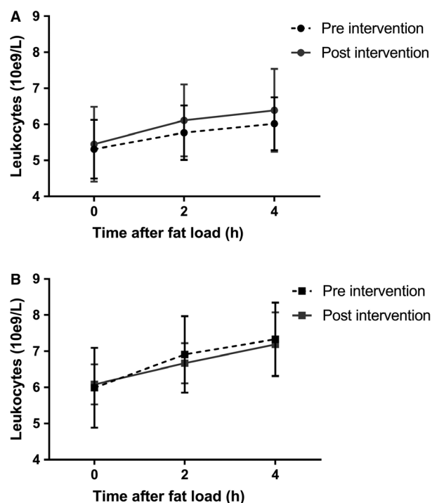
Figure 4. Postprandial blood leukocyte counts. Leukocyte counts significantly increased after the meal in both the lean (A) and obese (B) group (one-way rm-ANOVA: lean, P = 0.006 preintervention and P = 0.001 postintervention; obese, P = 0.001 preintervention and P = 0.003 postintervention). Vancomycin treatment did not affect postprandial leukocyte counts. Graphs show mean and SD.
