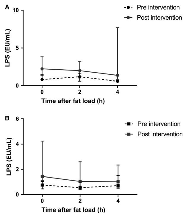
Figure 3. Postprandial LPS concentrations. LPS concentrations did not increase after the high-fat meal in both the lean (A) and obese (B) group. Vancomycin treatment did not affect postprandial LPS concentrations (two-way repeated measures ANOVA, time \times treatment interaction: lean, P = 0.318 , obese, P = 0.714 ). Lines show median and IQR.
