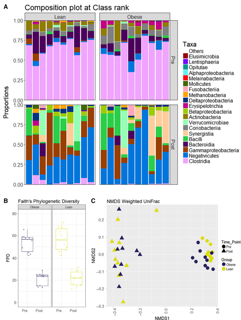
Figure 1. Effect of vancomycin on gut microbiota composition. Fecal microbial community characteristics of obese and lean subjects before and after treatment. Vancomycin treatment resulted in significant changes in gut microbiota composition in both groups. (A) microbial composition showing the 20 most abundant bacterial classes (upper part, preintervention; lower part, postintervention). (B) Faith's phylogenetic diversity distribution showed a significant decrease in alpha-diversity (lean, P < 0.001 ; obese, P < 0.001 ). (C) NMDS ordination of the weighted UniFrac distances showed a significant shift in beta-diversity (lean, P = 0.001 ; obese, P = 0.001 ).
