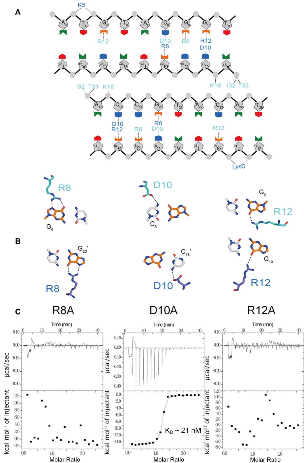
Figure 5. Interaction between KacA and DNA. (A) Schematic overview of the interactions between KacA and DNA. Dashed lines indicate hydrogen bonds or electrostatic interactions with phosphate-sugar backbone and bases. The residues in KacA are shown in colours matching those in Figure 1. (B) Details of the sequence-specific interactions of the antitoxin KacA heterodimer with bases in the operator DNA. (C) Measurement of the binding affinity between the palindromic sequence and the KacAT complex containing KacA mutants using ITC. Individual peaks from titrations were integrated and presented in a Wiseman plot.
