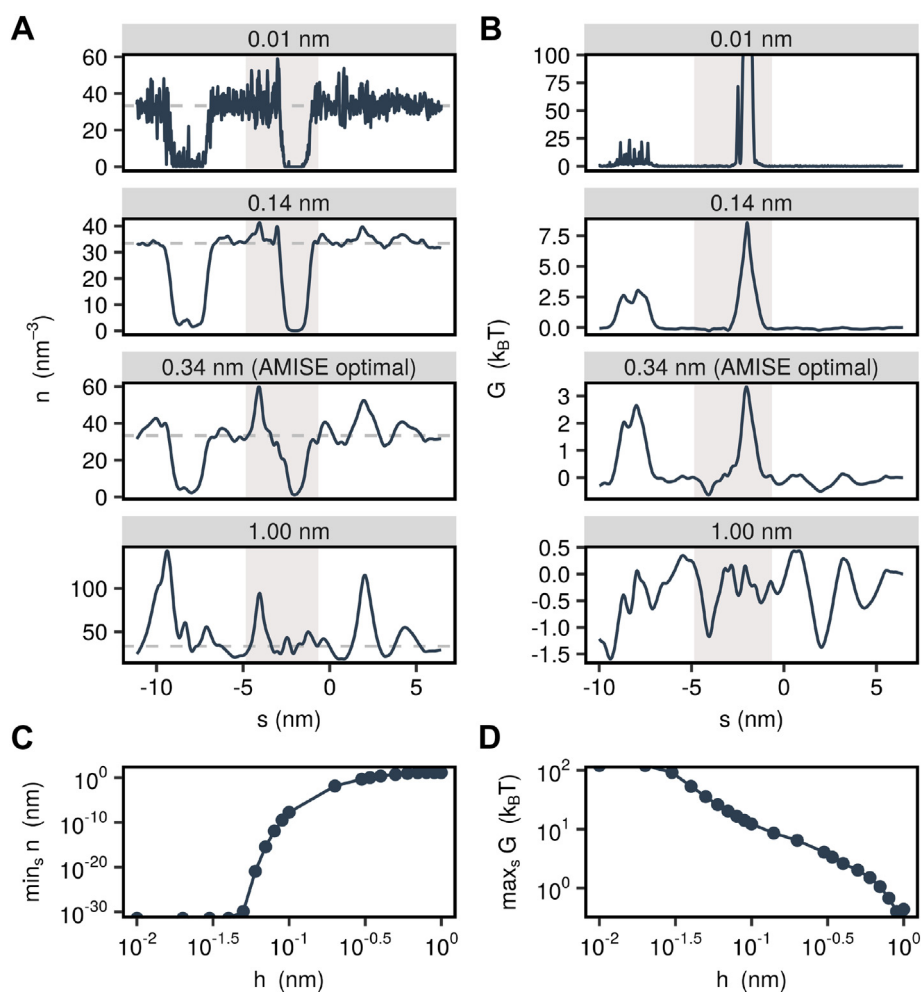
Fig. 7. Influence of bandwidth parameter. (A) Water number density along the permeation pathway of the 5-HT 3 receptor for various values of the kernel bandwidth. A value of 0.14 nm corresponds to the approximate size of a water molecule and a value of 0.34 nm corresponds to the statistically optimal bandwidth. (B) Corresponding free energy profiles calculated via Boltzmann inversion of the density profiles. The gray shaded area in panels A and B represents the transmembrane domain. (C) Minimum of number density profile in dependence of bandwidth. (D) Maximum of free energy profile in dependence of bandwidth.
