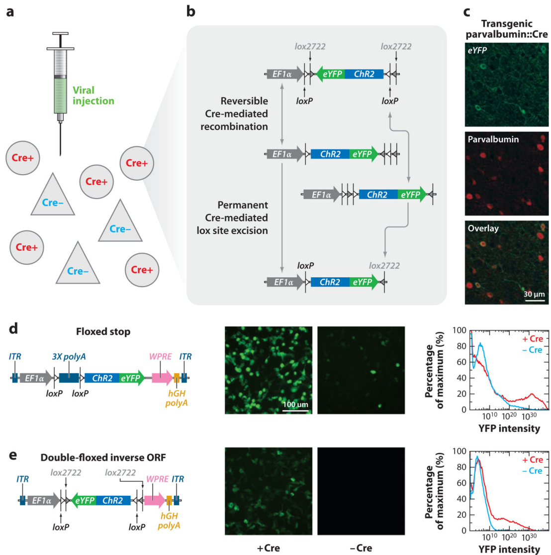
Figure 3. Low-leak Cre-dependent expression using the doublefloxed inverted open-reading-frame (DIO) strategy. The combination of a transgenic mouse expressing Cre recombinase in specific neuronal subtypes and the injection of a virally encoded DIO opsin ( a ) results in the physical inversion of the open reading frame (ORF) in only that population ( b,c ), which may be transient and revert back to the original state or undergo further recombination to be permanently anchored in the sense direction, resulting in functional expression of the opsin ( c ). The DIO strategy may be contrasted with the lox-stop-lox (“floxed STOP”) strategy ( d,e ). In the absence of Cre recombinase, lox-stop-lox ( d ) allows for some level of expression leak as assayed by both enhanced yellow fluorescent protein (eYFP) expression and fluorescence-activated cell sorting (FACS) analysis. Because the ORF of an opsin in DIO configuration encodes nonsense ( e ), there is no functional expression in the absence of Cre recombinase. Adapted with permission from Sohal et al. (2009) and F. Zhang and K. Deisseroth.
