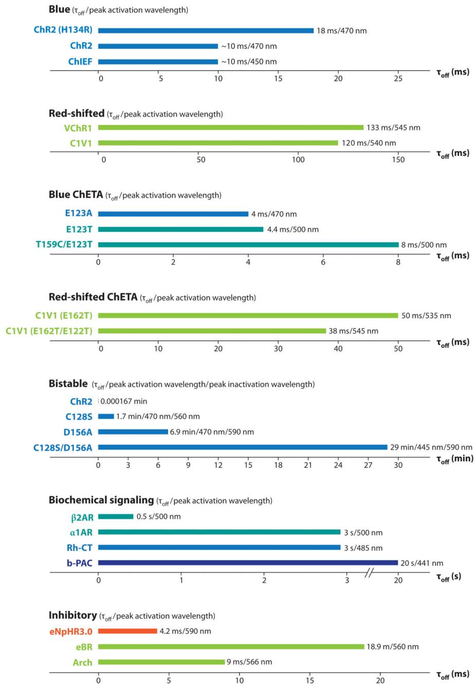
Figure 2. Spectral and kinetic diversification of optogenetic tools. Deactivation time constants ( \tau_{\text{off}} ) and approximate peak activation/inactivation wavelengths are shown for blue light-activated opsins, blue ChETAs (including E123T/T159C) (Berndt et al. 2011, Mattis et al. 2011), red-shifted opsins, red-shifted ChETAs, bistable (SFO) opsins, and modulatory/inhibitory tools in a compact look-up table. ChR2 is listed among the bistable group for scale purposes only. Where precise values are not available, decay kinetics were measured (courtesy of J. Mattis, personal communication) or estimated from published traces; all values were recorded at
