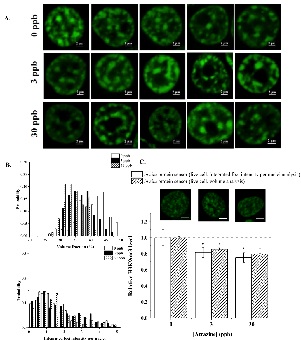
Figure 5. (A) Typical images of HEK293T cells transfected with \Delta CD-\Delta CSD sensors and treated with different concentrations of Atrazine (ATZ). (B) Probability distribution of volume % and IFIN under varying ATZ concentrations. (C) Relative changes in mean volume % and IFIN of transfected cells under varying [ATZ] and a comparison with findings from immuno-assays. n \geq 3 form immuno-assays. n \geq 90 for images-based assays. *: p < 0.05 denoting statistical difference among compared groups. All images are 2D projections of Z-stacks. Scale bar = 2 \mu m .
