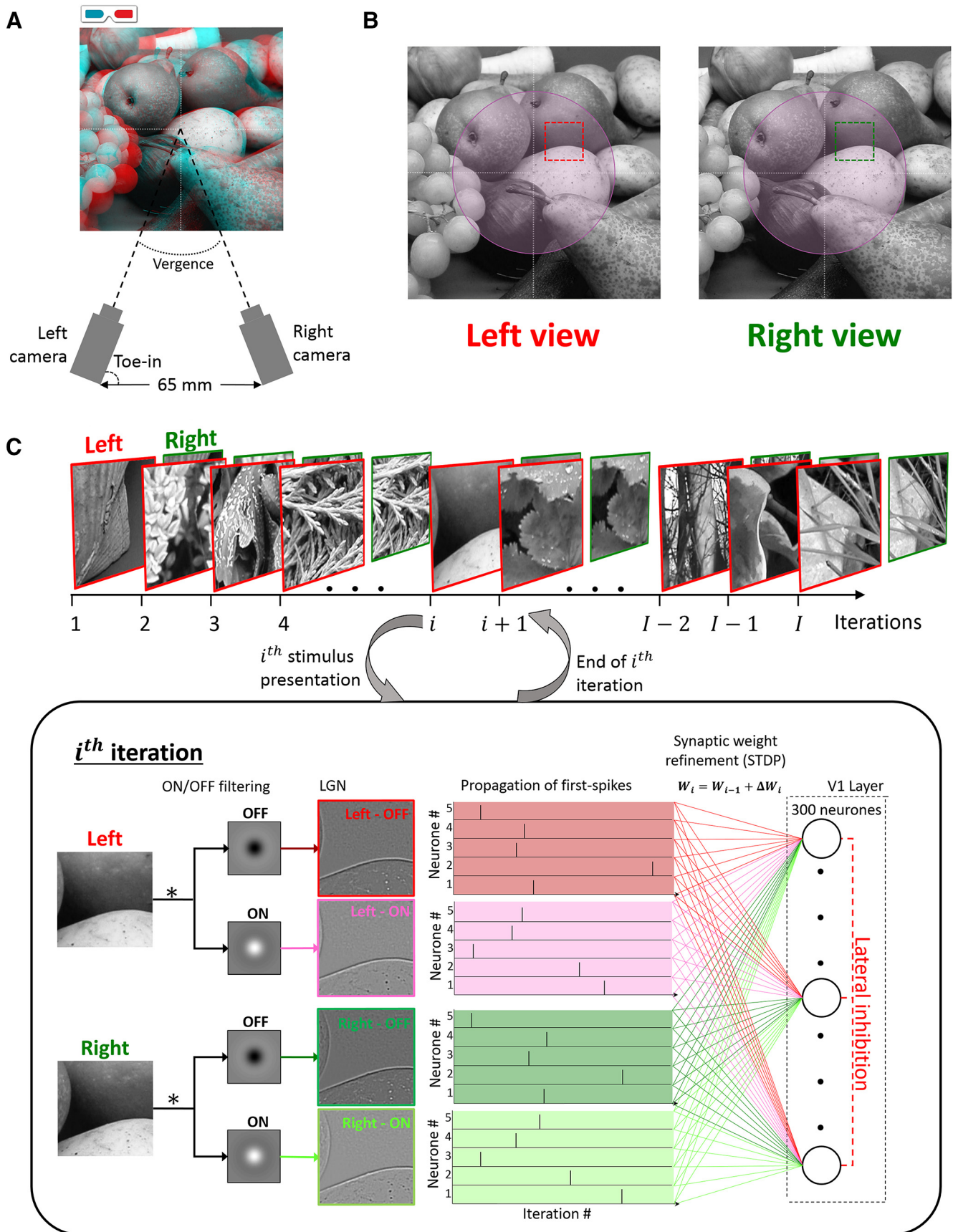
Figure 1. Processing pipeline. A , Acquisition geometry for the Hunter–Hubbard database. The setup mimicked the typical geometry of the human visual system (see more details in the text). This geometry is crucial for capturing realistic disparity statistics from natural scenes. A stereoscopic reconstruction (red-cyan anaglyph) of a sample from the dataset is also shown. B , Input images captured by the left and the right camera for the scene shown in A . The subtle differences in the images (disparity) provide important cues about the 3-D structure of the scene. Depending on the simulation, an ROI in the visual field was identified, and inputs were sampled only within this ROI (foveal ROI illustrated in purple). Each sample consisted of two ( Figure legend continues. )
