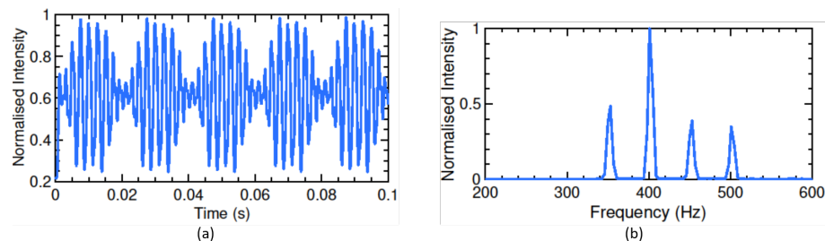
Fig. 2. (a) An example of a signal, captured by the photodetector (b) its Fourier Transform showing the four distinct peaks, corresponding to the four different frequencies.
