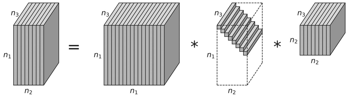
Fig. 3. The t-SVD of an n_1 \times n_2 \times n_3 tensor.
