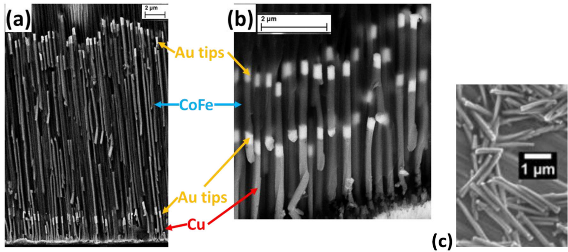
Fig. 2. Cross-sectional SEM images of \text{Co}_{35}\text{Fe}_{65} nanowires 16 μm (a) and 2 μm (b) aligned in an AAO template. The Cu layers at the bottom were dissolved by 1 M \text{FeNO}_3 before dissolving the AAO template. Note, some of the NWs were broken when the AAO template was cleaved to make these cross-sectional images. (c) Released Au-tipped Ni nanowires.
