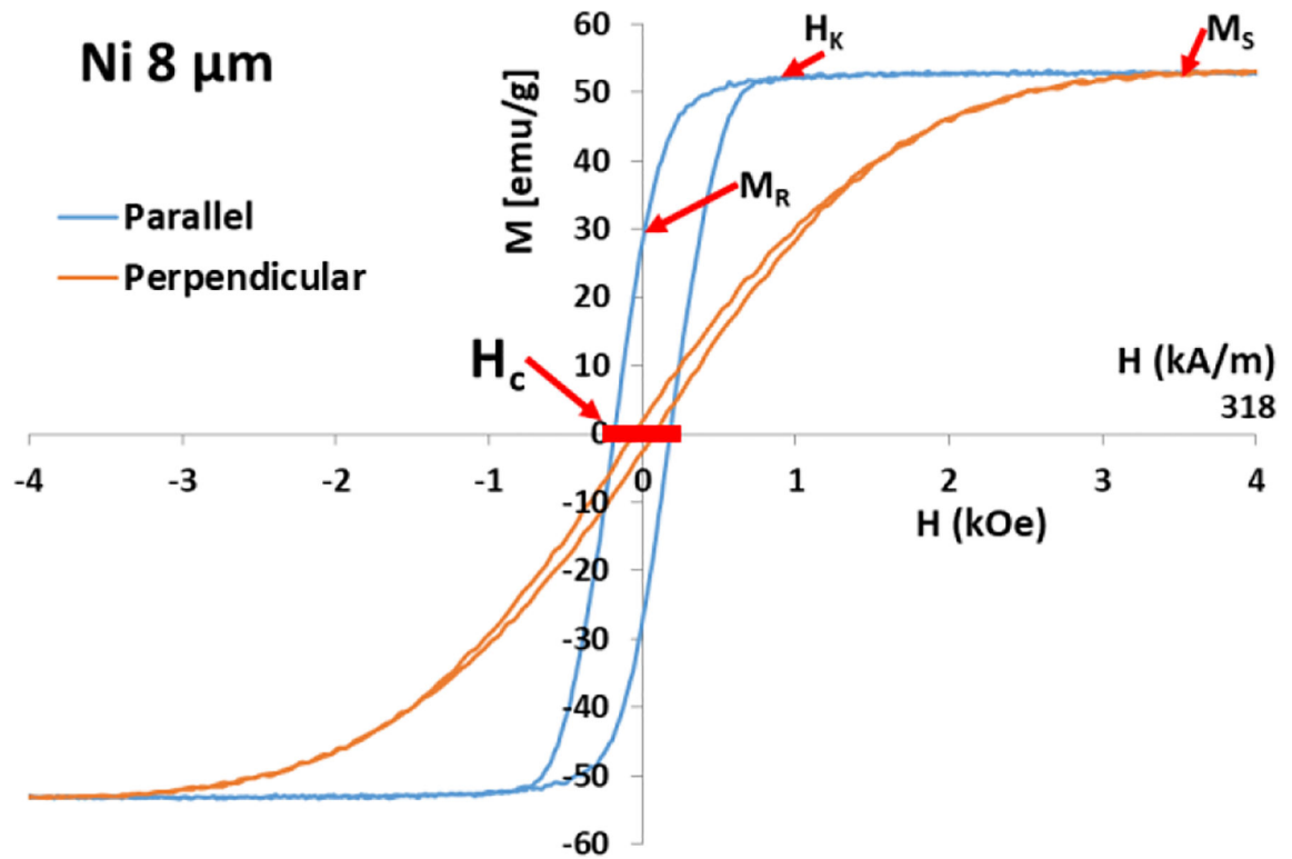
Fig. 1. Hysteresis loop for 8 \mu\text{m} Ni nanowires aligned in an AAO membrane parallel and perpendicular to the applied field. Red arrows indicate the important magnetic parameters. H is the applied magnetic field and M is the magnetization. Thick red line shows range of field used in SAR measurements.
