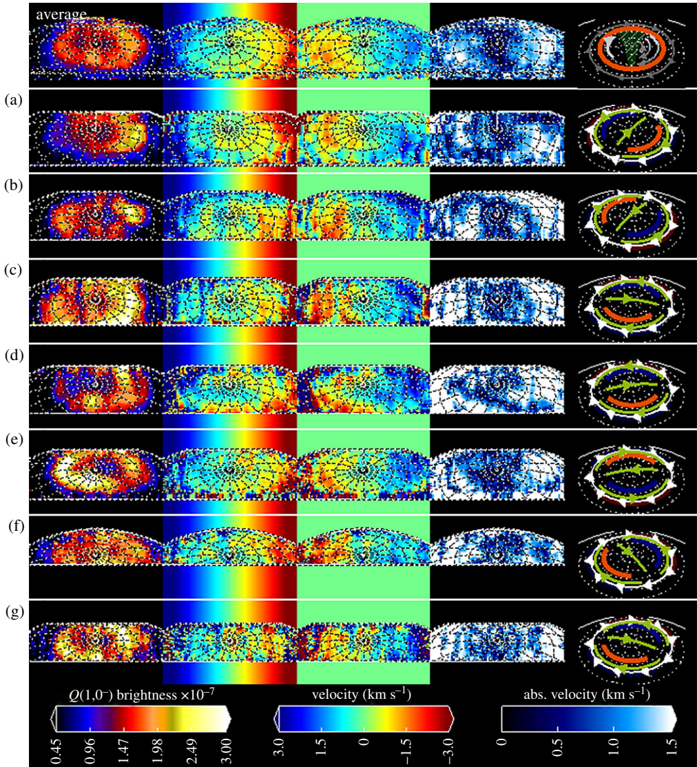
Figure 5. The H_3^+ brightness and ion winds. The first column shows H_3^+ emission brightness scaled between 0.45– 3 \times 10^{-7} \text{ W m}^{-2} \mu\text{m}^{-1} . The second column shows the line-of-sight velocity with ranged between blue and red shifts of 3 \text{ km s}^{-1} . The third column shows the same velocity once the rotation rate of the planet is removed. The fourth column shows the absolute value of the winds, here scaled to 0\text{--}1.5 \text{ km s}^{-1} ; this provides a quick view of where the planet it co-rotating (black) and significantly sub-corotating (white). The final column shows the predicted direction of ion wind flows driven by the planetary period current system based upon the average northern phase, assuming the thermosphere is driving ion winds (green), along with the location of auroral enhancement caused by this current system. Each row shows a separate night, as described in table 2, with the final row showing the average value across each night.
