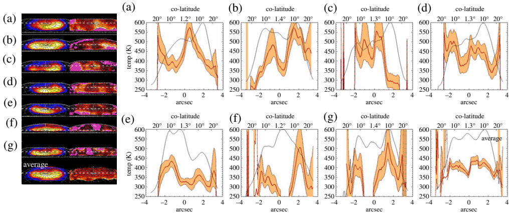
Figure 8. One-dimensional profiles of line-of-sight corrected H_3^+ intensity and temperature. These are smoothed by 1.0'' \times 1.0'' . On the left are maps of intensity and temperature. The first column of maps shows the line-of-sight corrected H_3^+ emission scaled between 15 and 100% of the maximum intensity, again using the same linear colour scale as is shown in the intensity colour bar in figure 7 (instead scaled between 15 and 100%). The second column of maps shows temperature ranging between 250 and 600 K, using the exact same temperature scale as is shown in figure 7. The position of the profiles is shown as a dashed white line over these. On the right, 1-d profiles of normalized line-of-sight corrected intensity (thin line) and temperature (bold red line) are shown. Temperature errors are shown in the shaded region around the temperature (orange infill). Individual profiles can be identified by the letter in the top right corner, described in table 2. (Online version in colour.)
