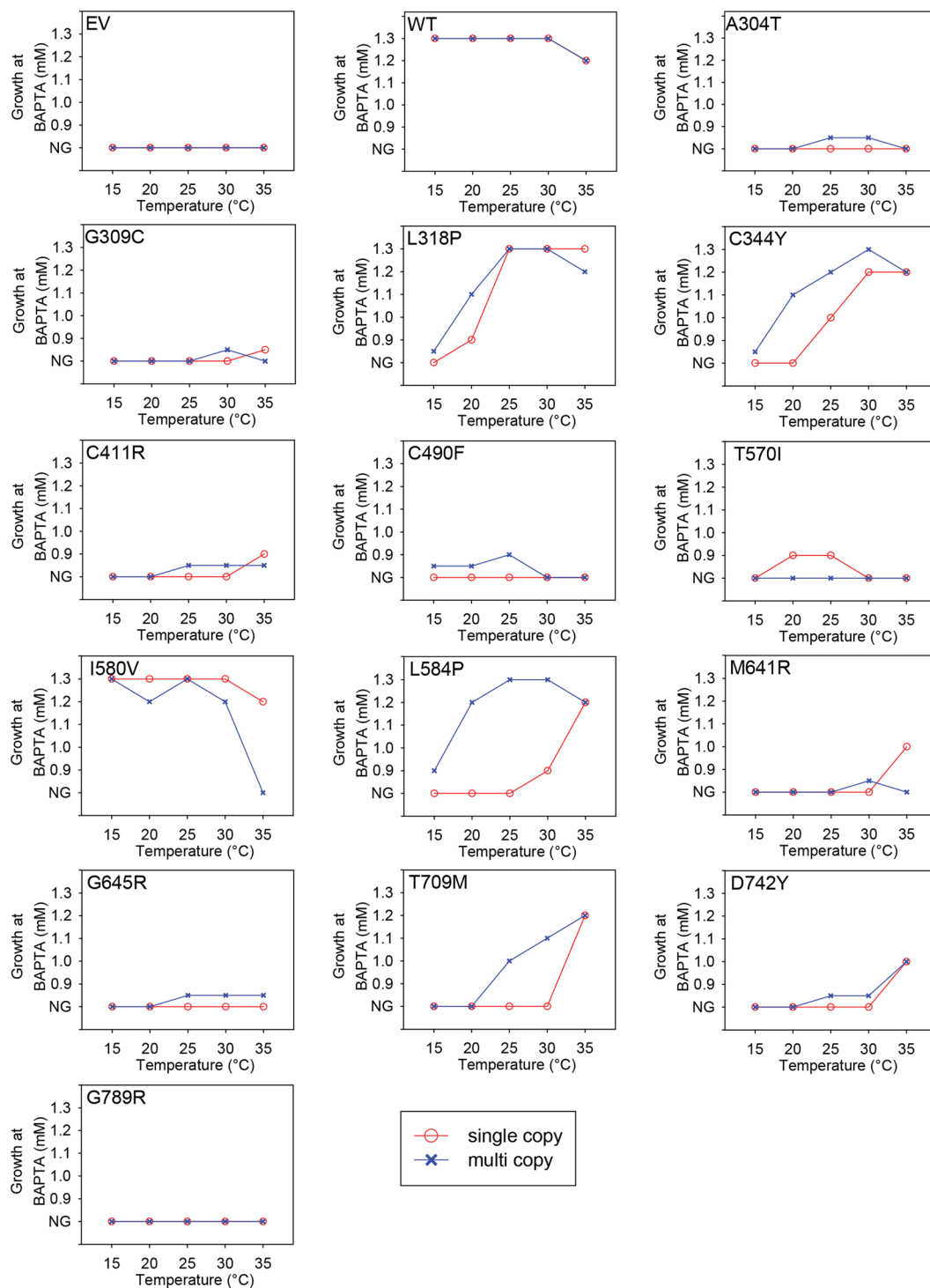
Figure 7. Expression of various ATP2C1a alleles confers a temperature dependent complementation profile. The maximal BAPTA concentration allowing generation of a growth spot at 15 °C, 20 °C, 25 °C, 30 °C and 35 °C was determined from the complementation assay in Fig. 6 and plotted with respect to temperature. Blue curves represent expression from the 2 \mu based plasmid, pPAP4997, while red curves are based upon expression from the single copy integrative plasmid pPAP5480. Mutants that showed growth at 0.9 mM BAPTA that was considerably better than the empty vector, but still poorer than wt were given a value between no growth (NG) and 0.9 mM BAPTA. The temperature profiles categorized each mutation as either cold sensitive (CS), heat sensitive (HS) or temperature insensitive (TI) when compared to that of wt.
