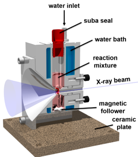
Figure 1. Schematic representation of a cross-section of the bespoke stirrable reaction cell used for in situ SAXS experiments performed during RAFT aqueous emulsion polymerization of MOEMA at 70 °C. The volume of reaction solution within this cell is approximately 2.0 mL, which provides sufficient diblock copolymer (~200 mg) for postmortem analysis using multiple characterization techniques (see main text for further details).
