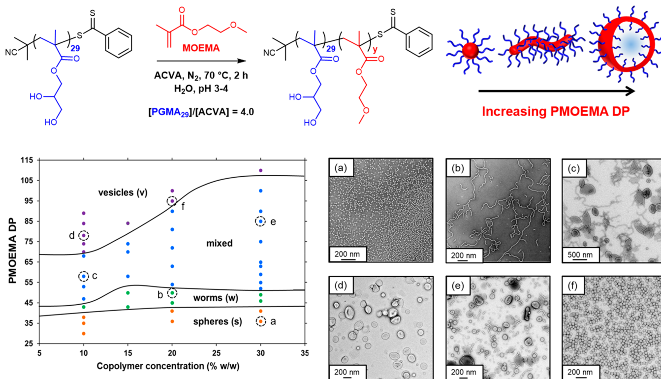
Figure 2. Synthesis of \text{PGMA}_{29}\text{-PMOEMA}_y diblock copolymer nano-objects via RAFT aqueous emulsion polymerization of MOEMA using a water-soluble \text{PGMA}_{29} precursor block at 70 °C, where y ranges from 30 to 110. Phase diagram constructed for \text{PGMA}_{29}\text{-PMOEMA}_y diblock copolymer nano-objects synthesized via RAFT aqueous emulsion polymerization of MOEMA at copolymer concentrations ranging from 10 to 30% w/w. Representative TEM images recorded for: (a) \text{PGMA}_{29}\text{-PMOEMA}_{36} spheres prepared at 30% w/w; (b) \text{PGMA}_{29}\text{-PMOEMA}_{45} worms prepared at 20% w/w; (c) a \text{PGMA}_{29}\text{-PMOEMA}_{38} mixed phase comprising worms, jellyfish and vesicles prepared at 10% w/w; (d) \text{PGMA}_{29}\text{-PMOEMA}_{78} vesicles prepared at 10% w/w; (e) a \text{PGMA}_{29}\text{-PMOEMA}_{85} mixed phase (comprising spheres, worms and vesicles) prepared at 30% w/w; (f) \text{PGMA}_{29}\text{-PMOEMA}_{95} vesicles prepared at 20% w/w.
