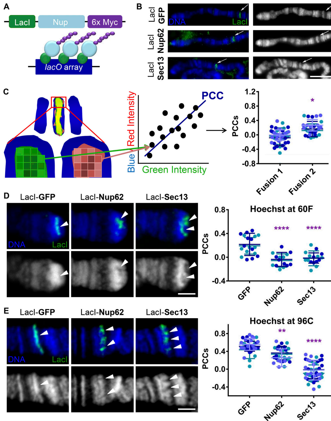
Figure 1. Ectopic targeting of Nups to chromatin induces chromatin decondensation at multiple genomic locations. (A) Schematic of lacO - Lacl - Nup -inducible chromatin tethering system. (B) Widefield IF of squashed polytene chromosomes with Hoechst stain (labeled DNA and shown as blue or white/gray here and hereafter) and \alpha - Lacl (green). The right column shows Hoechst only in grayscale, whereas the left column shows the overlay of both channels. Arrows point to the lacO integration site at location 4D5 near the end of the X chromosome. Lacl -fusion protein expression was driven with second chromosome Nubbin-Gal4. The scale bar is 10 \mu m. (C) Schematic of the PCC method of analyzing fluorescence changes, where intensities of blue Hoechst or red protein of interest and green ( Lacl ) are measured pixel-by-pixel under green-defined Lacl -band, the PCC value between blue/red and green is determined for each image, and \sim 30 PCC values are measured per genotype. Example significance of P < 0.05 (*). (D) Confocal IF images of Lacl -fusion proteins targeted to the subtelomeric lacO integration site on squashed polytene chromosomes at location 60F stained with Hoechst (blue or white) and \alpha - Lacl (green). The top row shows the overlay of both channels, and the bottom row shows Hoechst only. "Holes" (areas of highly reduced staining density) in Hoechst staining can be reproducibly observed under Lacl - Nup binding. Expression was driven with Sgs3 -Gal4. Arrowheads show observed decondensation or lack thereof under Lacl . The scale bar is 2 \mu m. Quantification displays PCCs between blue and green signal under Lacl . Data are from two biological replicates (colored), each from an independent experiment. GFP, n = 19 ; Nup62 , n = 15 ; Sec13 , n = 17 . ****, P < 0.0001 . Error bars represent SDs. (E) Experimental conditions, staining, and imaging are identical to D above, with the replacement of cytological location 60F with location 96C and Nubbin-Gal4 driver. Holes in Hoechst can reproducibly be observed under Lacl - Sec13 and occasionally under Lacl - Nup -62. Data are from three biological replicates (colored) from two independent experiments. GFP, n = 39 ; Nup62 , n = 27 ; Sec13 , n = 44 . ****, P < 0.0001 ; **, P < 0.01 . Error bars represent SDs. The image for control Lacl -GFP is the same as the image for control Lacl -GFP in Fig. 2 A.
