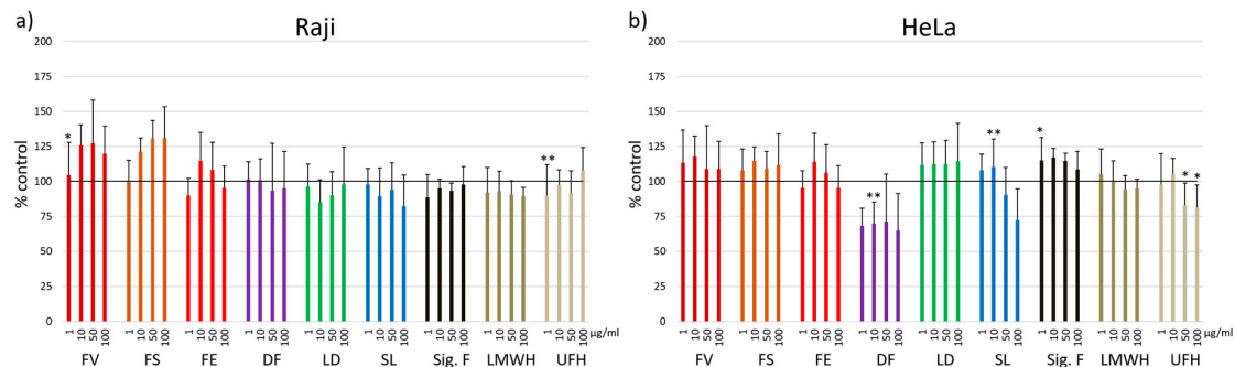
Figure 2. Cell viability was determined using MTS assay after 72 h incubation with 1, 10, 50 and 100 \mu\text{g/mL} fucoidan from Fucus vesiculosus (FV), Fucus serratus (FS), Fucus distichus subsp. evanescens (FE), Dictyosiphon foeniculaceus (DF), Laminaria digitata (LD) and Saccharina latissima (SL) as well as the reference substances Sigma-Aldrich fucoidan ( F. vesiculosus ) (Sig. F), enoxaparin (LMWH) and heparin (UFH). Two different cell lines were tested: a) Raji, b) HeLa. Values are expressed as mean and standard deviation in relation to untreated cells (100%). Significances compared to control were determined using student's t-test * p < 0.05 , ** p < 0.01 , n = 3 \times 3 .
