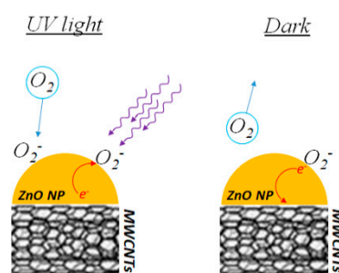
Figure 8. A scheme of the processes taking place on the ZnO–CNT system under UV light irradiation.
