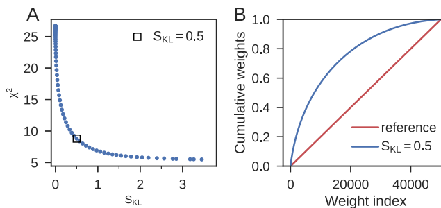
Figure 6. BioEn optimization for Ala-5. (A) L-curve analysis to determine the optimal value of the confidence parameter \theta by plotting \chi^2 as a function of S_{KL} for different values of \theta . (B) Cumulative weight of rank-ordered w_\alpha for the uniformly distributed reference weights w_\alpha^0 (red) and for optimized weights (blue) at \theta = 6.65 with S_{KL} \approx 0.5 .
