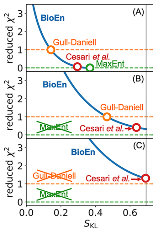
Figure 8. MaxEnt approaches to ensemble refinement as special cases of BioEn. For BioEn optimal ensembles, we plot the reduced \chi^2 and the relative entropy S_{\text{KL}} parametrized by the confidence parameter \theta (blue). The solution of Gull–Daniell-type 60 methods is given by the intersection of this curve with \chi^2 = 1 (orange), of traditional MaxEnt methods 20,22,61,62 by the intersection with \chi^2 = 0 (green), and of the method of Cesari et al. 25,30 by the BioEn solution for \theta = 1 (red). For a simple model ( M \times N = 1 \times 2 , y = (0,1) , \sigma = 0.14 ), we vary the experimental value Y , top to bottom. (A) All methods provide a solution for an experimental value Y = 0.09 within the range of calculated observables. (B) Traditional MaxEnt methods fail to give a solution for Y values outside this range ( Y = 1.08 ). (C) Both traditional MaxEnt and Gull–Daniell-type methods fail to give a solution where a reduced \chi^2 \leq 1 cannot be realized by reweighting ( Y = 1.16 ). The vertical gray lines indicate the maximum value S_{\text{KL}} = \ln(2) for a two-state system.
