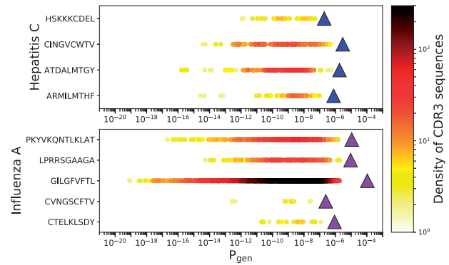
Fig. 4. Generation probabilities of human CDR3s that respond to hepatitis C and influenza A epitopes. P_{\text{gen}}^{\text{aa}} of sequences that respond to an epitope are plotted as circles (color encodes density of the points). The fraction of the repertoire specific to each epitope ( P_{\text{gen}}^{\text{func}} as defined in Eq. 7) is obtained as the sum of the P_{\text{gen}}^{\text{aa}} for each of the corresponding sequences (values plotted as triangles) (Color version of this figure is available at Bioinformatics online.)
