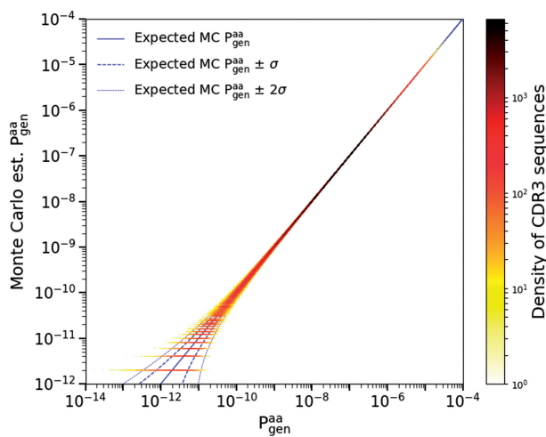
Fig. 2. Monte Carlo estimate of the generation probability of amino acid CDR3 sequences, P_{\text{gen}}^{\text{paa}} , versus OLGA's predictions (mouse TRB). The horizontal lines at the lower left of the plot represent CDR3s that were generated once, twice, etc., in the MC sample. The one- and two-sigma curves display the deviations from exact equality between simulated and computed P_{\text{gen}} to be expected on the basis of Poisson statistics
