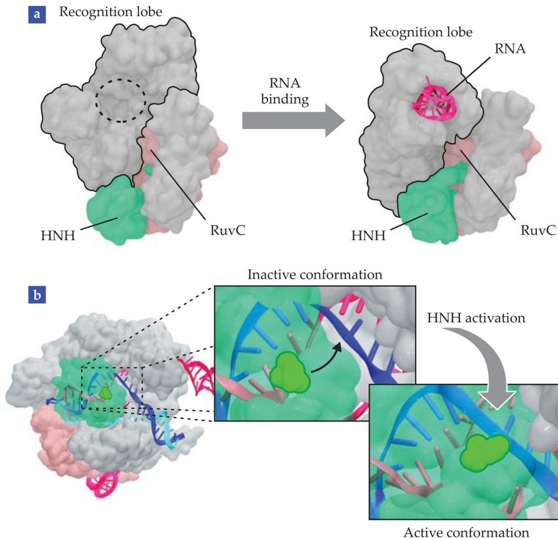
FIGURE 4. MOLECULAR MECHANISMS OF CRISPR-CAS9, revealed by molecular dynamics simulations. (a) Rearrangements made to the recognition lobe reshape the molecular architecture of unbound Cas9 into its RNA-bound conformation. (b) The movement of HNH into its final catalytic state prepares it to cleave the DNA. The conformational change, shown as insets, brings the HNH catalytic residue close to the cleavage site in the DNA complementary strand. In all structures, Cas9 nuclease domains HNH and RuvC are green and pink, respectively. RNA is magenta; DNA is dark blue (complementary strand) and light blue (noncomplementary strand).
