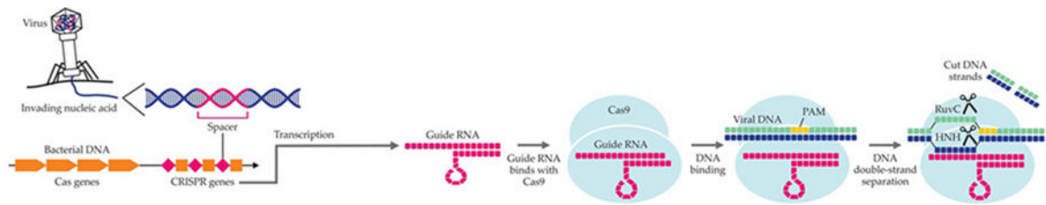
FIGURE 1. CRISPR-CAS9 IMMUNE DEFENSE MECHANISM.
