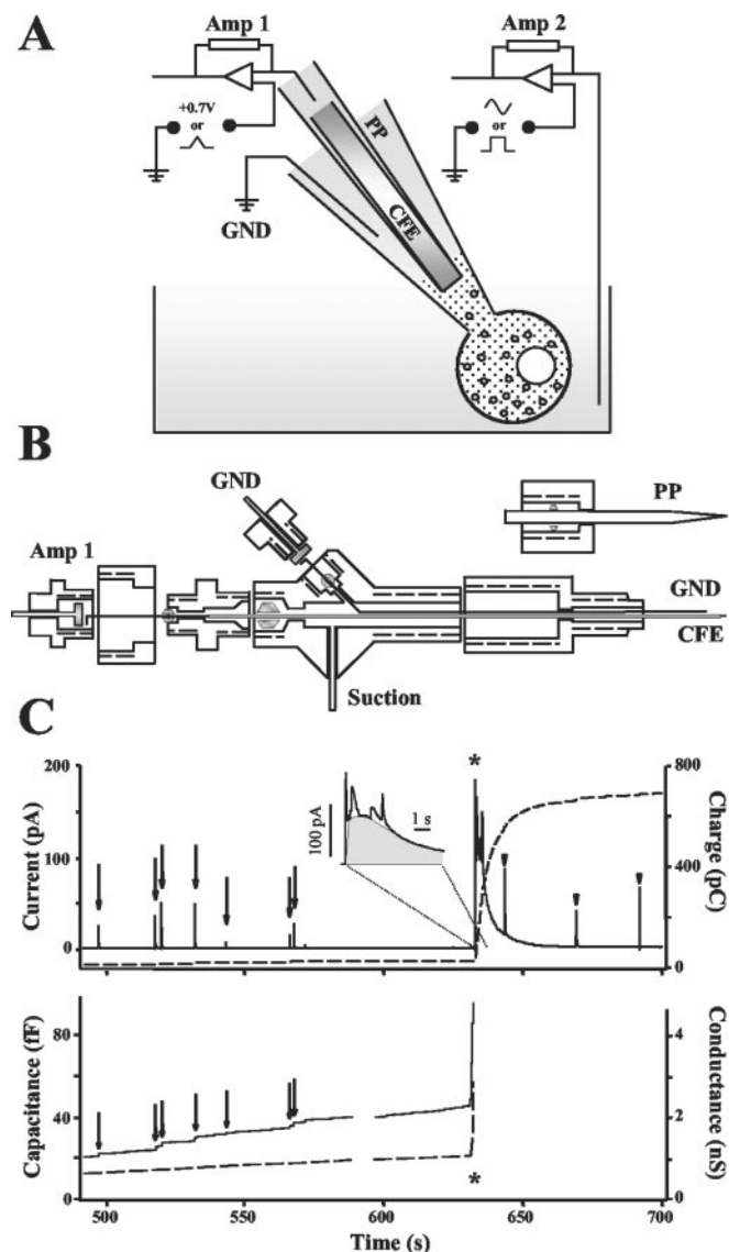
Figure 1. A , Schematic diagram of the IPE setup. Amp 1, Amp 2, Amplifiers; GND, electric ground; CFE, carbon fiber electrode; PP, patch pipette. B , Design of the IPE electrode holder. Two Ag|AgCl wires are connected to the GND and Amp 1 via golden-plated pins. The ground wire is in contact with the PP saline; an electrode wire supplies electric current to the CFE via polyethylene tubing filled with 3 M KCl. Air tightness between different compartments inside the holder is achieved by four rubber O-rings. C , An amperometric recording from a bovine chromaffin cell in which measurement of quantal release of catecholamines by patch amperometry is followed by IPE in amperometric mode. Asterisks indicate the time when the patch was disrupted by suction and a whole-cell configuration was attained. Amperometric current from the CFE (top, solid line), its running integral (top, dashed line), membrane capacitance (bottom, solid line), and conductance (bottom, dashed line) were monitored simultaneously during the same recording. Quantal events in the patch are indicated by amperometric spikes and capacitance steps (arrows). In ~50% of the recordings, the slow amperometric current wave had superimposed quantal spikes, indicating vesicles diffusing out of the cell and bursting on contact with the CFE (arrowheads). The inset displays a magnification of the initial phase of the slow oxidation wave. The first sharp peak from the left is an artifact resulting from suction. The gray area shows the portion of the peak considered to represent the cytosolic molecules.
