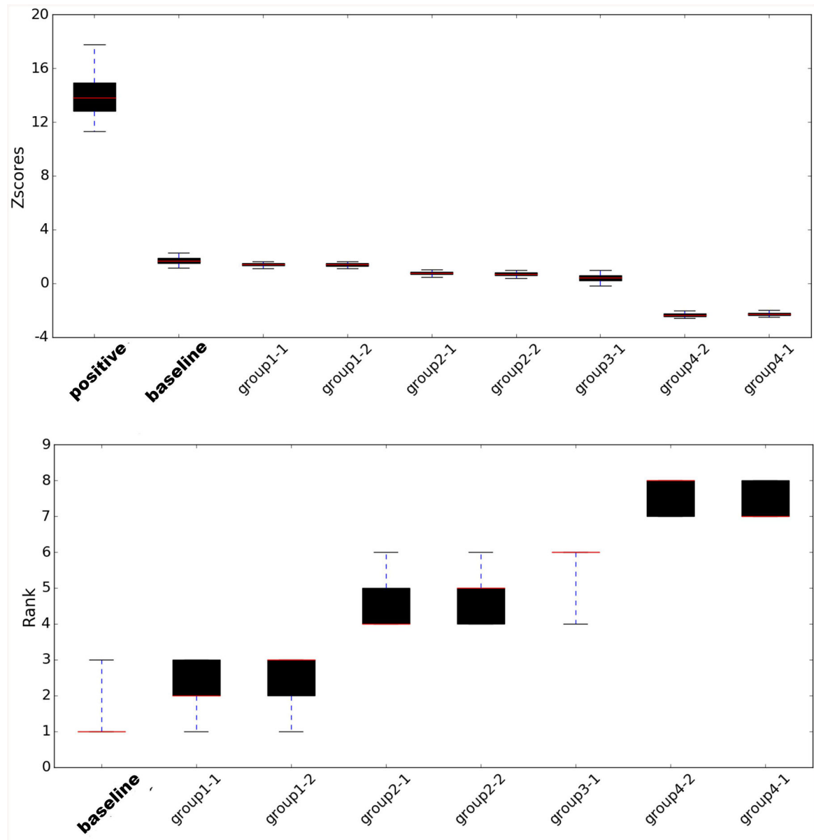
Figure 4. Statistical robustness of Z-scores and rank of predictors.
