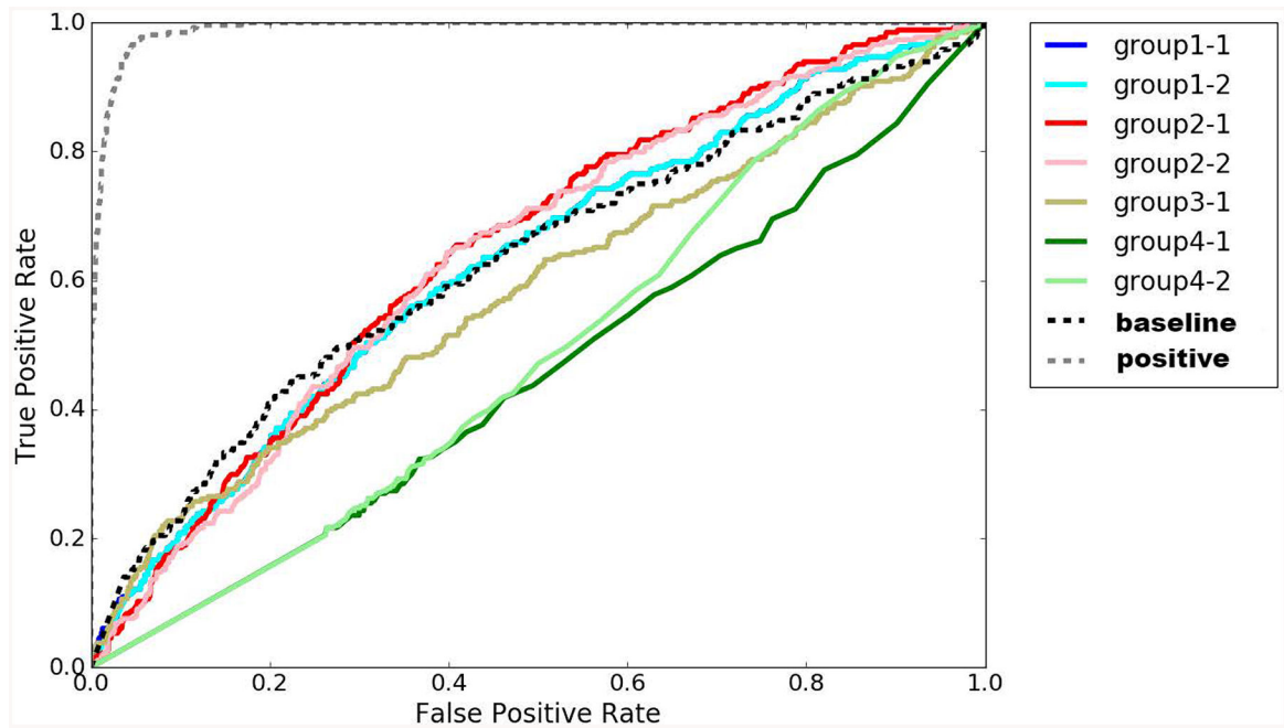
Figure 5. ROC showing performance of predictors for predicting deleterious variants. baseline, baseline predictor; positive, positive control.
