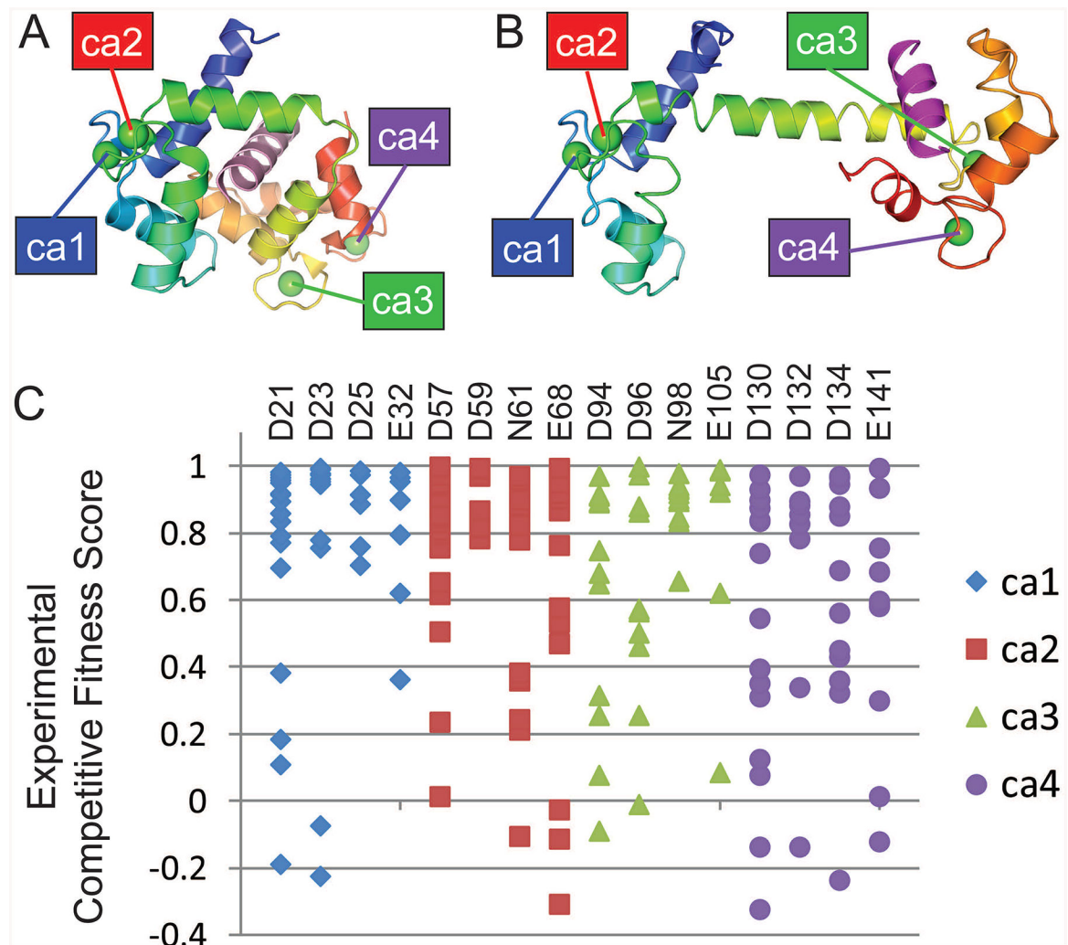
Figure 2. CALM1 Ca-binding Functional Residue Mutations Exhibit Redundancy. Calcium binding sites are labeled numerically (Ca1-Ca4) and colored according to primary sequence order. Calmodulin structures are colored in rainbow from the N-terminus (blue) to the C-terminus (red). (A) Compact calmodulin structure conformation depicts Ca-dependent binding to the hydrophobic IQ Domain (pink cartoon, peptide2 mode) of the Cardiac Ca(v)1.2 Calcium Channel [PDB:2f3y]. (B) Extended calmodulin structure conformation depicts Ca-dependent binding to the inactivation gate DIII-IV linker (magenta cartoon, peptide1 mode) of the cardiac sodium channel (Na(V)1.5) [PDB: 4djc]. (C) Experimental competitive fitness scores (unscaled) for Ca-binding site mutations diverge from wildtype (green section) through intermediate (yellow section) to detrimental (red section).
