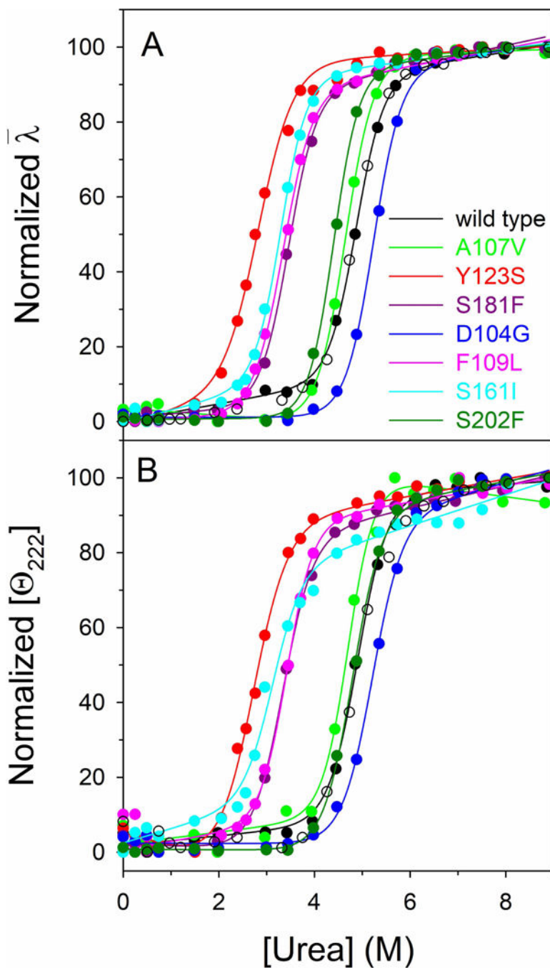
Figure 3. Urea-induced equilibrium unfolding of FXN wild type and variants. (A) Normalized intensity-averaged emission wavelength ( \bar{\lambda} ). (B) Normalized molar ellipticity at 222 nm ( [\Theta_{222}] ) reported after removal of the high-frequency noise and the low-frequency random error by SVD. The continuous lines represent the nonlinear fitting of the normalized ( \bar{\lambda} ) and [\Theta_{222}] data to Eq (3). The reversibility points (empty circles) are shown, for clarity, only for the wild type and were not included in the nonlinear regression analysis. All spectra were recorded at 20 °C, as described in Materials and Methods.
