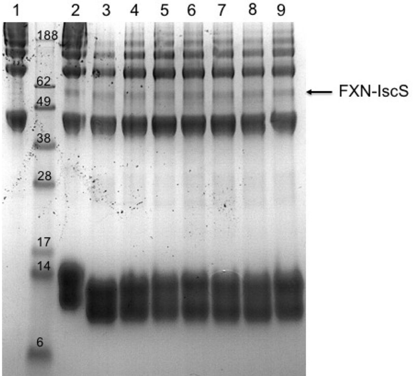
Figure 5. Cross-linking.
