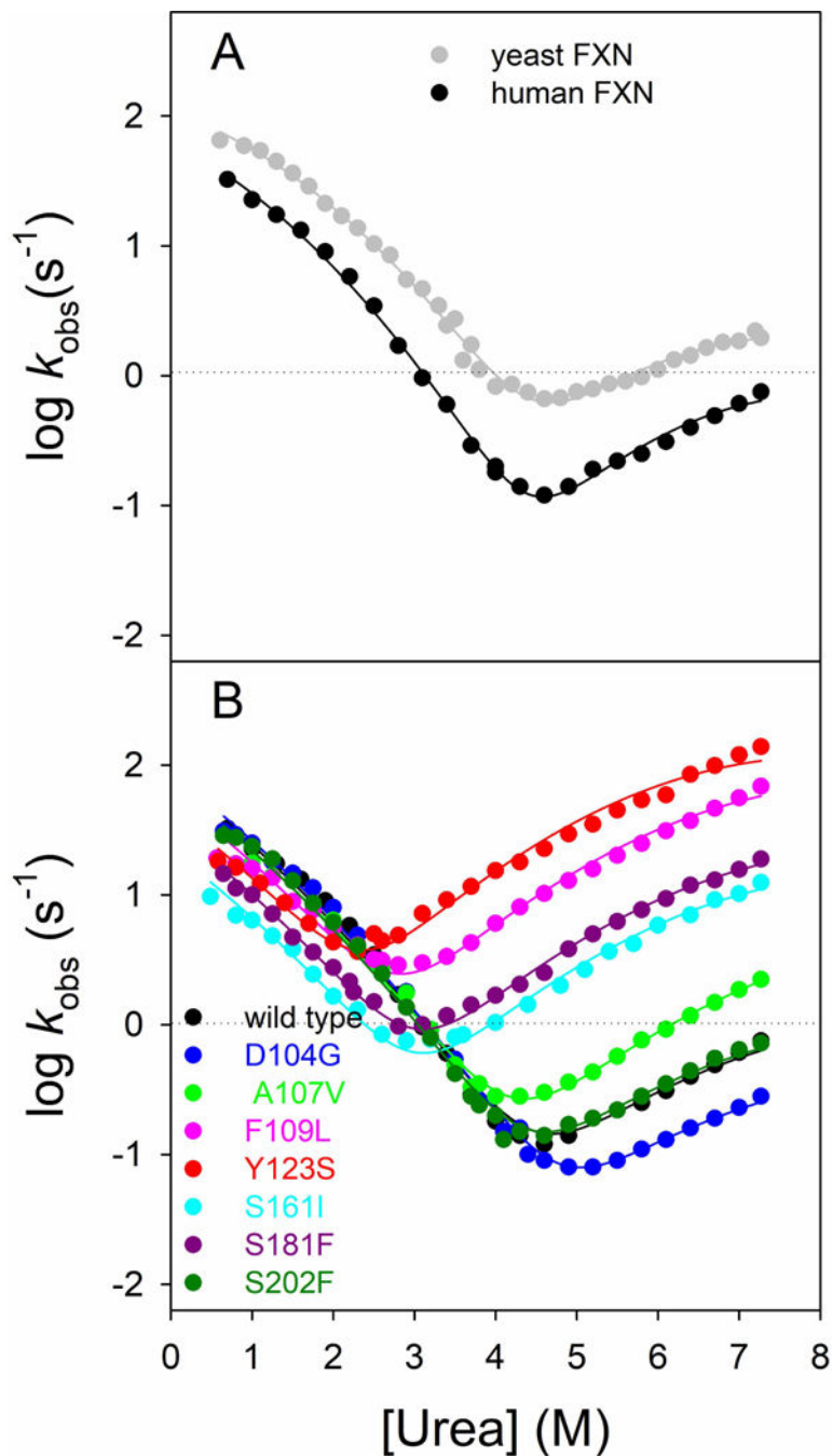
Figure 4. Chevron plots.
