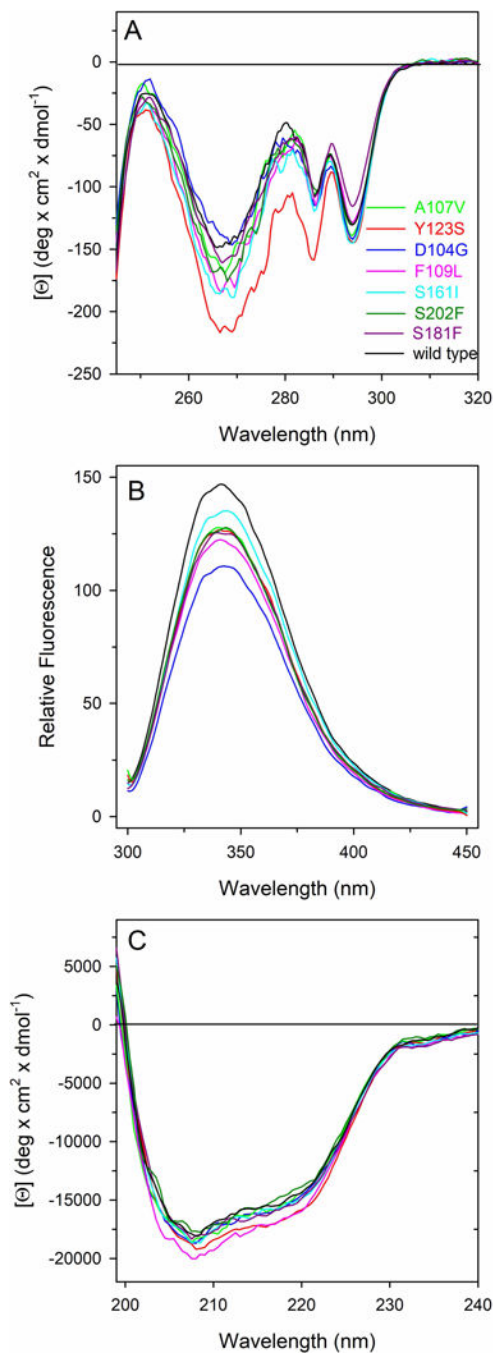
Figure 2. Spectral properties of FXN wild type and variants.
