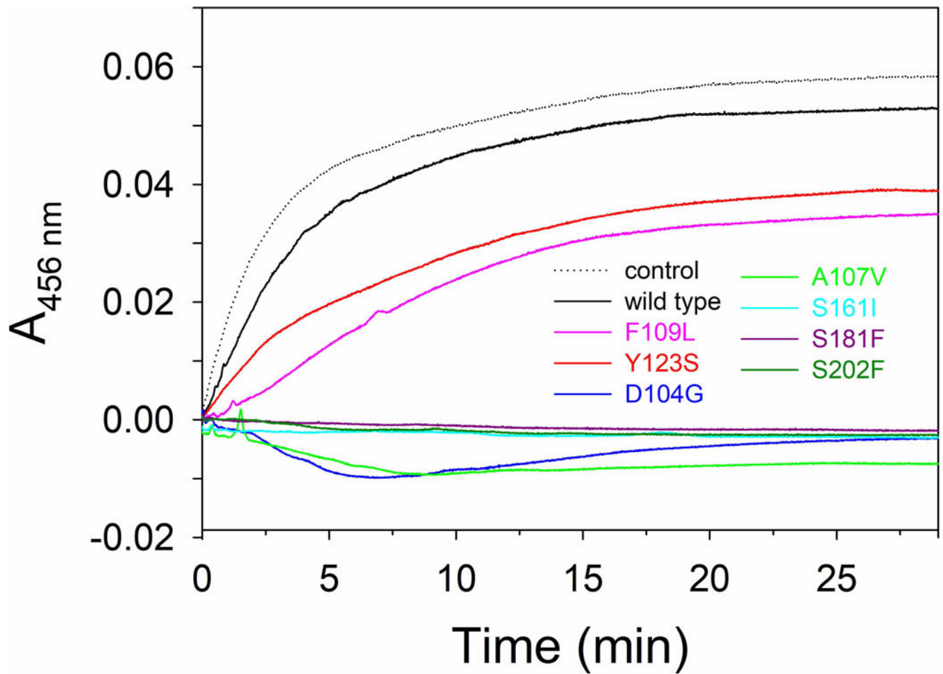
Figure 6. Cluster formation.
