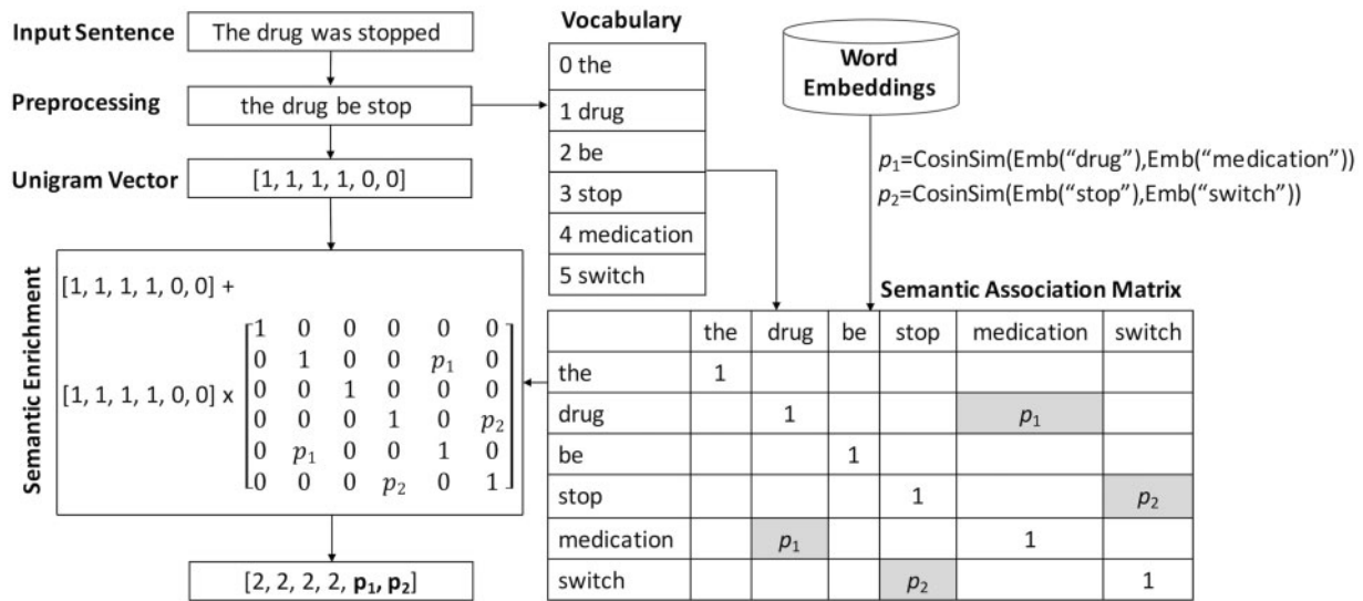
Figure 2. Illustrative example for semantic enrichment via word embeddings.
