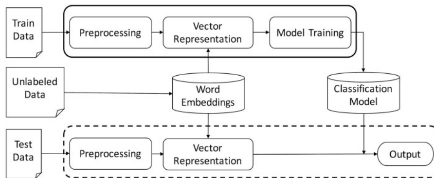
Figure 1. System Workflow. The classification model trained on the training data is applied on unseen test data.
