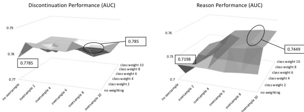
Figure 3. Performance trend on combined oversampling and cost-sensitive training.
