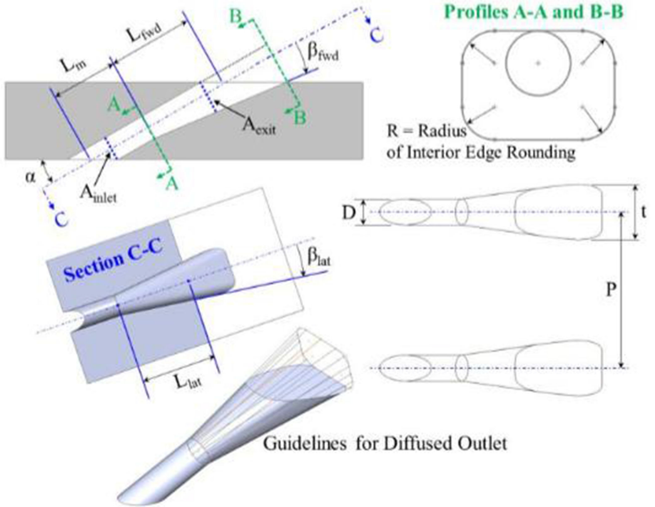
FIGURE 8. GEOMETRY OF 777 HOLE [14]
