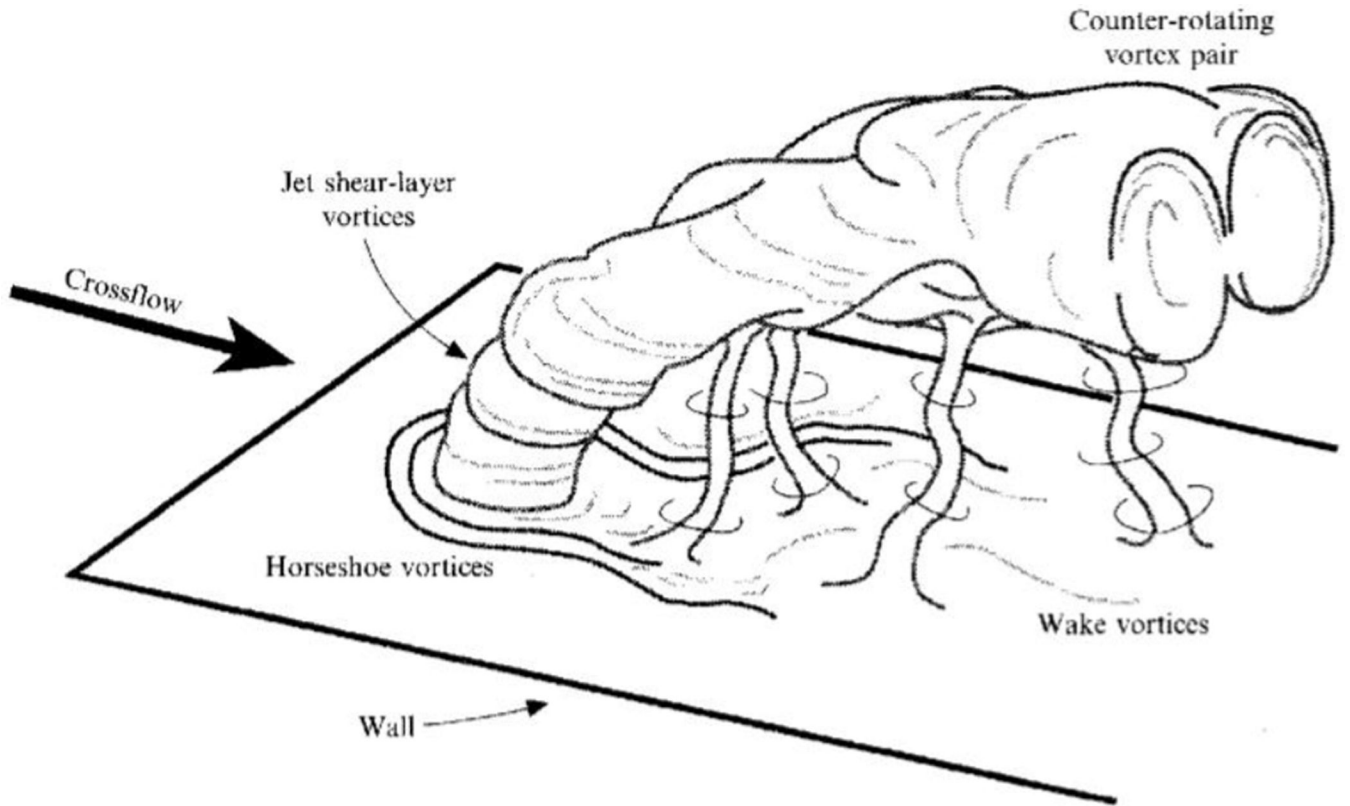
FIGURE 1. VORTICAL STRUCTURES FOR JET-IN-CROSSFLOW [5]
