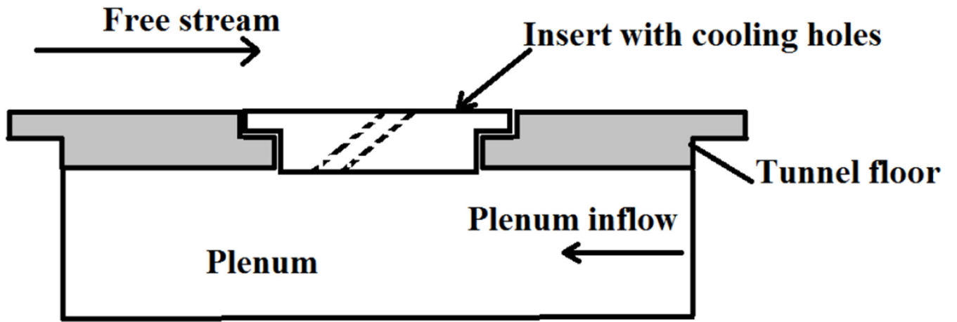
FIGURE 5. TEST SECTION FLOOR SHOWING INSERT FOR COOLING HOLE
