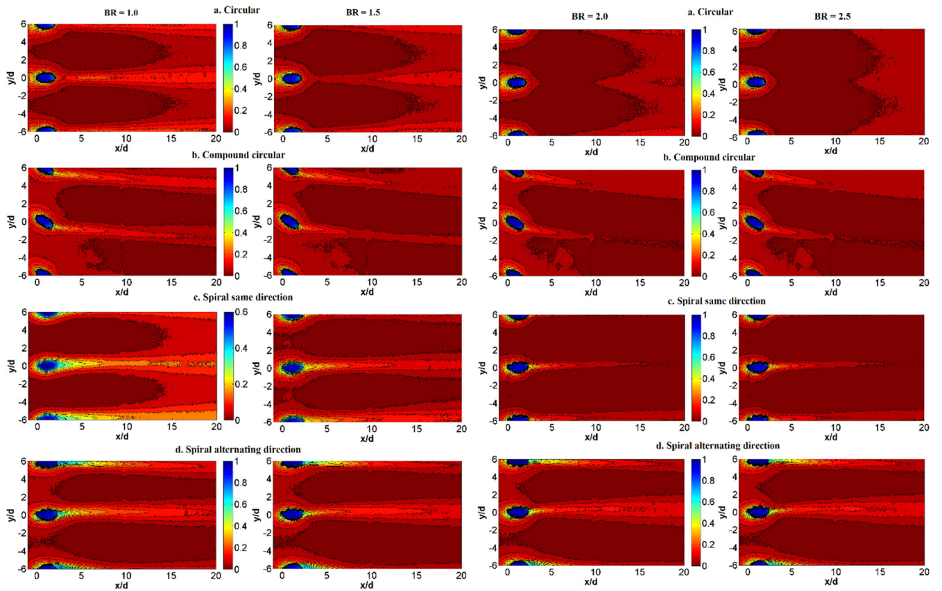
FIGURE 20. ADIABATIC FILM EFFECTIVENESS BASED ON IR SURFACE TEMPERATURE MEASUREMENTS FOR CYLINDRICAL-TYPE HOLES AT P/D=6.0 , L/D=4.0 , Re = 11,000 . LEFT TO RIGHT: BR=1.0, 1.5, 2.0, 2.5
