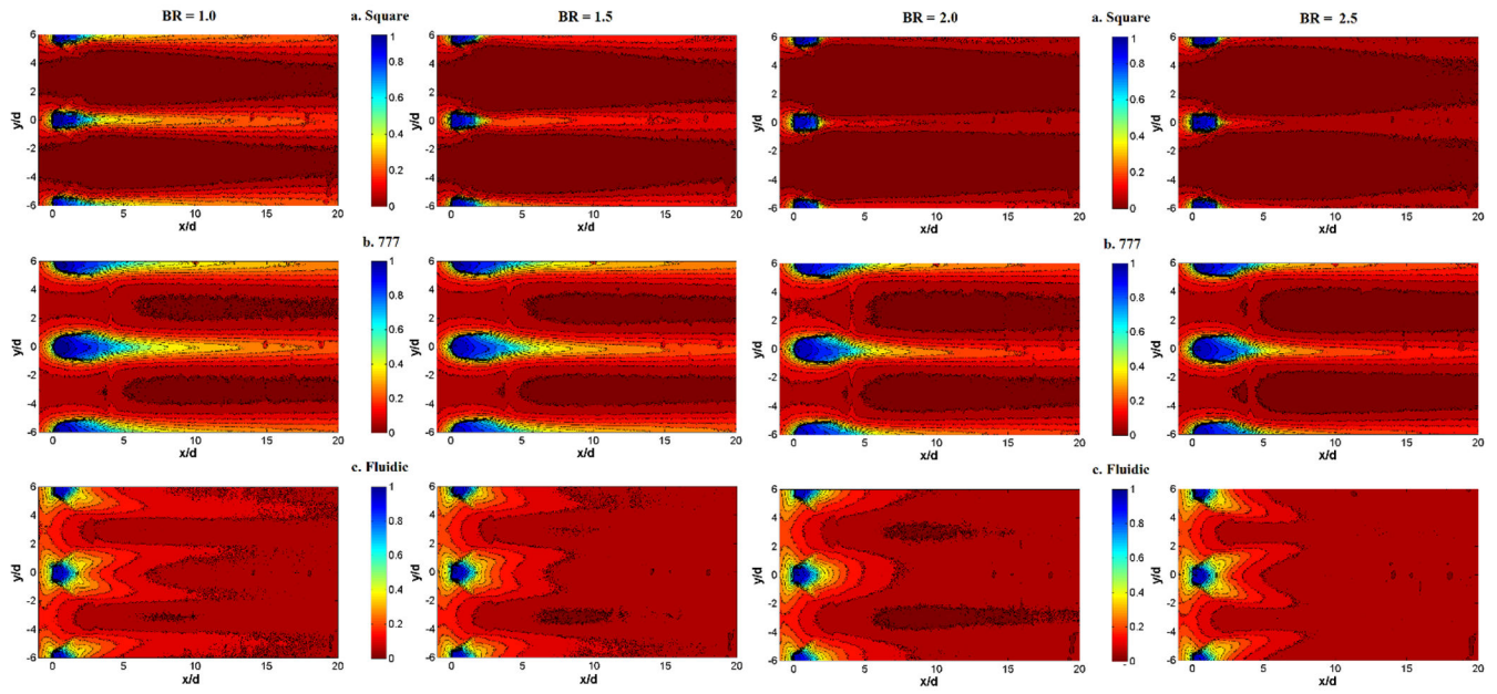
FIGURE 15. ADIABATIC FILM EFFECTIVENESS BASED ON IR SURFACE TEMPERATURE MEASUREMENTS FOR SQUARE, 777 AND FLUIDIC HOLE AT DR=1.05 . LEFT TO RIGHT: BR=1.0, 1.5, 2.0, 2.5
