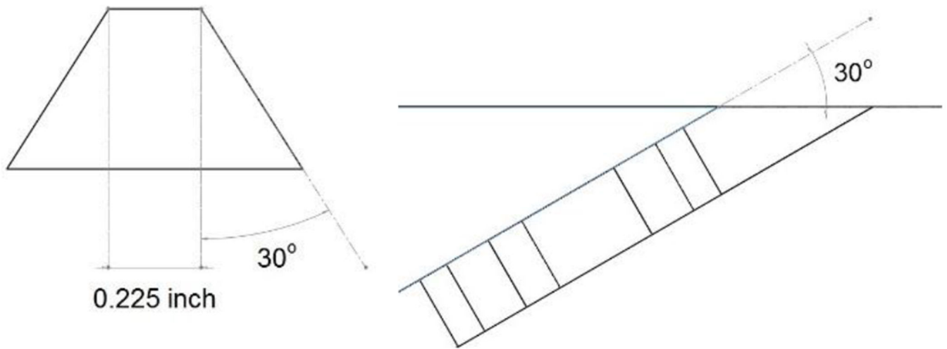
FIGURE 7. GEOMETRY OF FLUIDIC AND SQUARE HOLES
