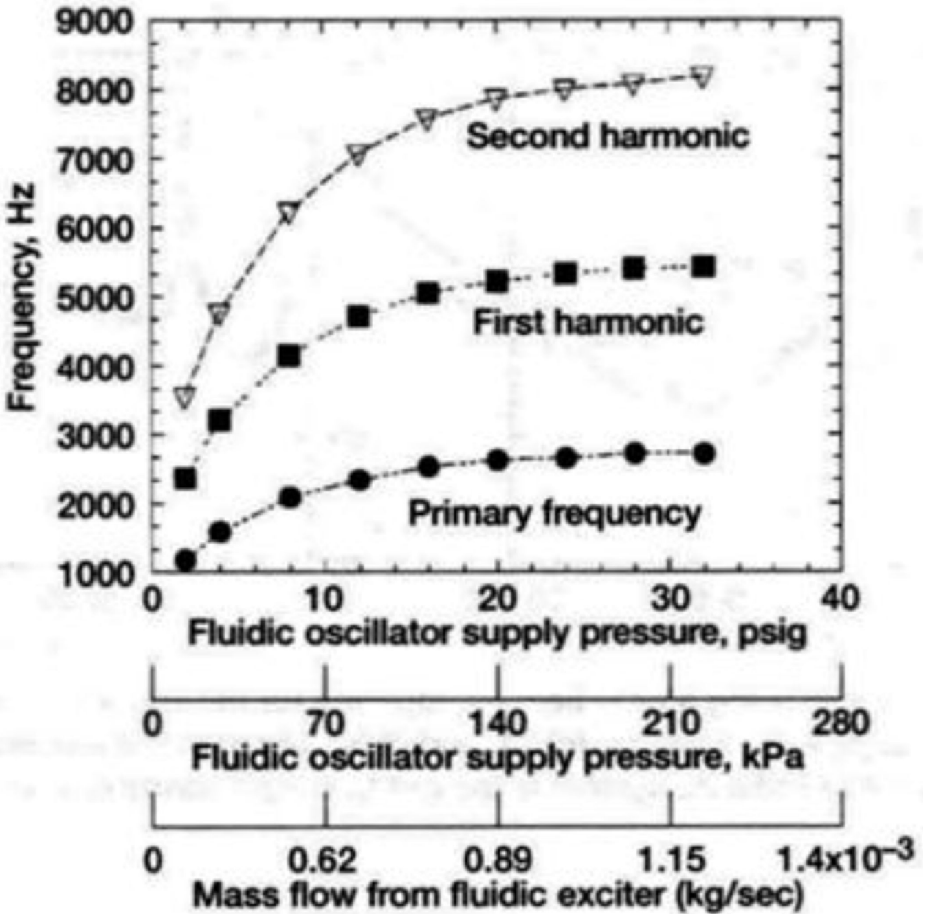
FIGURE 3. FREQUENCY AND MASS FLOW CHARACTERISTICS OF A SWEEPING JET [12, 13]
