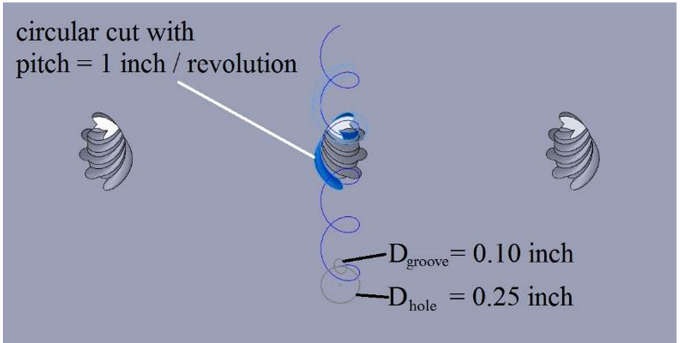
FIGURE 9. GEOMETRY OF SPIRAL HOLES
