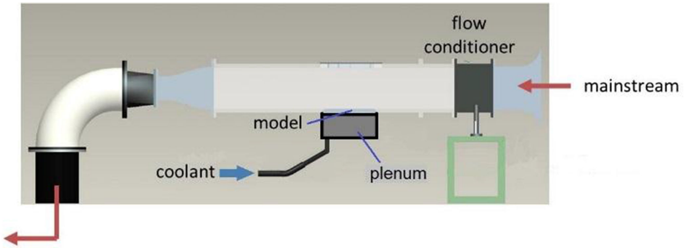
FIGURE 4. TEST FACILITY
