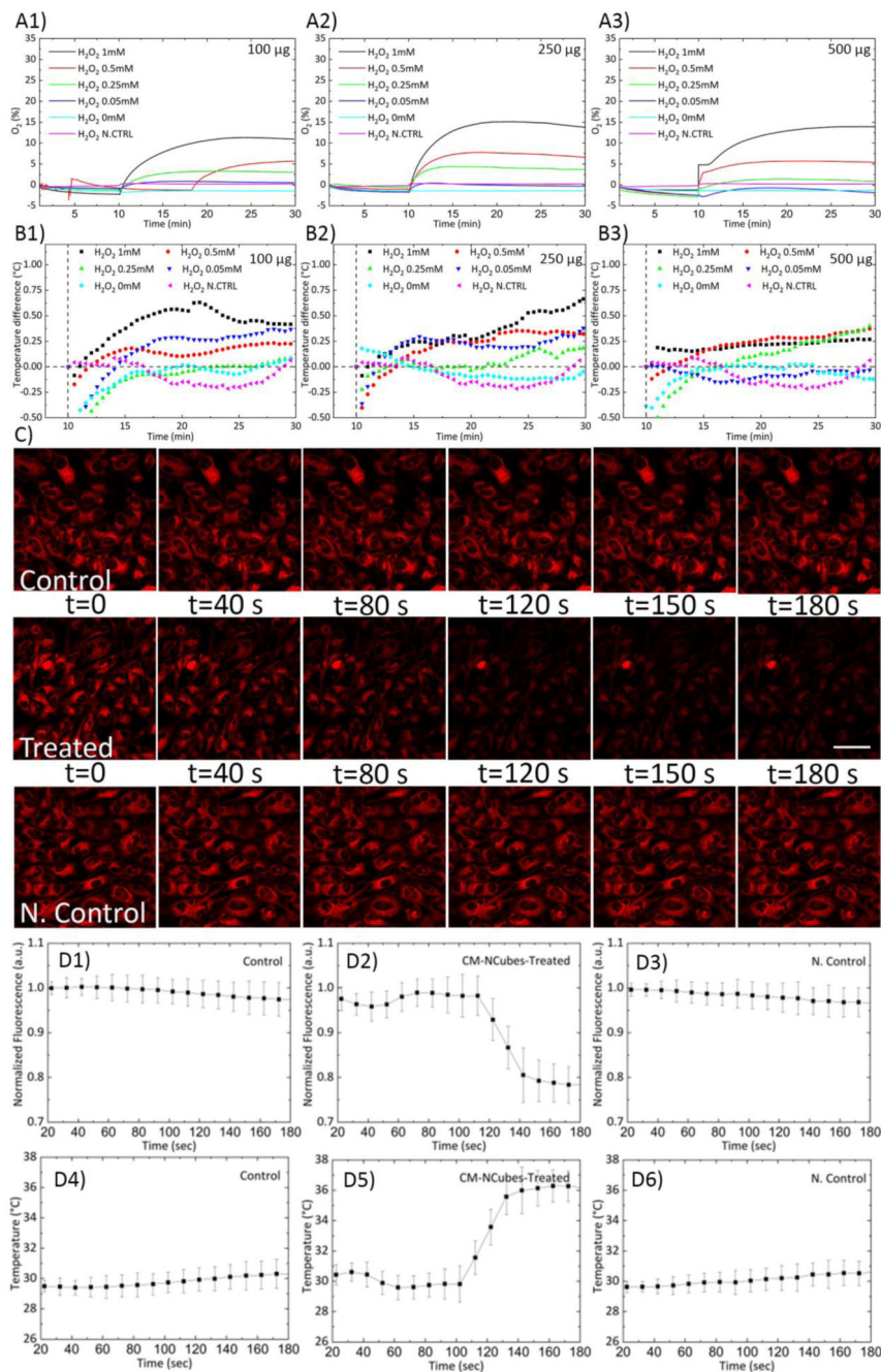
Figure 4. A) Oxygen generation and B) temperature increment after the reaction of different concentrations of CM-NCubes (100, 250 and 500 μg ml -1 ) with increasing concentrations of H 2 O 2 (0, 0.05, 0.25, 0.5 and 1 mM). H 2 O 2 1 mM reacting with plain medium (H 2 O 2 N. Control) was used as a negative control both in the oxygen generation and in the temperature measurements; C) confocal images showing the difference of fluorescence intensity in U-251 MG cells incubated with 250 μg ml -1 of CM-NCubes overnight after the addition of plain DMEM supplemented with 25 mM HEPES (control), and after the addition of 100 μM
