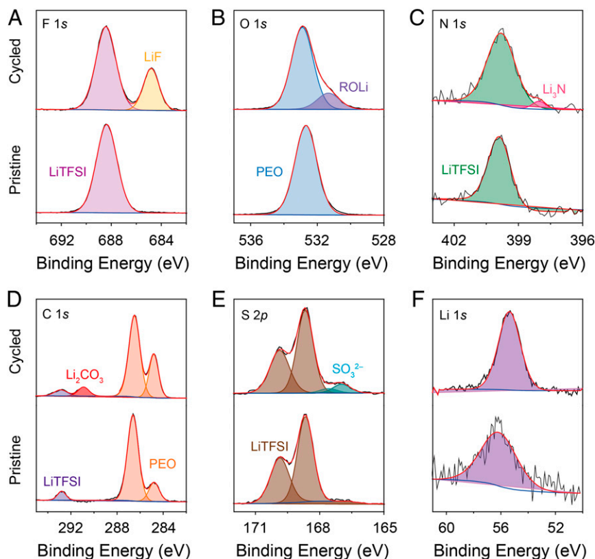
Fig. 4. XPS spectra of the pristine and cycled PEO/LSTZ membrane: (A) F 1s, (B) O 1s, (C) N 1s, (D) C 1s, (E) S 2p, and (F) Li 1s; spectra of the pristine PEO/LSTZ are below the cycled.
