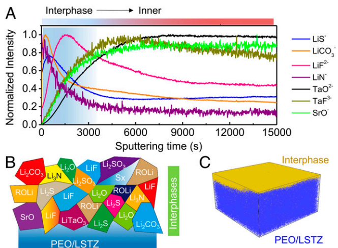
Fig. 5. (A) Normalized TOF-SIMS depth profiles of fragments of interest collected from a cycled PEO/LSTZ membrane. (B) Schematic illustration showing the chemical species of interest formed on the surface of the cycled PEO/LSTZ. (C) Corresponding 3D distribution of the interphase on the cycled PEO/LSTZ membrane.
