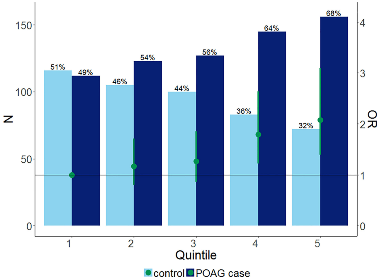
Fig. 1. Genetic Risk Score. Genetic risk score based on the 15 known POAG-loci identified in Europeans and Asians GWAS (rs1192415, rs28504591, rs4619890, rs2745572, rs11969985, rs4236601, rs284489, rs10712703, rs2472493, rs58073046, rs7137828, rs10483727, rs3785176, rs9897123, rs16984299). Participants were grouped into quintiles of the genetic risk scores. Green circles represent the POAG odds ratio (adjusted for age, sex and principal components) when comparing each quintile to the lowest quintile (Q1 = reference line). The green-capped lines represent 95% CI of the POAG odds ratios. Bars represent the percentage of POAG cases (dark blue) and controls (light blue) per quintile.
