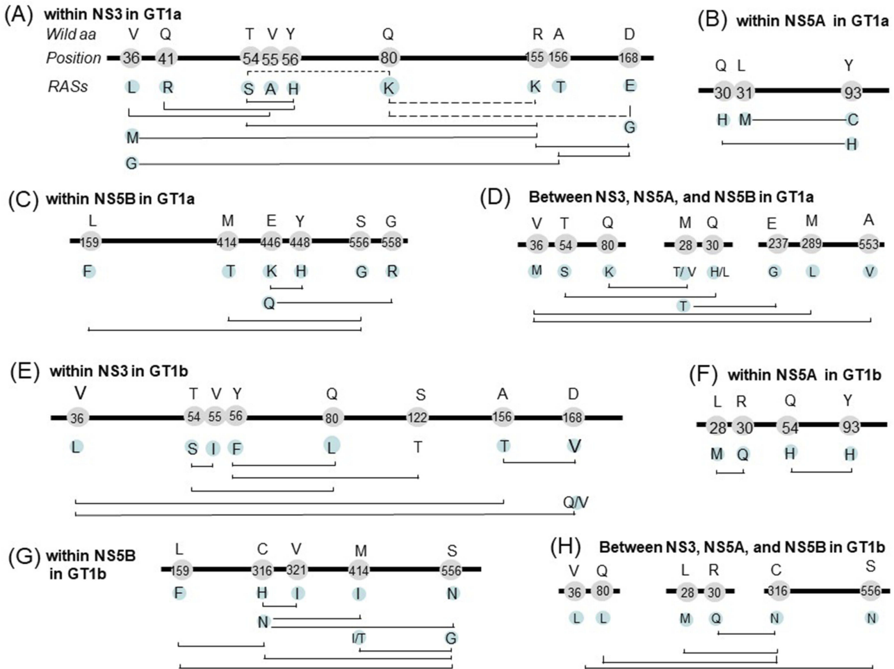
Figure 4 Co-occurring and mutually exclusive RAS pairs within NS3 (A), NS5A (B) and NS5B (C) and among regions (D) in GT1a; within NS3 (E), NS5A (F) and NS5B (G) and among regions (H) in GT-1b. Bold line represents HCV genome, the figures on the line indicate the location of amino acid, the characters above the location indicate the wild type amino acids, and the characters below the location indicate RASs. The solid, and dashed line connecting two RASs indicate co-occurring RAS pairs (significantly more frequent appearance than expected) and mutually exclusive RAS pairs (significantly infrequent occurrence than expected), respectively. Amino acid residue position is numbered relative to the first amino acid of the NS3, NS5A, or NS5B region.
