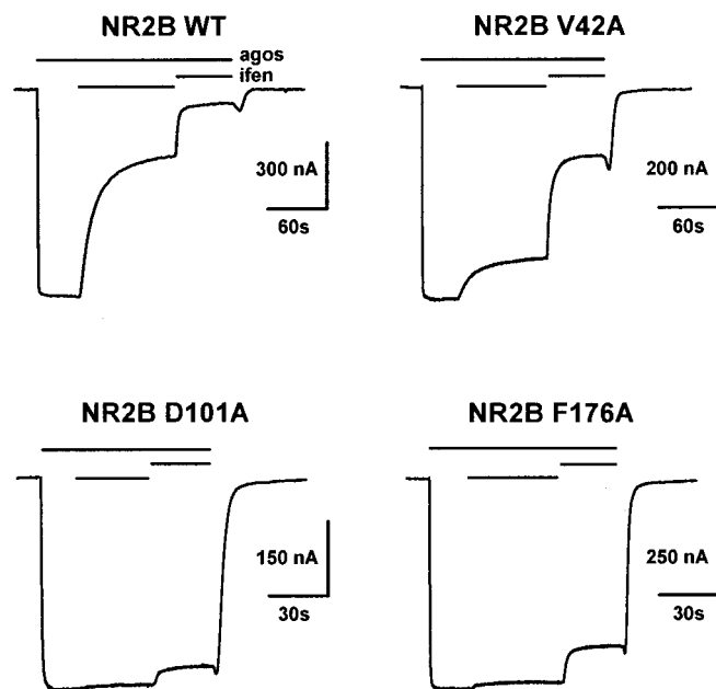
Figure 5. Identification in the LIVBP-like domain of NR2B critical residues controlling high-affinity ifenprodil inhibition. A comparison of the current traces obtained from oocytes coexpressing NR1 with either wt or mutated NR2B subunits is shown. Ifenprodil was applied at two increasing concentrations (300 nM and 3 \mu M) during an application of agonists. The bars above the current traces indicate the duration of agonists ( agos ) and ifenprodil ( ifen ) applications. The holding potential was -60 mV. These current traces are typical of NR2B mutants having an intermediate ( V42A ) or strong ( D101A , F176A ) effect on ifenprodil sensitivity.
