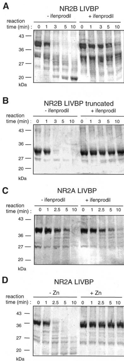
Figure 3. Ifenprodil protects the isolated LIVBP-like domain of NR2B but not that of NR2A against hydrolysis by trypsin. Isolated LIVBP-like domains of NR2A and NR2B were produced in E. coli and subjected to trypsinization with or without ifenprodil or Zn for various amounts of time (up to 10 min). Fifty micrograms of the purified LIVBP-like domains were mixed with 0.1 \mu g of trypsin. The samples were analyzed on 12% SDS-PAGE gels. Lane 0 corresponds to the protein solution just before trypsin addition. A , Ifenprodil (10 \mu M) protects the NR2B LIVBP-like domain (main band at ~40 kDa) against trypsin digestion. B , Ifenprodil (10 \mu M) also protects a C-terminal truncated NR2B LIVBP-like domain (main band at ~30 kDa) against trypsin digestion. C , Ifenprodil (100 \mu M) does not protect the NR2A LIVBP-like domain (main band at ~40 kDa) against trypsin digestion. D , Zn (10 \mu M) protects the NR2A LIVBP-like domain against trypsin digestion.
