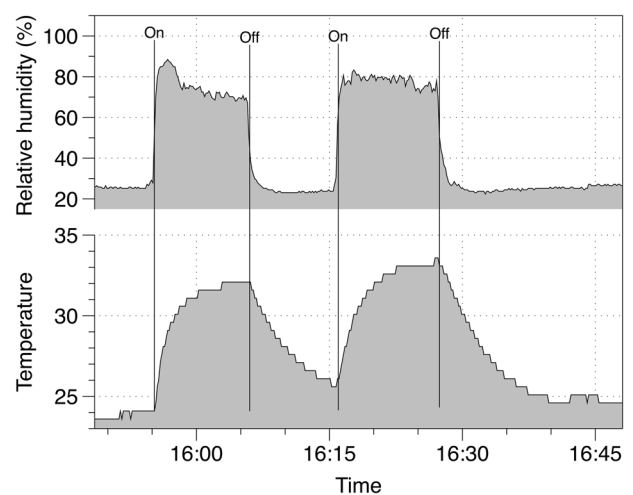
Fig. 1 Typical temperature and humidity profile from donning a respirator on two occasions—on/off times as recorded by the participant
