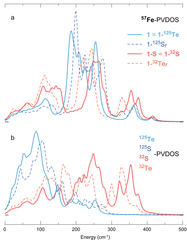
Fig. 6 DFT-simulated (a) ^{57}\text{Fe} - and (b) ^{125}/^{32}\text{Te}/\text{S} -PVDOS spectra from models 1 (=1\text{-}^{125}\text{Te}) and 1\text{-S} (=1\text{-}^{32}\text{S}) , as well as their fictitious ^{32}\text{Te} - and ^{125}\text{S} -isotopologues 1\text{-}^{32}\text{Te}_f and 1\text{-}^{125}\text{S}_f .
