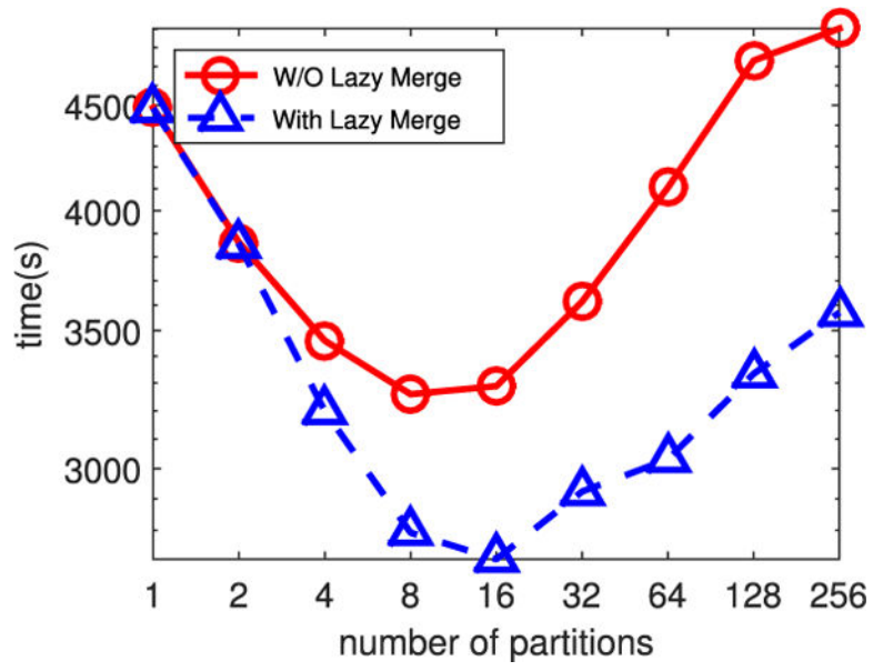
Fig. 10. Computation time with and without lazy merging.
