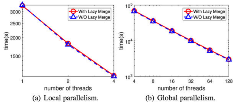
Fig. 11. Local parallelism and global parallelism.
