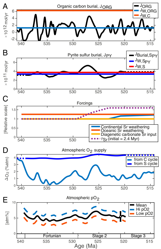
Fig. 5. Atmospheric \text{O}_2 levels in the Terreneuvian is simulated from (A) organic carbon burial (Eqs. 1 and 2) and (B) pyrite sulfur burial (Eqs. 11 and 12) using typical Cambrian parameter values (Dataset S3) obtained from seawater carbon and sulfur isotope curves and forced by a shift toward more continental weathering 524 to 523 Ma. (C) The weathering flux forcings applied to fit the Sr isotope data in Fig. 3 is shown together with the expected oceanic Sr residence time. (D) \text{O}_2 release to the atmosphere from organic C burial (light blue) and pyrite S burial (blue) are the principal sources of atmospheric \text{O}_2 . In combination with global \text{O}_2 removal through oxidative weathering (blue curves in A and B), we estimate atmospheric \text{pO}_2 change. (E) The absolute atmospheric \text{pO}_2 curve (black) is fit to a model-dependent constraint at 521 Ma 4 to 7 atm% (black, dashed curves). A shift from preferential aragonite to calcite precipitation in the ocean \sim 525 Ma (here shown a few million years too early to distinguish the effect from enhanced weathering) would have changed the Sr residence time (33), but has no effect on the atmospheric \text{pO}_2 curve. Note that enhanced weathering both affects atmospheric \text{O}_2 supply through sediment burial and atmospheric \text{O}_2 removal through oxidative weathering, and therefore has little effect on atmospheric \text{pO}_2 in this model.
