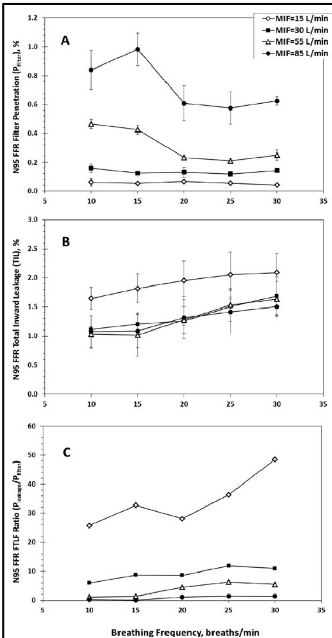
FIGURE 1. Filter penetration (A), Total Inward Leakage (TIL) (B), and faceseal leakage-to-filter (FLTF) ratio (C) for a N95 FFR sealed to a plastic manikin's face. Each data point in plot C represents the FLTF ratio calculated as the mean P_{leakage} (determined from three replicates) divided by the mean P_{filter} (also determined from three replicates). Consequently, no error bars are presented in plot C.
