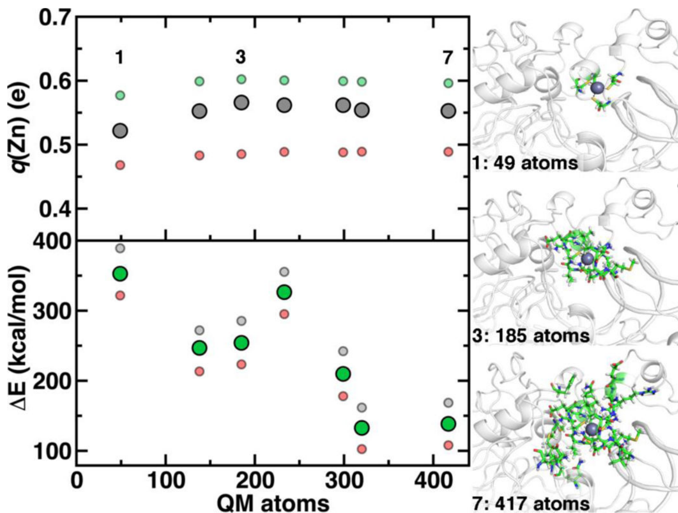
Figure 11. Dependence of properties with QM region size: Zn Mulliken partial charge ( q(\text{Zn}) , in e ) shown at top left and rigid binding energy ( \Delta E , in kcal/mol) shown at bottom left. For each property, three snapshots are computed (40 ns in gray, 60 ns in red, and 100 ns in green), and the middle range symbol is shown in large solid symbols, whereas the upper and lower quantities are shown as translucent, smaller symbols. QM regions 1 , 3 , and 7 are shown at right in ball and stick representation.
