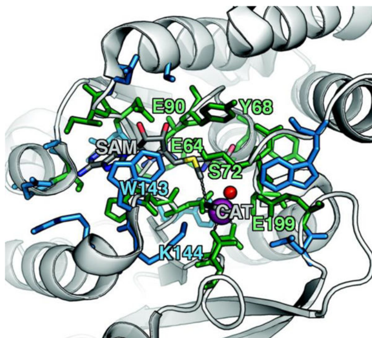
Figure 1. COMT structure with SAM and catechol (CAT) substrates shown in gray along with Mg^{2+} as a magenta sphere and a water coordinating the Mg^{2+} as a red sphere. The 28 protein residues (518 atoms with H atoms) included in a large QM region, as described in the main text, are shown as sticks. A subset that was identified by systematic analysis of QM regions is shown in green, whereas the remainder is shown in blue. Specific residues of interest are labeled by their single letter residue code and number.
