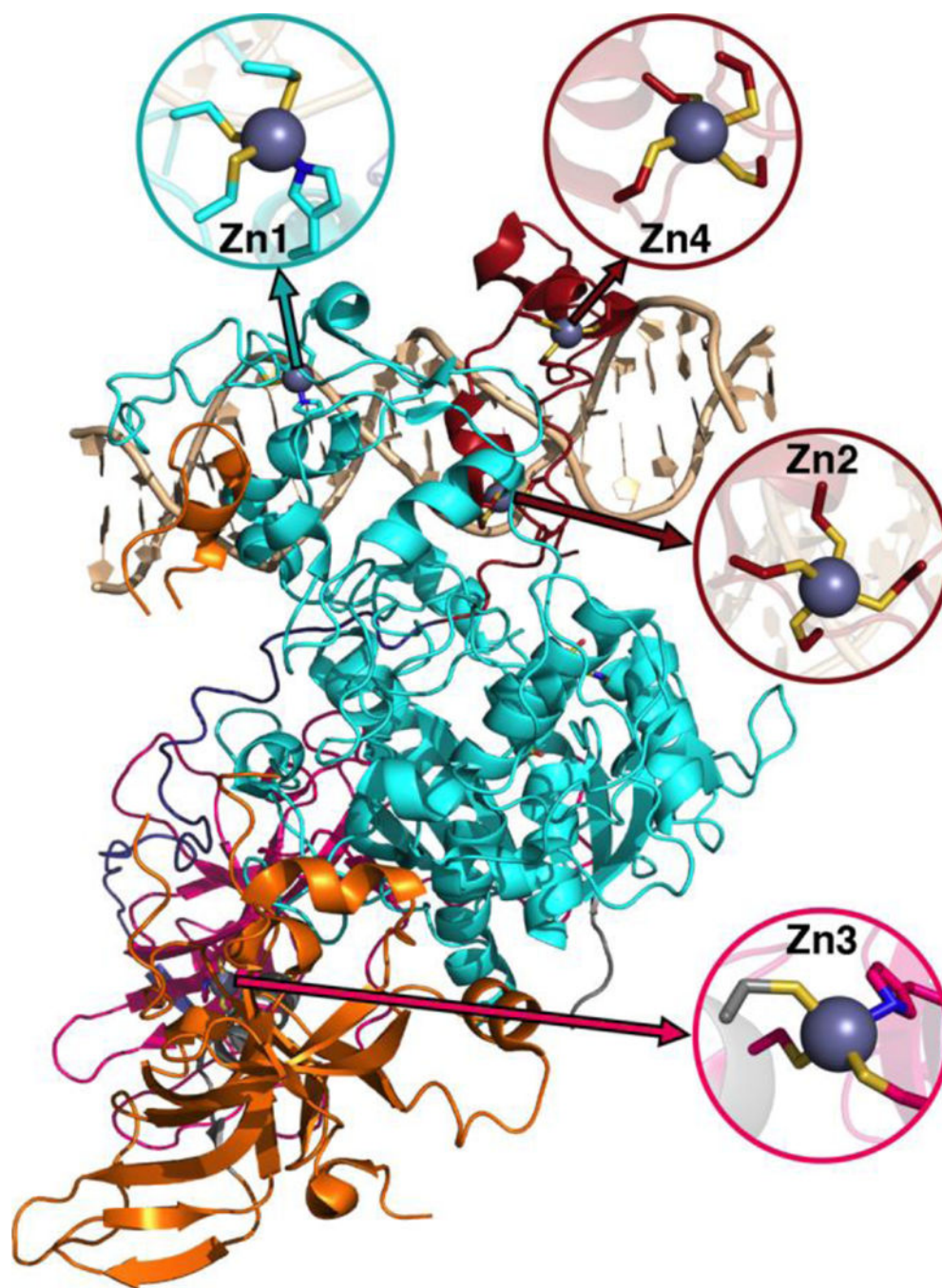
Figure 10. Structure of DNMT1 with DNA bound and separately colored protein chains. Each of the Zn sites in the crystal structure is shown in an inset with the relevant site on the protein indicated by arrows. Zn site numbering corresponds to the numbering in the experimental crystal structure. Zn is shown as a gray sphere, Cys S is shown in yellow, His N is shown in blue, and carbon atoms are colored according to the chain to which they belong.
