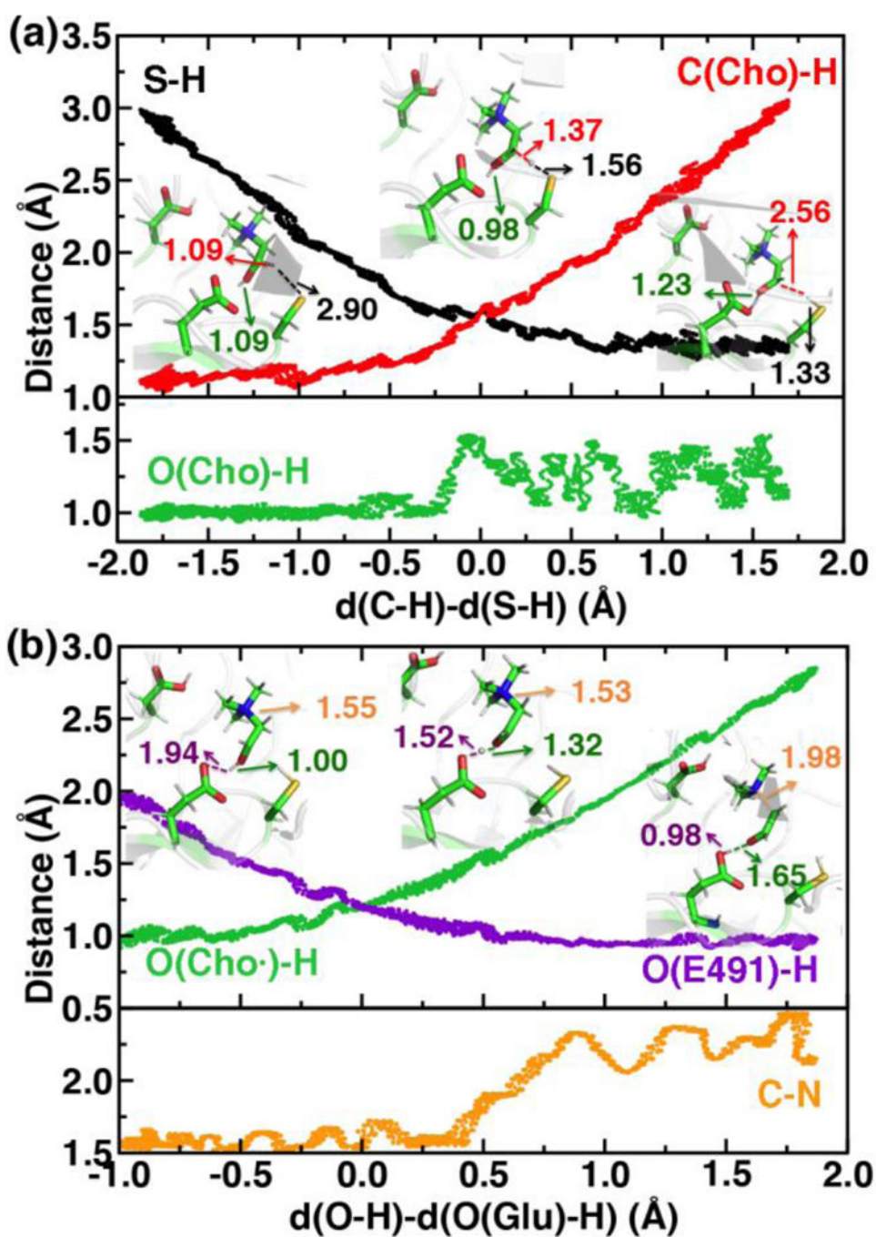
Figure 6. Distances along independent SMD trajectories defined by the LCODs described in the main text. (a) Choline C-H abstraction by cysteinyl radical S (C489) is shown, where the green line in the second pane indicates the choline hydroxyl O-H distance and black and red lines represent the S-H and the C-H distances, respectively. (b) Cholinyl radical deprotonation by E491 is shown, where the yellow line in the second pane represents the C-N distance, and purple and green lines represent O(E491)-H and O(Cho \cdot )-H distances, respectively. Select snapshots are shown in inset with the respective distances annotated.
