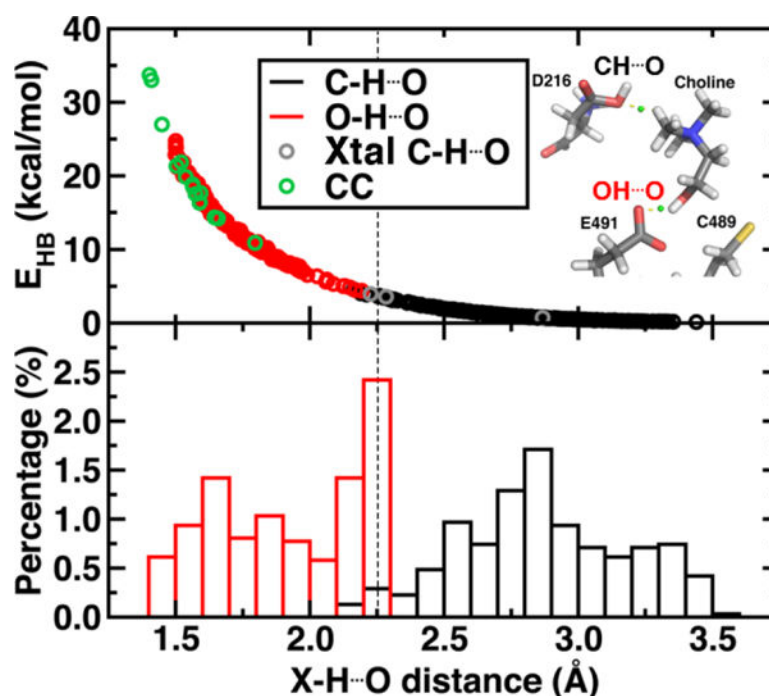
Figure 9. (top) Hydrogen bond energy ( E_{HB} , in kcal/mol) versus X-H...O distance for i) snapshot MD distances with X=O (red circles), X=C (black circles), ii) all observed close contacts in crystal structures (CC, green circles), and the X=C non-covalent interactions observed in CutC (Xtal C-H...O, gray circles). A snapshot showing the C-H...O and O-H...O hydrogen bond is provided in inset with the BCP shown as a green sphere. (bottom) Normalized distribution of CH...O and OH...O distances from MD snapshots as described for the top pane. A qualitative cutoff between CH...O and OH...O distances is indicated by a vertical dashed line at 2.25 Å.
