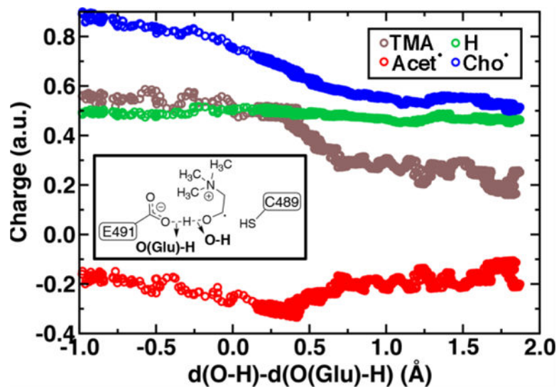
Figure 8. By-fragment-summed partial charges along the cholinyl radical deprotonation reaction coordinate: total cholinyl radical (Cho·, blue circles) and its substituent transferring H + (green circles), TMA (brown circles), and acetaldehyde radical (Acet·, red circles). A skeleton structure of the distances in the LCOD reaction coordinate is shown in inset.
