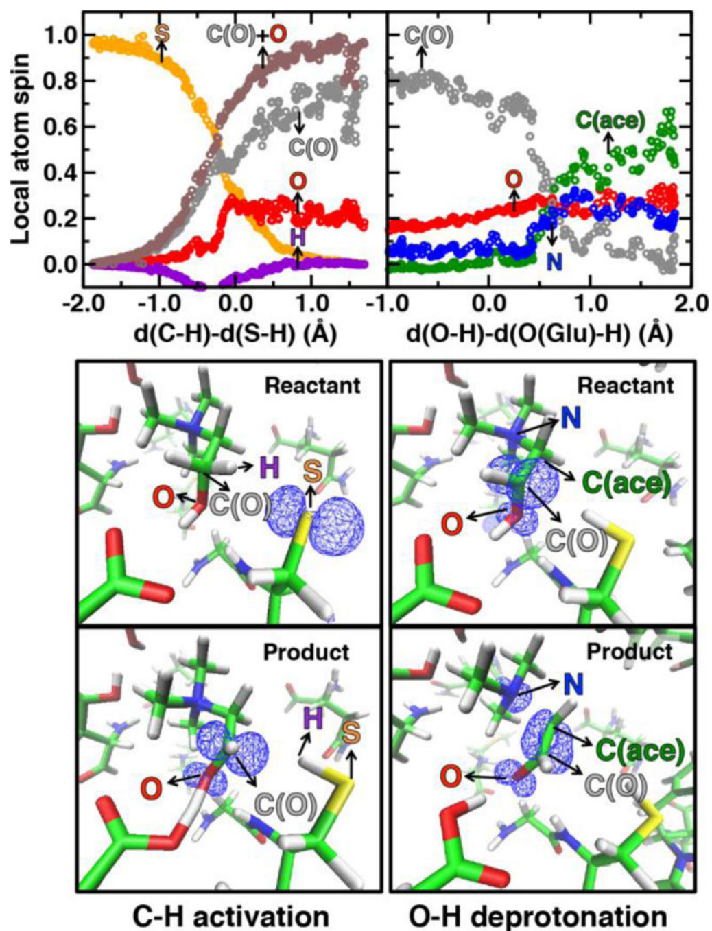
Figure 7. (top) Variation of local atom spin along the reaction coordinate of C-H abstraction (left pane) and of O-H deprotonation (right pane). The atom spin of S, O, N, and H are colored orange, red, blue, and purple, respectively. C(O) and C(ace) refers to the alpha- and beta-hydroxyl carbon atom, and are colored by grey and green, respectively. (bottom) Spin density distribution of typical reactant and product snapshots in H abstraction, and O-H deprotonation, respectively, where the spin density isosurface value is set to 0.01.
