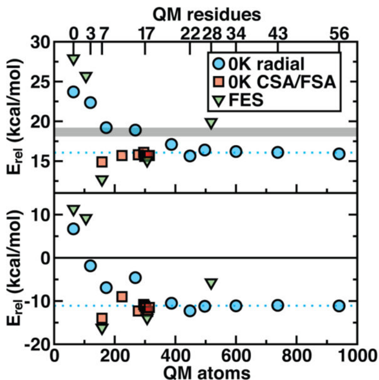
Figure 2. Barrier heights (top) and reaction energies (bottom) in kcal/mol for methyl transfer in COMT versus the number of atoms in the QM region obtained three ways: 0 K QM/MM properties from radially increasing distance cutoffs (blue circles, from Ref. 35), systematically constructed regions (red squares, from Ref. 62) and 300 K QM/MM free energy dynamics (green triangles, from Ref. 34). (top) G^\ddagger at 300 K or the 0 K E_a with the experimental G^\ddagger range 126–127 indicated as a gray shaded region that should only be compared to the green triangles. (bottom) G_{rxn} at 300 K or the 0 K E_{rxn} . In both plots, the asymptotic limit from the average of the three largest 0 K radial QM regions is shown as a blue dotted line and should only be compared to the blue circles and red squares. Approximate protein residue counts for each QM region size are labeled on the x-axis at top.
