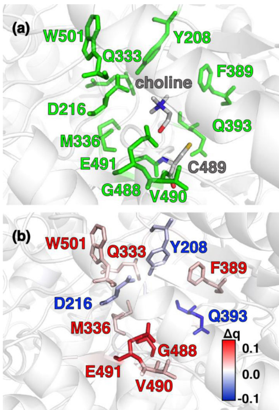
Figure 5. (a) CutC active site structure with choline substrate and cysteinyl radical (C489) shown in gray. Protein residues that were identified by charge shift analysis of QM regions are shown in green. (b) Difference of residue VDD charge upon substrate removal of the choline and residue mutation of C489 to alanine. Residues color-coded in blue and red correspond to loss and gain of partial charge upon substrate removal and residue mutation, respectively (as shown in inset color bar). All residues with |q| > 0.015 e are shown as sticks. Residues of interest are labeled by their single letter residue code and number.
