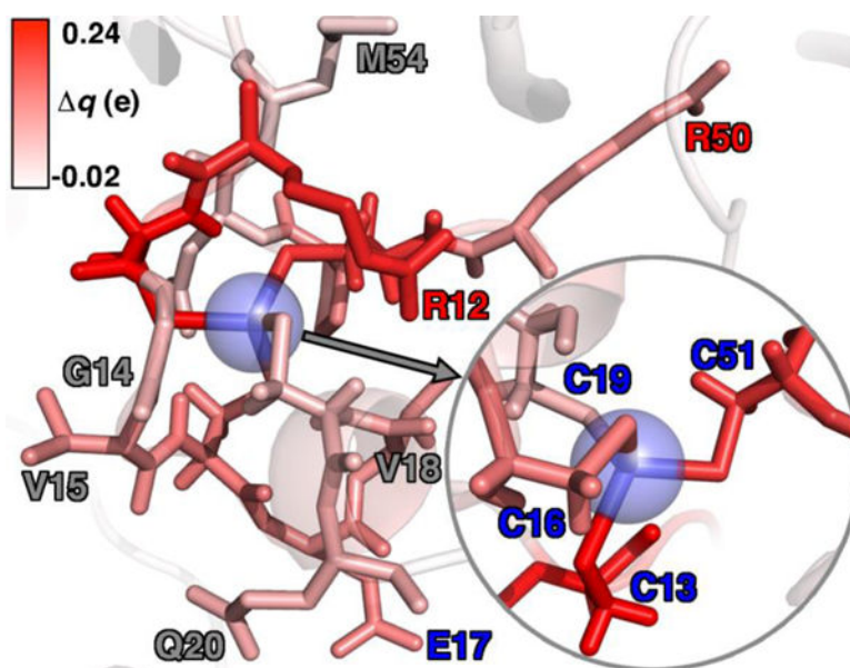
Figure 12. Difference of by-residue-summed Mulliken charges upon removal of \text{Zn}^{2+} in QM region 7 QM/MM simulations colored according to color bar in top left inset. All residues with |q| > 0.03 are shown as sticks, with key residues labeled by the single letter residue code and number colored for according to the formal charge (positive in red, neutral in gray, and negative in blue). Zn is not present in the simulation but its position is shown as a translucent blue sphere, and the coordinating Cys residues are shown in the inset at right.
